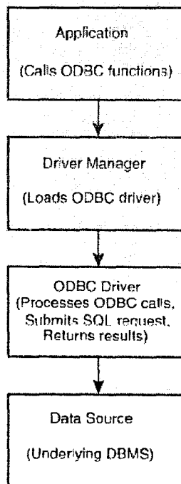
Figure 6.2 ODBC structure.
