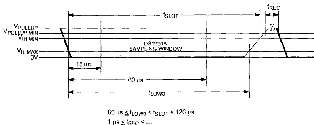
Figure 7.6.b Read / Write timing diagram, write-zero time slot.
