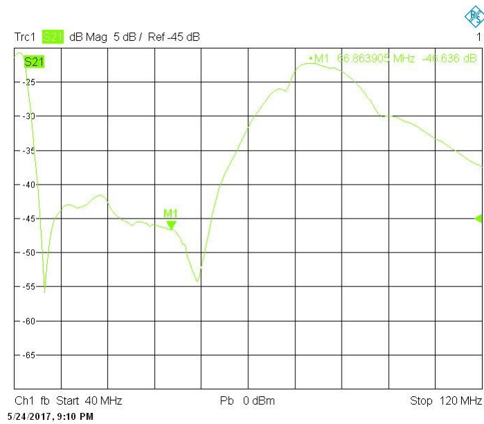
Figure 5.16 S_{21} results of the monopole antennas in the phantom with a conductive silver ink shielding in a cylindrical geometry (The Green marker shows that S_{21} is -46.6 dB at 66 MHz).
