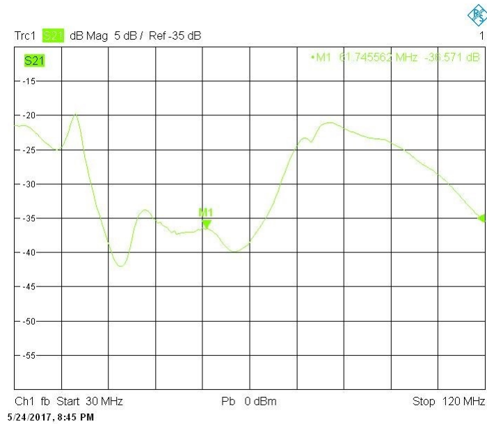
Figure 5.13 S_{21} results of the monopole antennas in the phantom with a conductive silver ink shielding planar geometry (The Green marker shows that S_{21} is -36.6 dB at 61 MHz).
