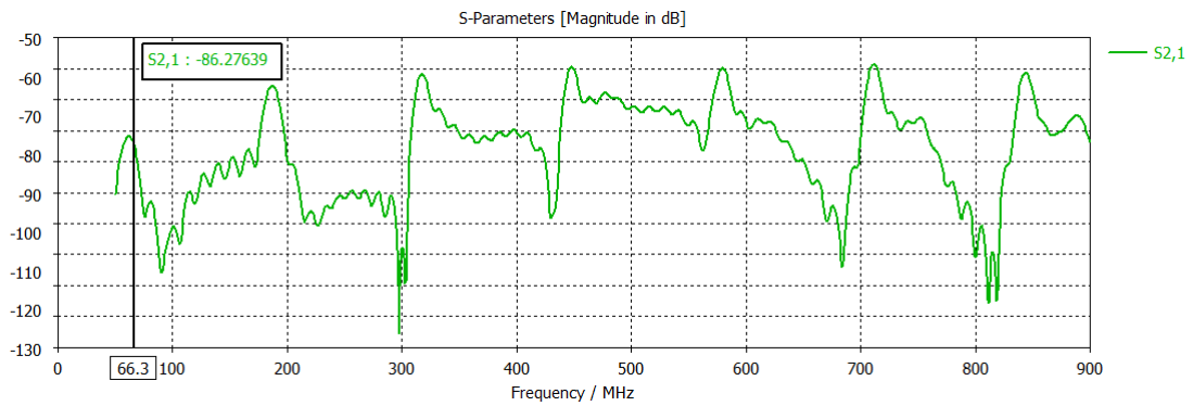
Figure 5.8 S_{21} parameter demonstrating the antenna behavior with cylindrical silver shielding material (The Black marker shows that S_{21} is -86.3 dB at 66 MHz).
