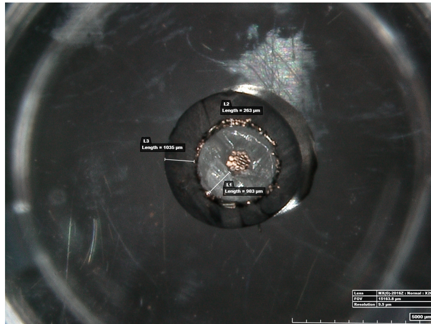
Figure 4.1 Microscopic (Hirox Microscope KH 8700) cross-section view of RG-58 coaxial cable(Lens MX(G)-2016Z: Normal: X20, FOV: 15163.8 \mu m , Resolution: 9.5 \mu m ).
