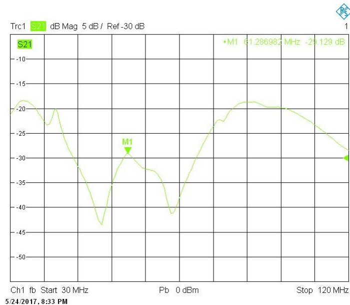
Figure 5.10 S_{21} results of the monopole antennas in the phantom (The Green marker shows that S_{21} is -29 dB at 61 MHz).
