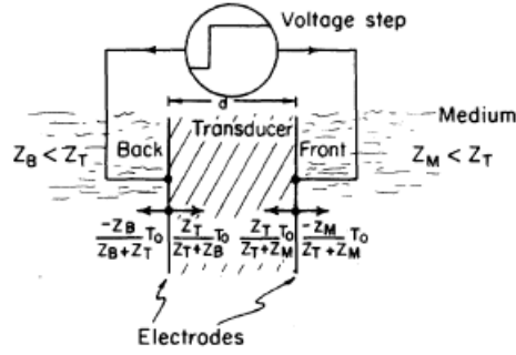
Figure 3.4 Schematic of pressure wave generation when applied voltage to a transducer [83].
