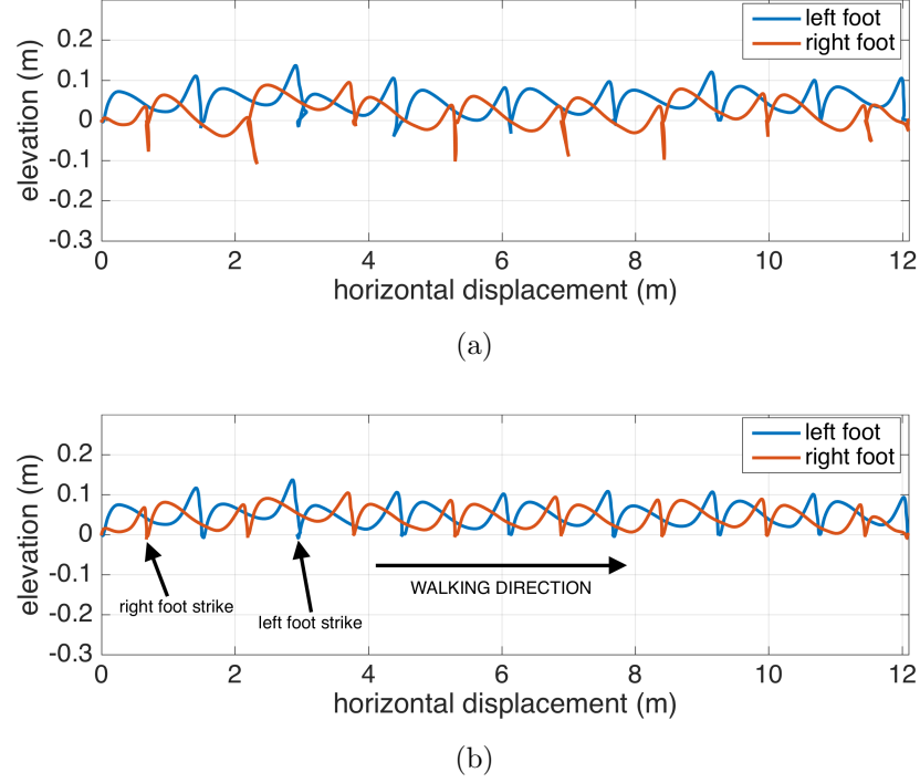
Figure 5.3. Lateral view of a walking subject, (a) Only Kalman filtering, (b) Kalman filtering with RTS smoothing.
