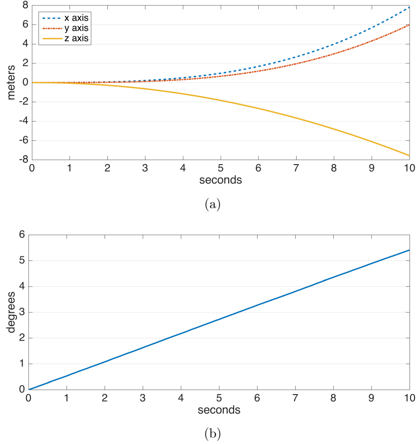
Figure 2.2. Typical drifts observed in integration of data from (a) accelerometer, (b) gyroscope.
