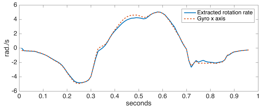
Figure 5.7. Extracted ankle axis rotation rate vs. x-axis gyroscope data of a correctly positioned sensor.
