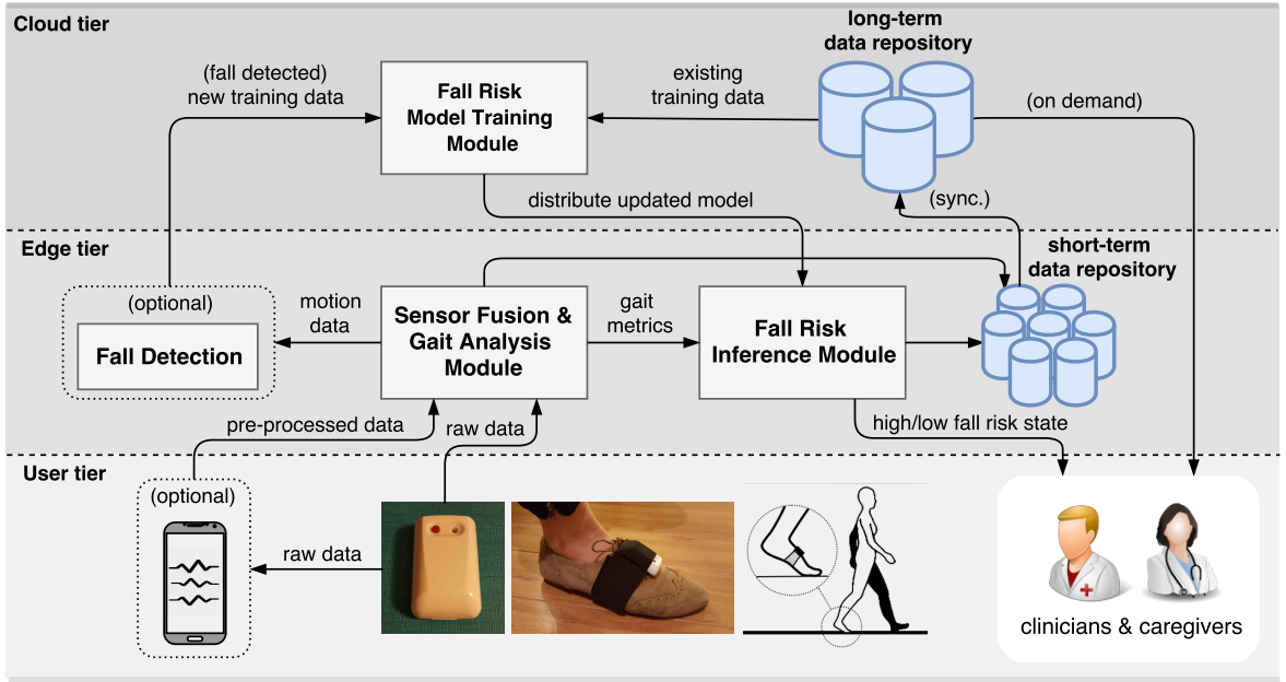
Figure 7.6. Multi-tier fall risk assessment service architecture.
