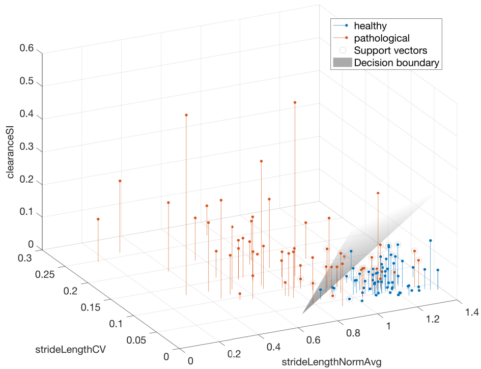
Figure 6.5. 3D visualization of selected parameters (SVM with linear kernel).
