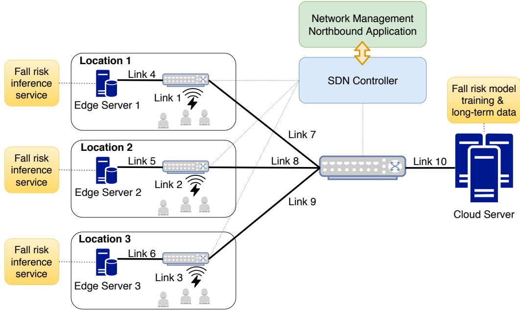
Figure 7.7. Emulation topology of multi-tier architecture.
