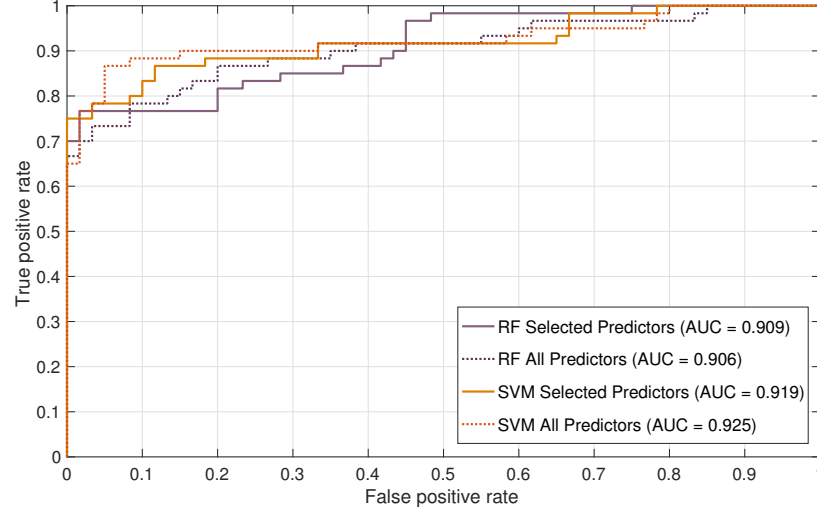
Figure 6.4. ROC curves for validating selected predictors.
