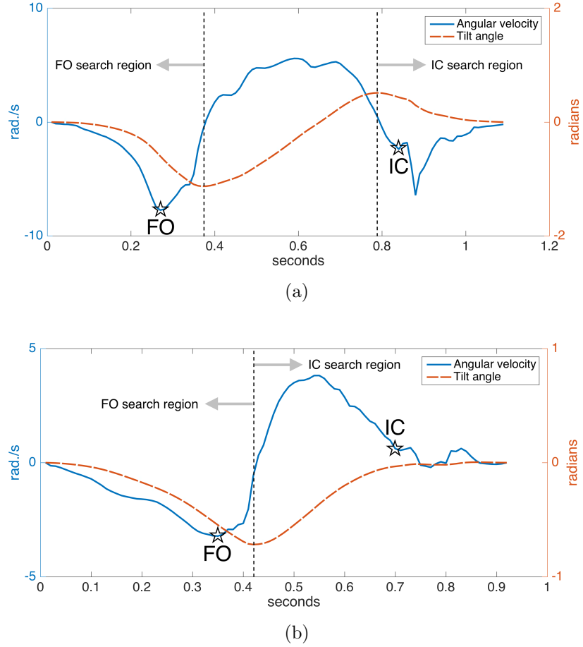
Figure 5.8. Detected FO & IC events, (a) healthy gait, (b) pathological gait.
