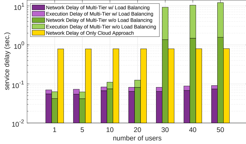
Figure 7.9. Contribution of network and execution conditions in overall delay.
