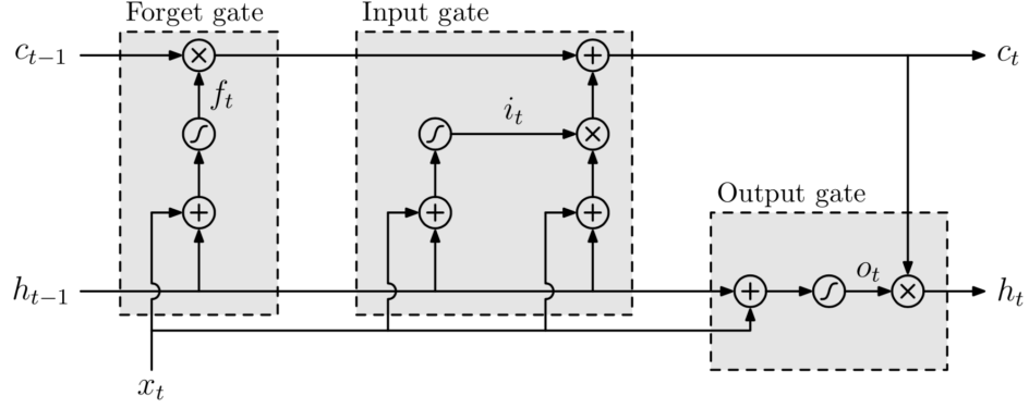
Figure 7.2. Schematic representation of an LSTM module [57].
