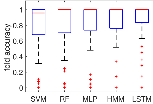
Figure 7.5. Box plots for fall risk classifier fold accuracies.
