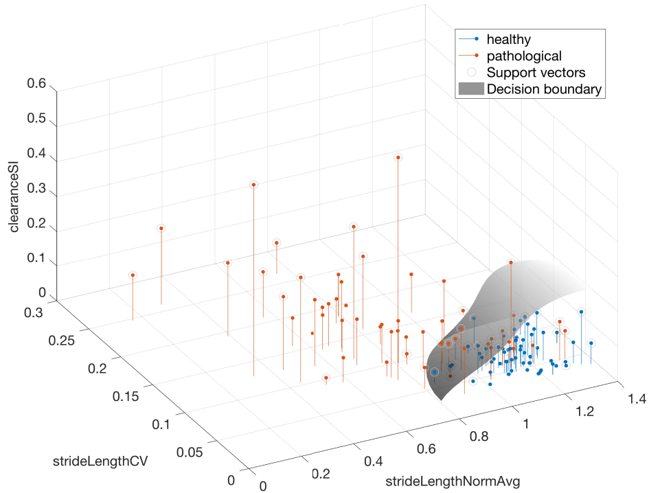
Figure 6.6. 3D visualization of selected parameters (SVM with RBF kernel).
