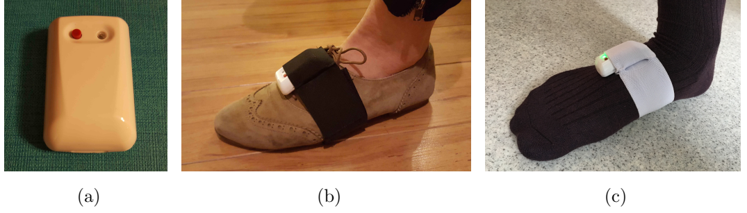
Figure 4.1. (a) ExLs3 IMU, (b) strapped to shoe, (c) strapped on socks.
