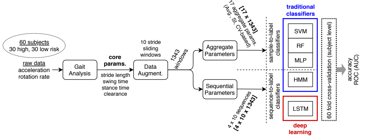
Figure 7.1. Data processing pipeline for fall risk assessment.
