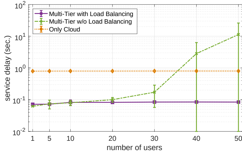
Figure 7.8. Performance comparison of multi-tier approaches.
