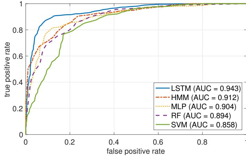
Figure 7.4. ROC curves for fall risk classifiers.
