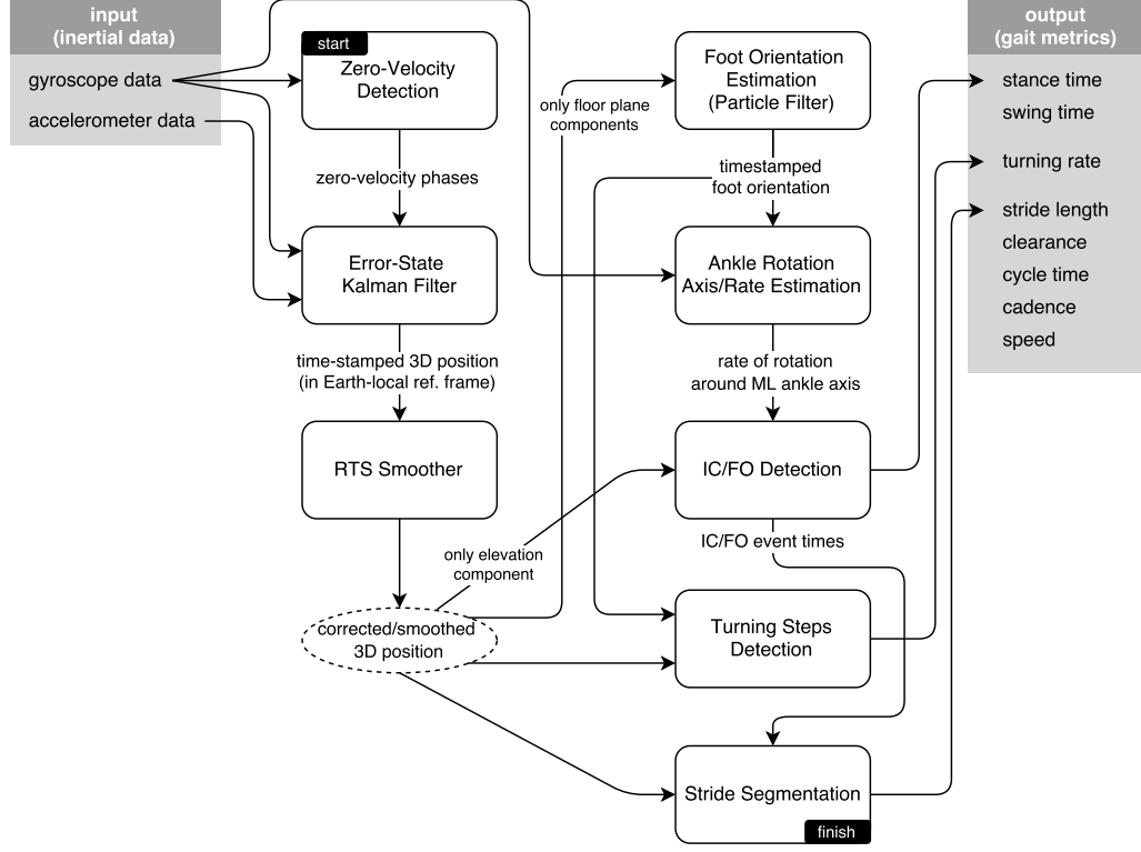
Figure 5.1. Inertial sensor-based gait analysis system block diagram.
