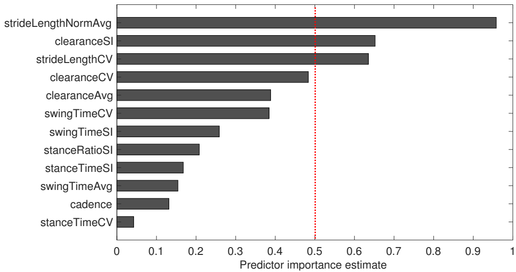
Figure 6.3. Random forest predictor importance estimates.
