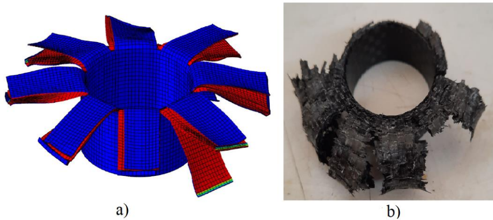
Figure 4.31. Crushing modes of Ø30mm empty tube outwards crushing a) Numerical simulation b) Experimental test.
