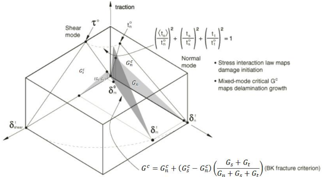
Figure 3.7. Mixed mode traction-separation response of cohesive surfaces [54].
