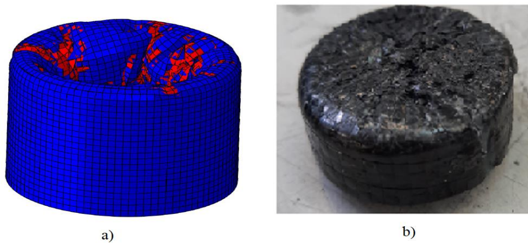
Figure 4.27. Crushing modes of Ø30mm empty tube inwards crushing a) Numerical simulation b) Experimental test.
