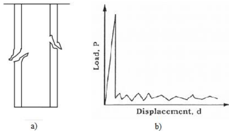
Figure 1.17. Catastrophic crushing behavior a) Crushing mode illustration [13] b) Typical load displacement curve [10].
