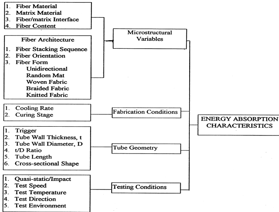
Figure 1.24. General parameters that effects the energy absorption characteristics of a composite tube [6].
