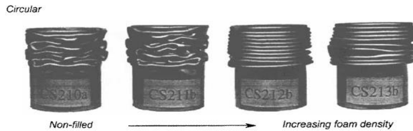
Figure 1.28. Foam filled metallic tube folding subjected to axial crushing as foam density increases [9].
