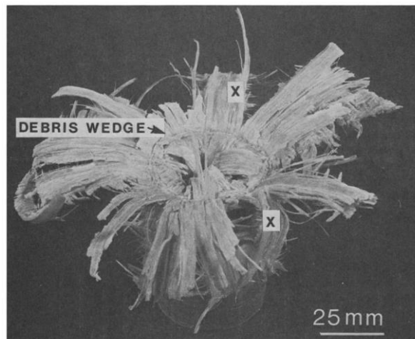
Figure 1.18. Crush zone of a [0/90/90/0] glass fibre-polyester resin tube [10].
