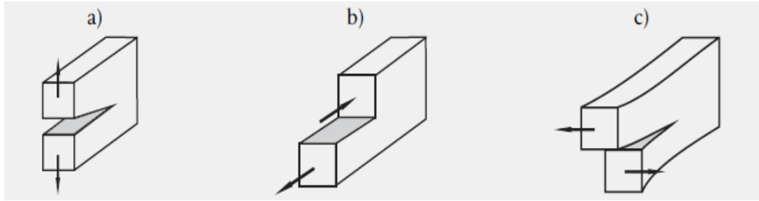
Figure 3.5. Delamination modes, a) mode I b) mode II c) mode III [51].
