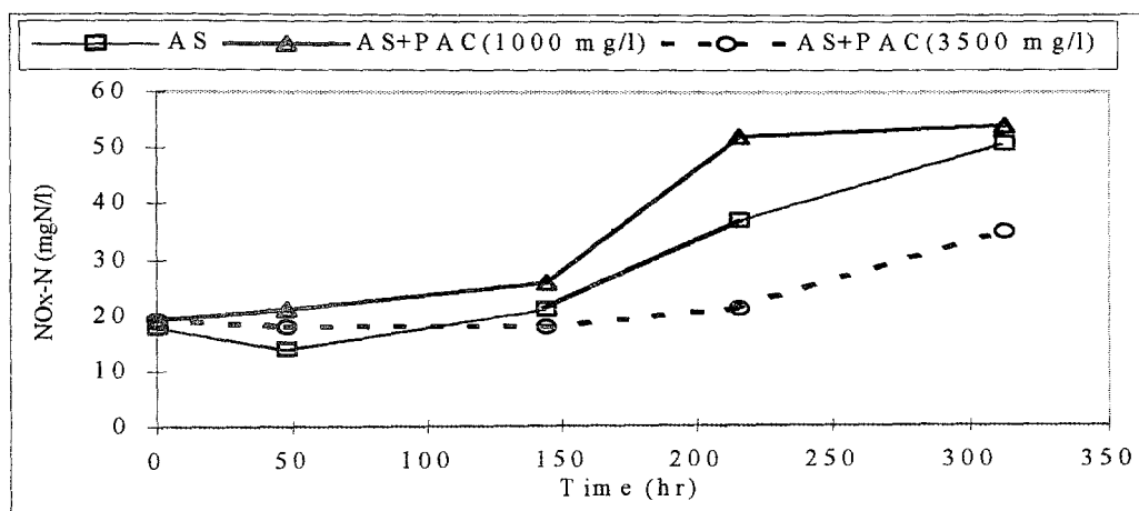
FIGURE 4.25. NO x -N Profiles in BATCH RUN 5.
