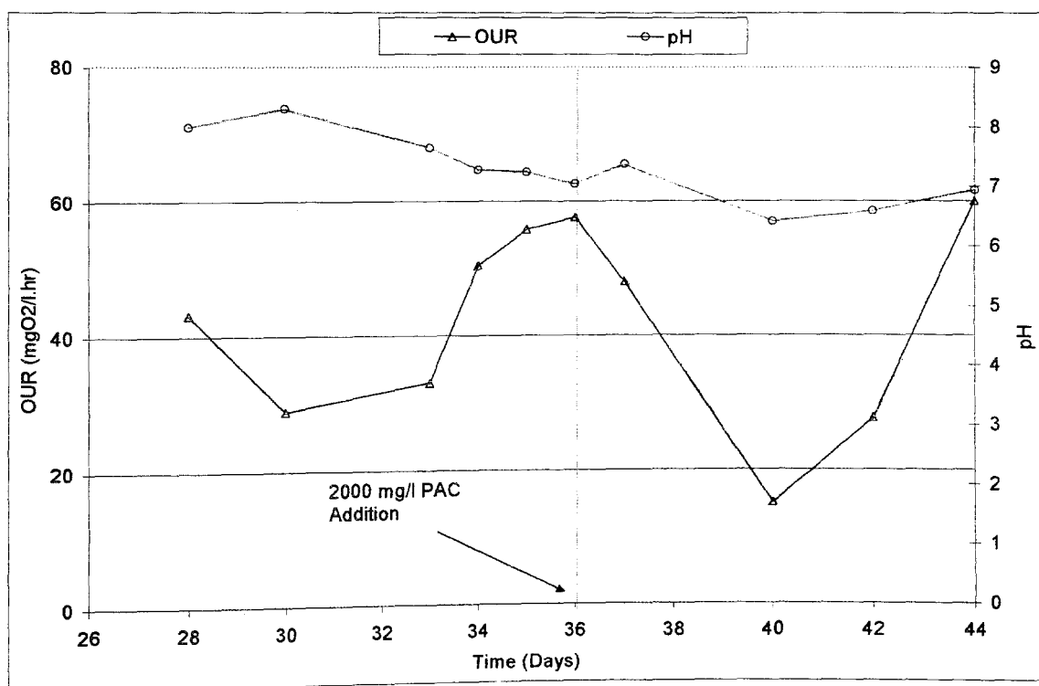
FIGURE 4.49. OUR and pH Profiles in CFSTR Operation (Leachate Ratio: 13.3% by volume).
