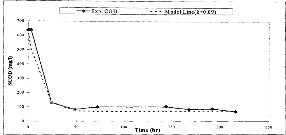
FIGURE 4.15. Braha’s model for SCOD removal in BATCH RUN 2.
