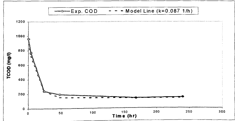
FIGURE 4.16. Braha’s model for TCOD removal in BATCH RUN 3.
