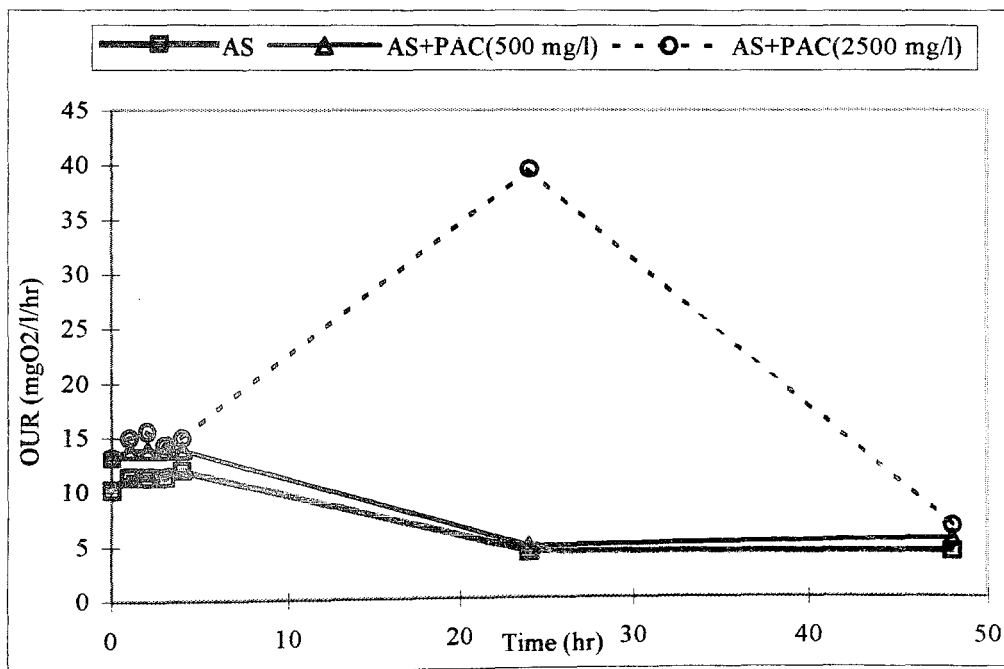
FIGURE 4.30. OUR Profiles in BATCH RUN 4.
