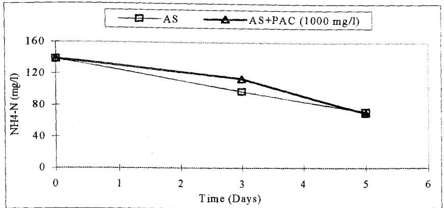
FIGURE 4.40. \text{NH}_4\text{-N} Profiles in SCFB RUN1.
