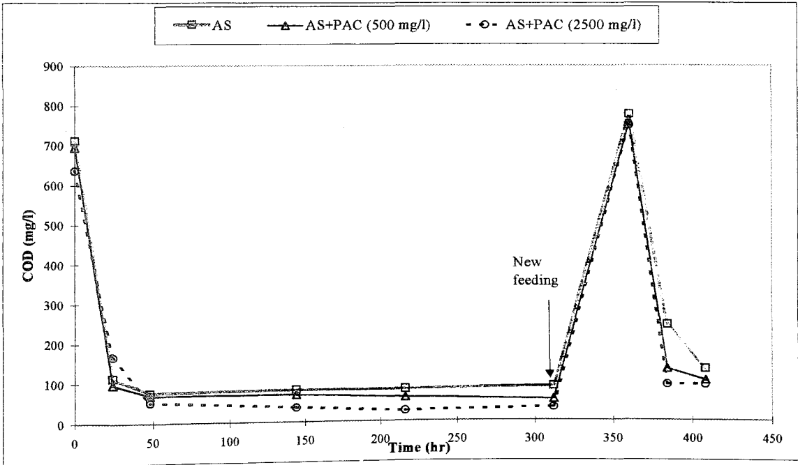
FIGURE 4.7. COD Profiles in BATCH RUN 4.
