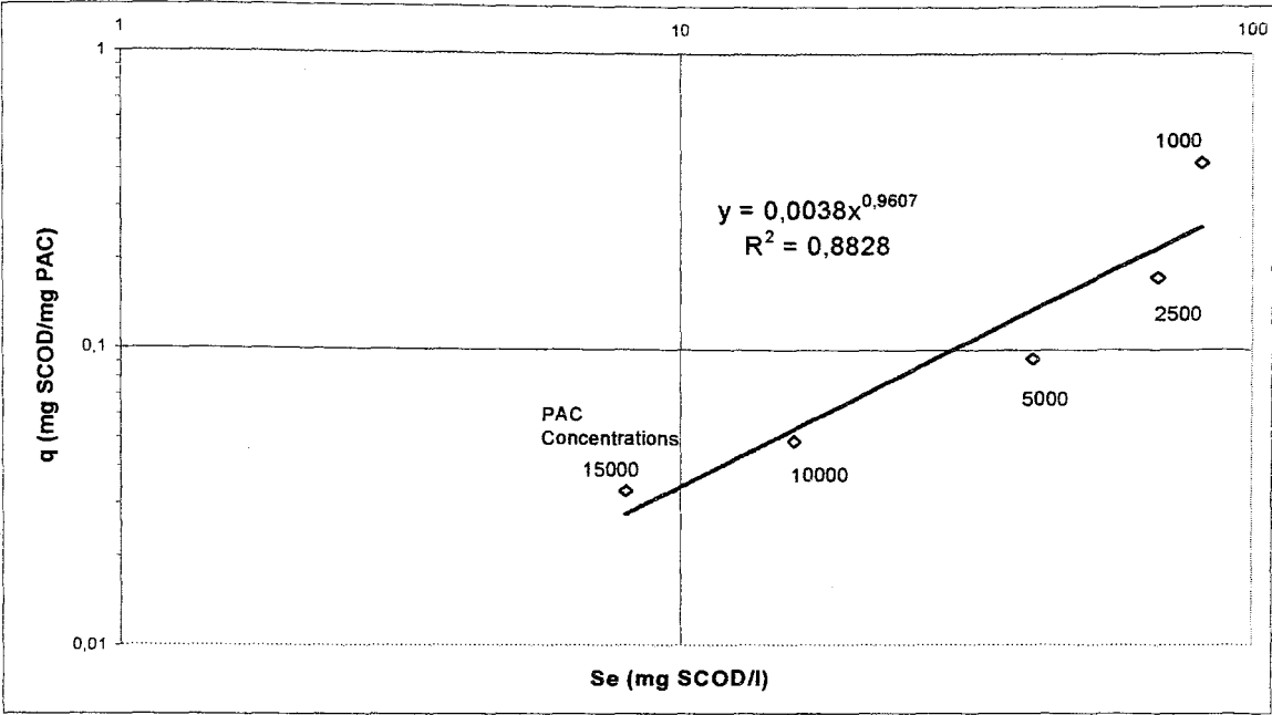
FIGURE 4.1. Freundlich adsorption isotherm for diluted leachate (5%) at high PAC concentrations
