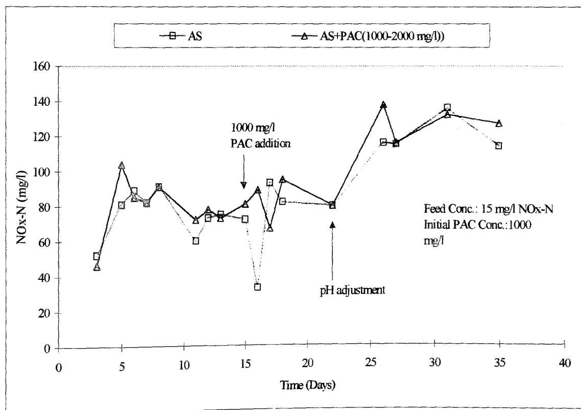
FIGURE 4.43. \text{NO}_x\text{-N} Profiles in SCFB RUN 2.
