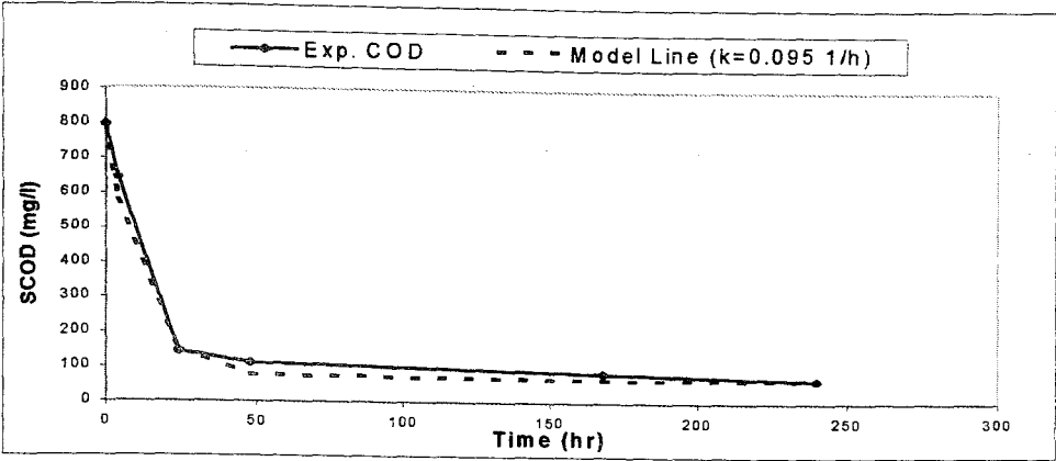
FIGURE 4.17. Braha's model for SCOD removal in BATCH RUN 3.
