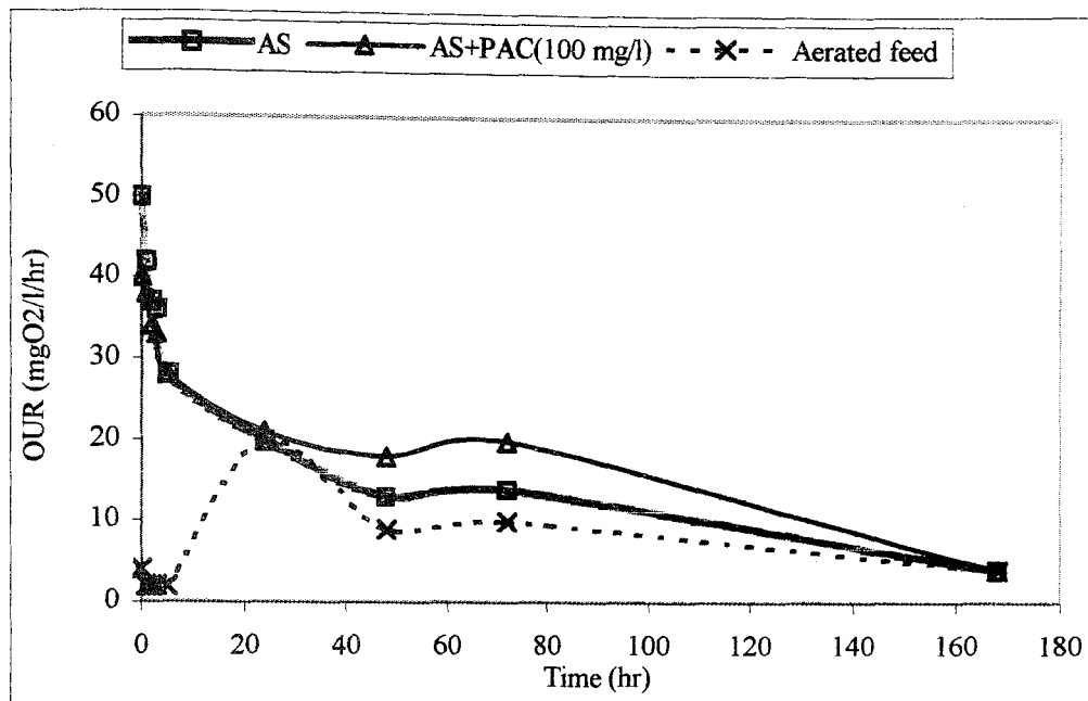
FIGURE 4.29. OUR Profiles in BATCH RUN 3.
