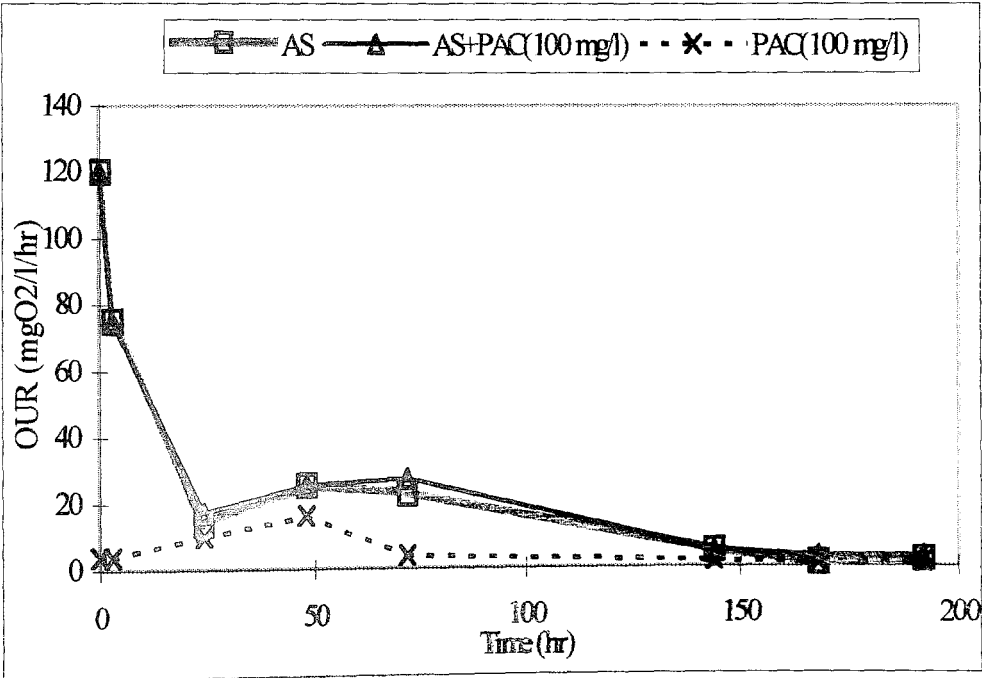
FIGURE 4.28. OUR Profiles in BATCH RUN 2.
