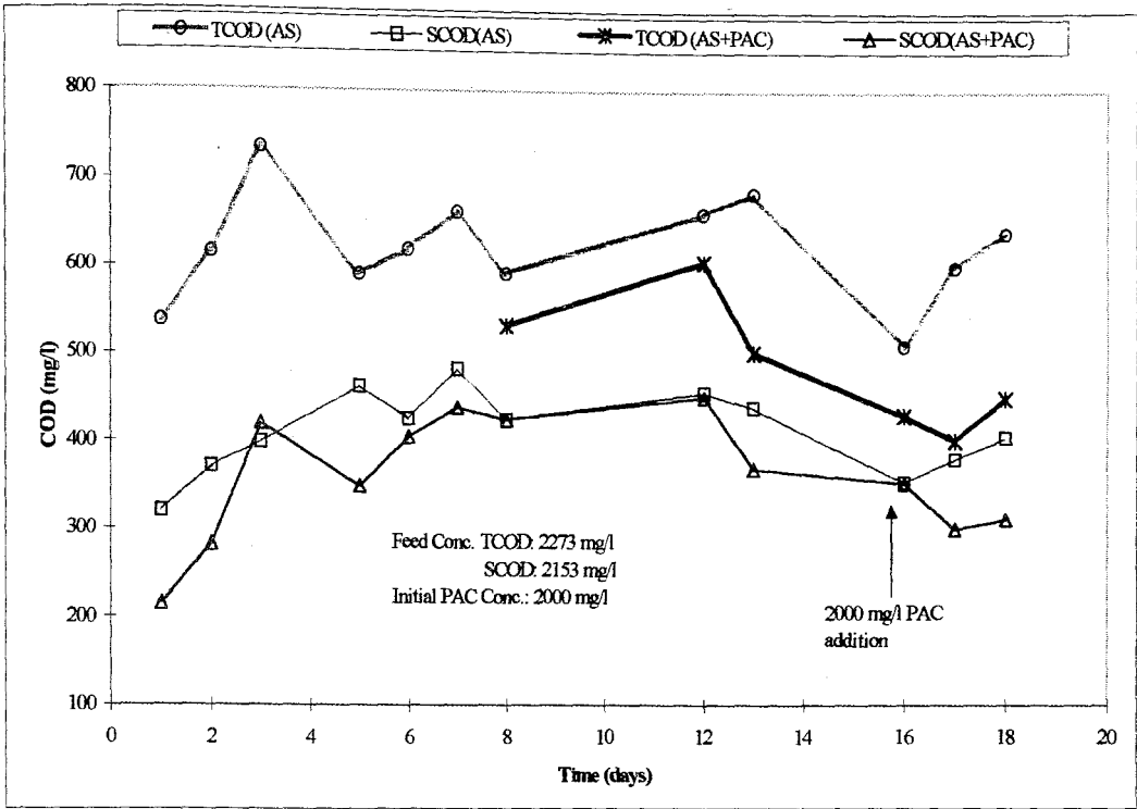
FIGURE 4.36. COD Profiles in SCFB RUN 3.
