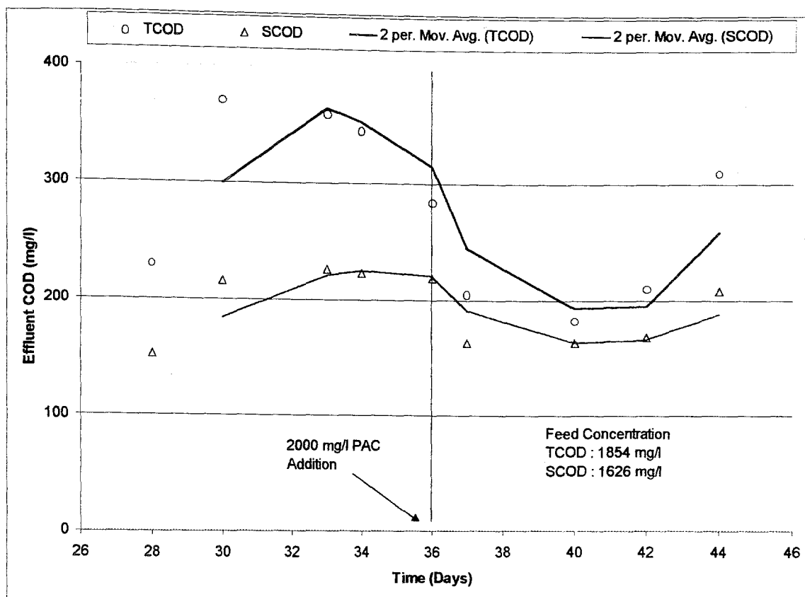
FIGURE 4.48. COD Profiles in CFSTR Operation (Leachate Ratio: 13.3% by volume).
