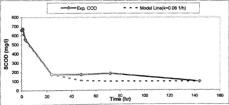
FIGURE 4.13. Braha’s model for SCOD removal in BATCH RUN 1
