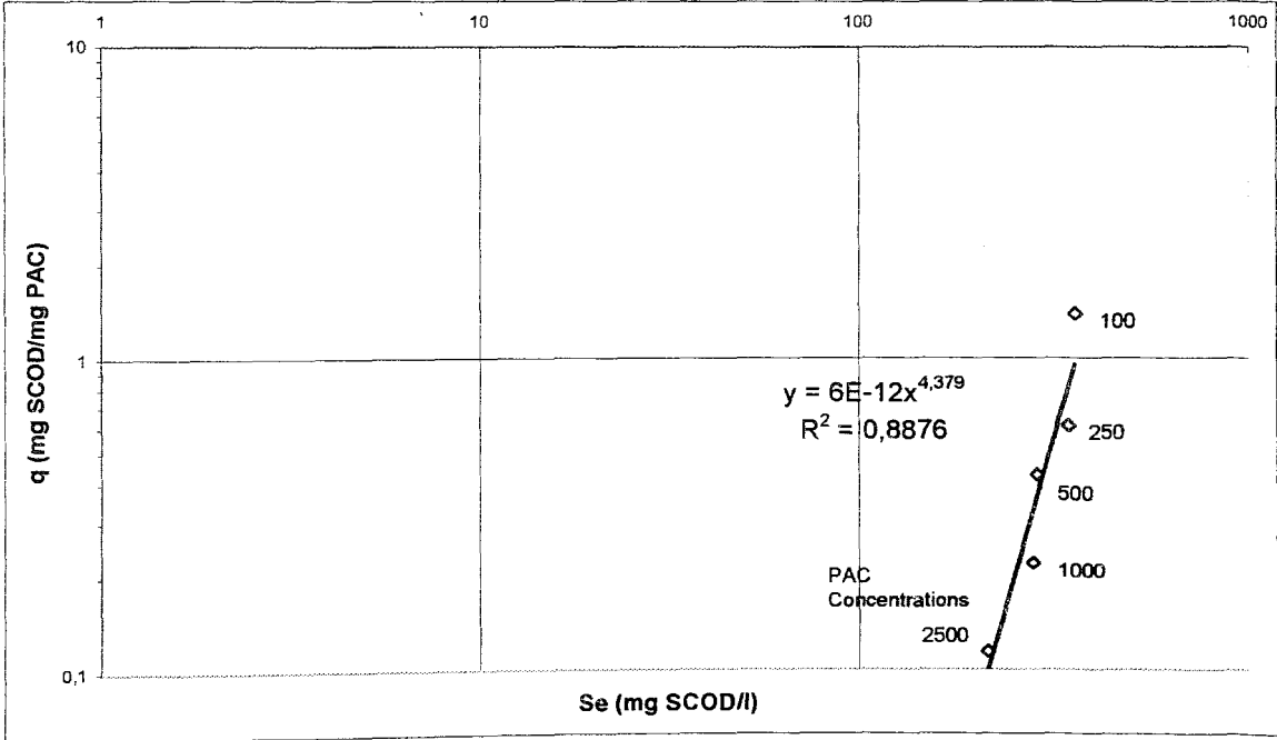
FIGURE 4.2. Freundlich adsorption isotherm for diluted leachate (5%) at low PAC concentrations.
