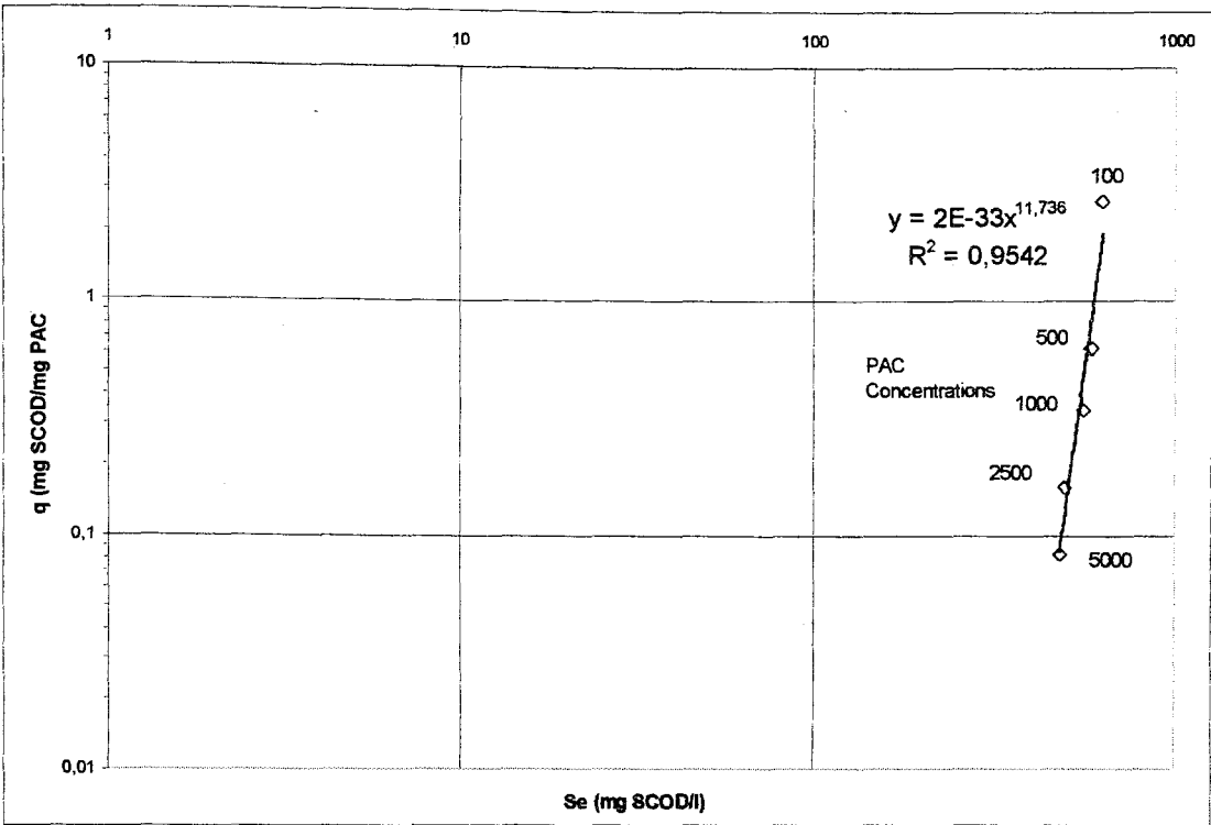
FIGURE 4.3. Freundlich adsorption isotherm for combined leachate and synthetic domestic wastewater (Leachate ratio: 5% by volume).
