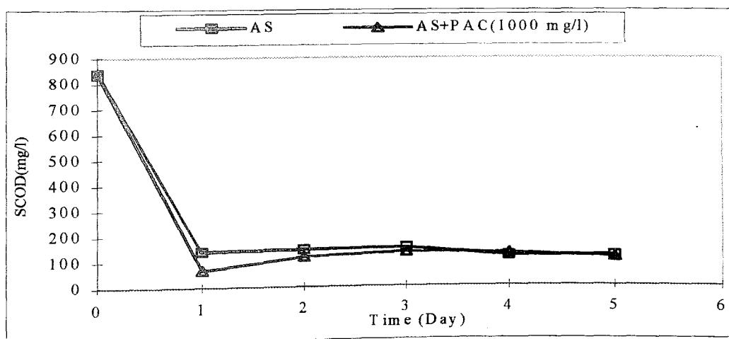
FIGURE 4.33. COD Profiles in SCFB RUN 1.
