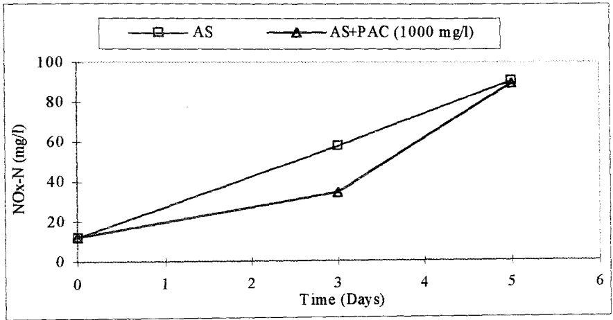
FIGURE 4.41. \text{NO}_x\text{-N} Profiles in SCFB RUN 1.
