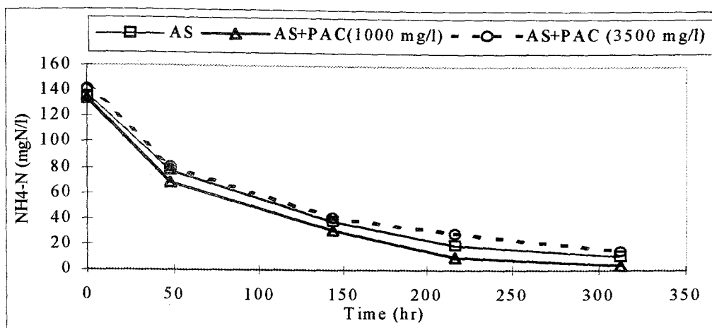
FIGURE 4.24. NH 4 -N Profiles in BATCH RUN 5.
