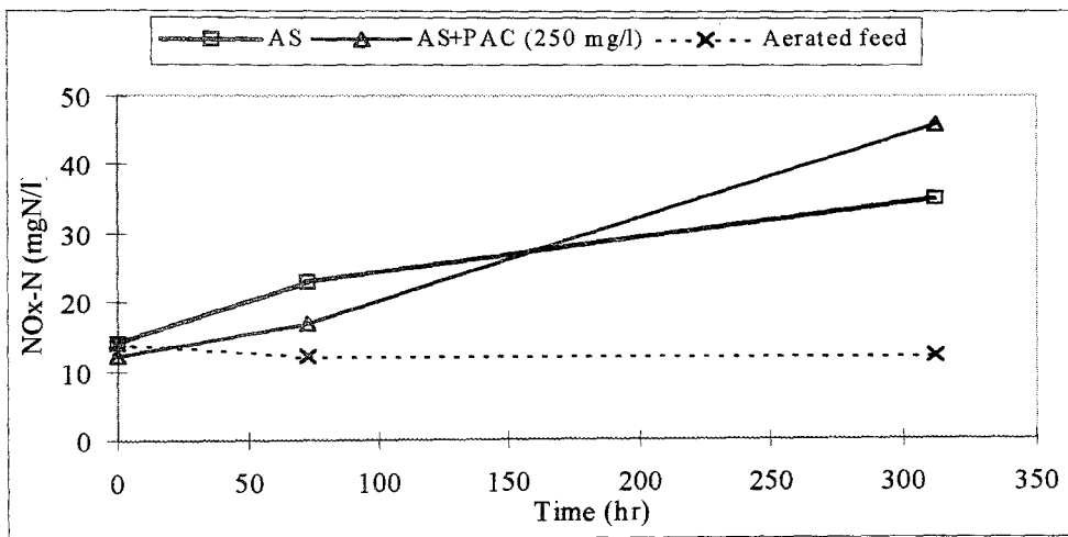
FIGURE 4.22. \text{NO}_x\text{-N} Profiles in BATCH RUN 3.
