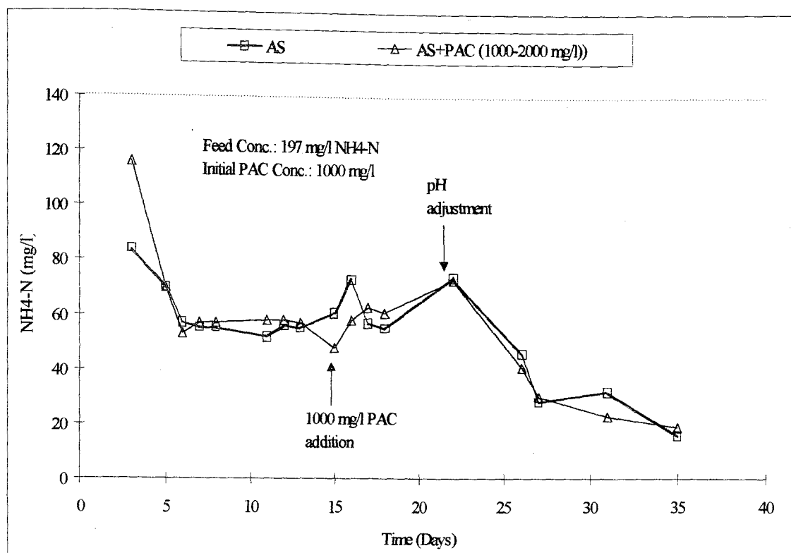
FIGURE 4.42. \text{NH}_4\text{-N} Profiles in SCFB RUN 2.
