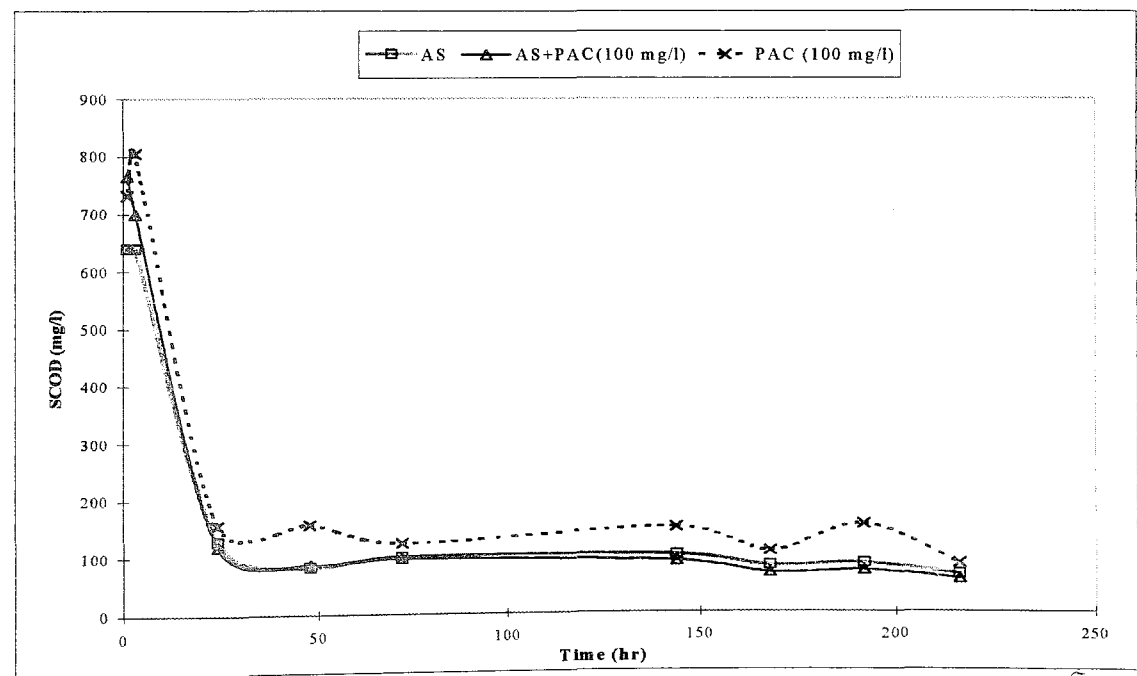
FIGURE 4.5. COD Profiles in BATCH RUN 2.
