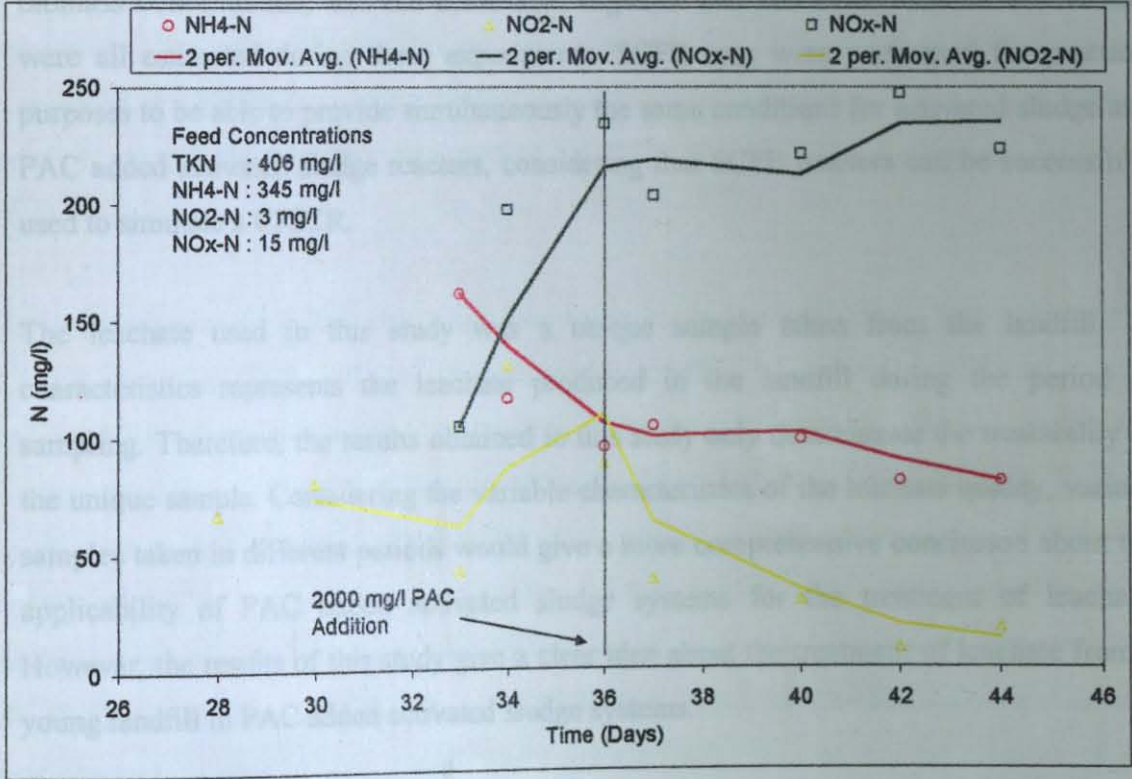
FIGURE 4.51. Nitrogen Profiles in CFSTR Operation (Leachate ratio: 13.3% by volume).
