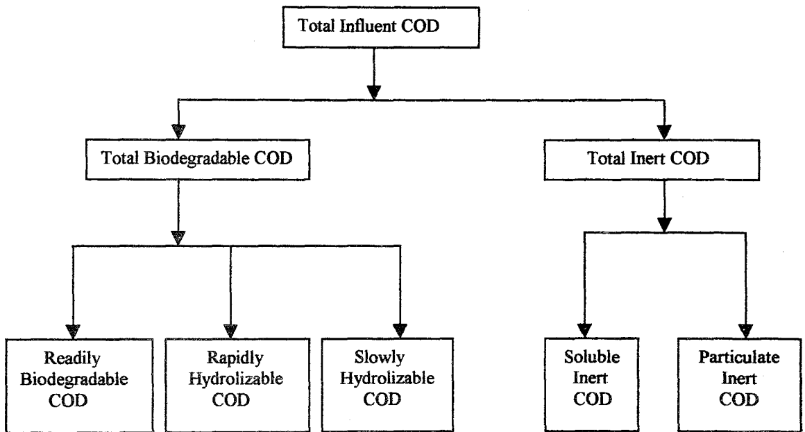
FIGURE 2.3. Distribution of COD fractions in wastewaters (12).
