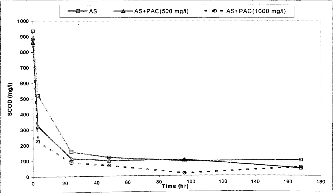
FIGURE 4.9. COD Profiles in BATCH RUN 6.
