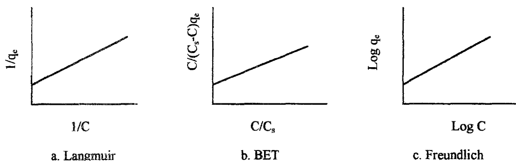
FIGURE 2.1. Linear forms for graphical representation of adsorption equations (7).
