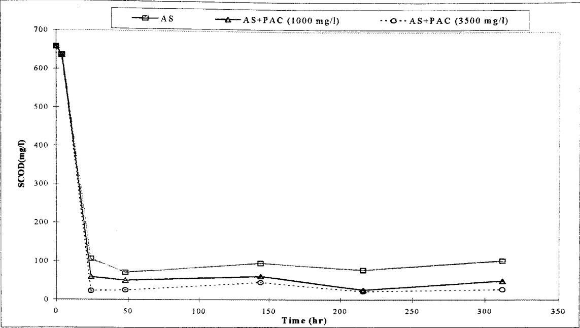
FIGURE 4.8. COD Profiles in BATCH RUN 5.
