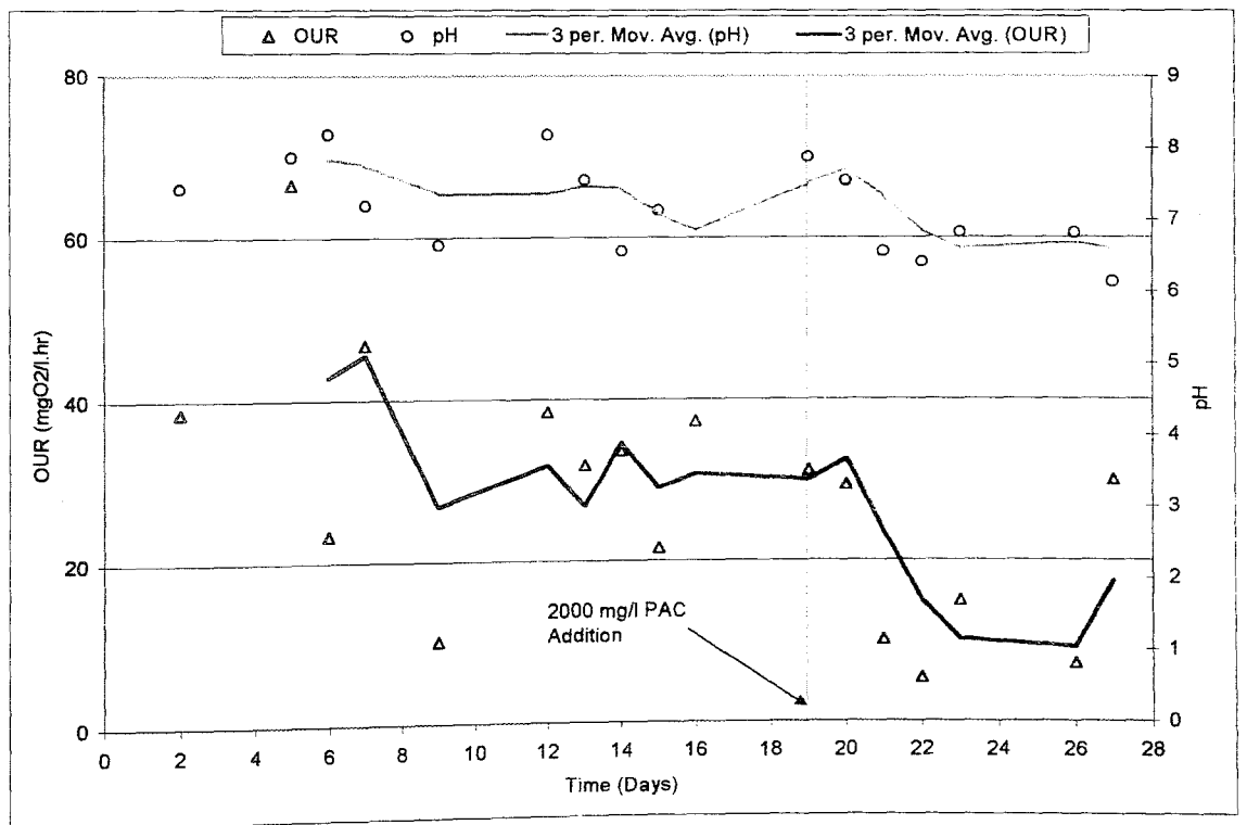
FIGURE 4.47. OUR and pH Profiles in CFSTR Operation (Leachate Ratio: 6.7% by volume).
