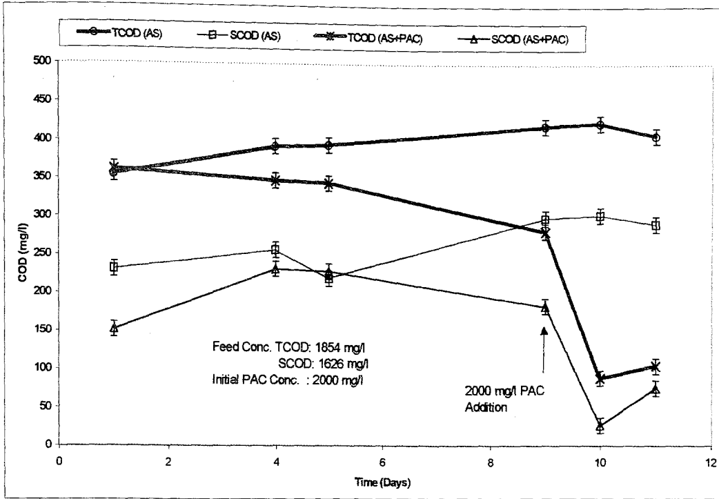
FIGURE 4.38. COD Profiles in SCFB RUN 4.
