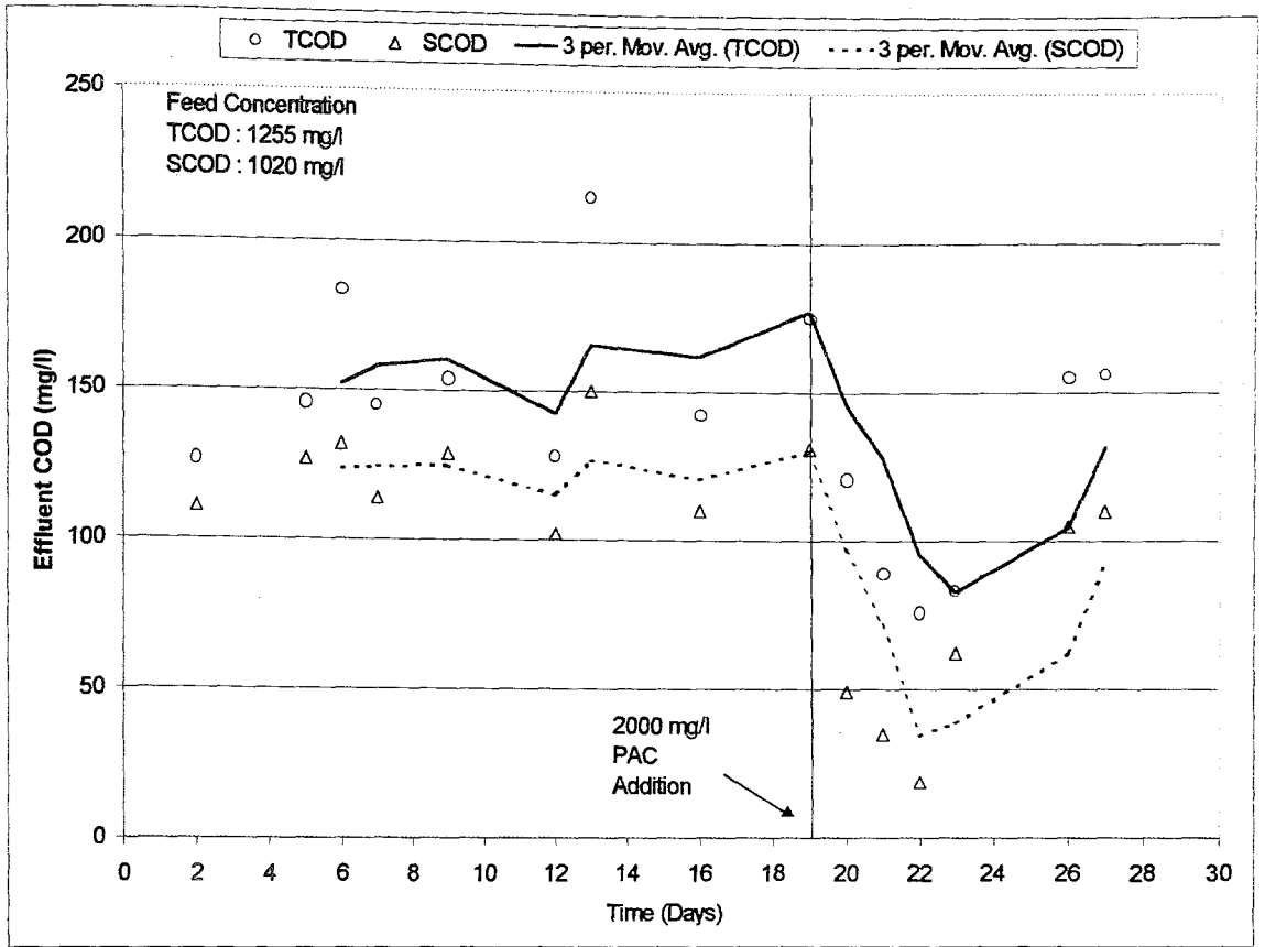
FIGURE 4.46. COD Profiles in CFSTR Operation (Leachate Ratio: 6.7% by volume).
