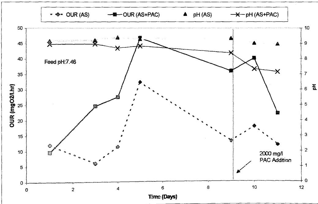
FIGURE 4.39. OUR and pH Profiles in SCFB RUN 4.
