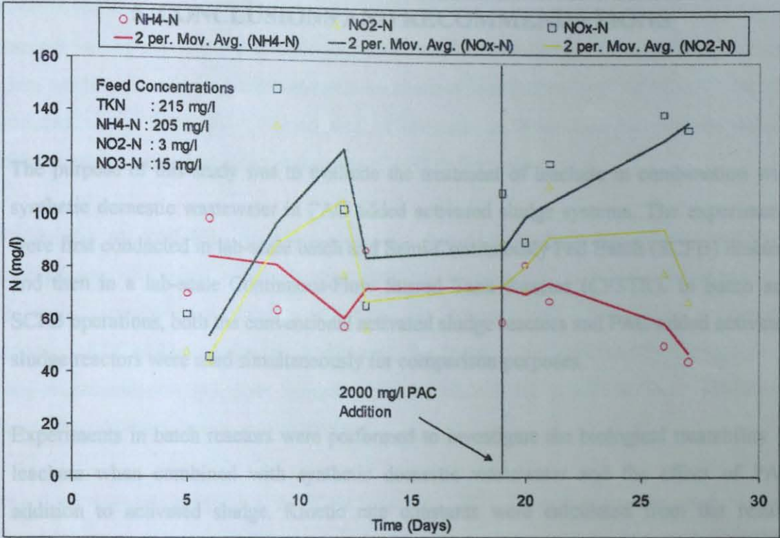
FIGURE 4.50. Nitrogen Profiles in CFSTR Operation (Leachate ratio: 6.7% by volume).
