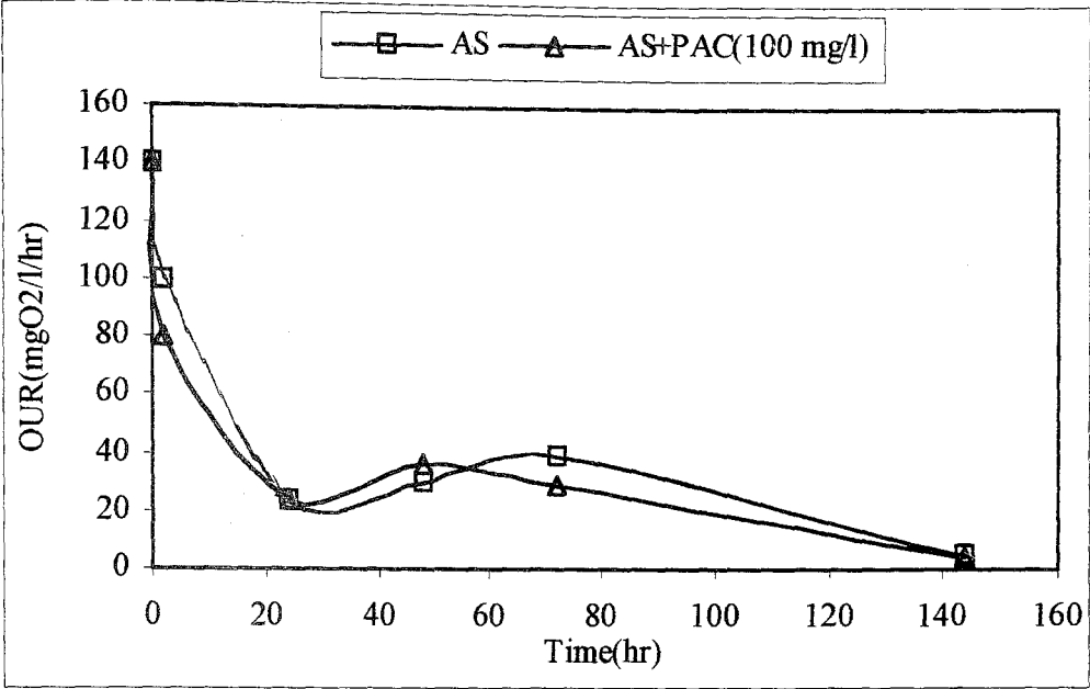
FIGURE 4.27. OUR Profiles in BATCH RUN 1.
