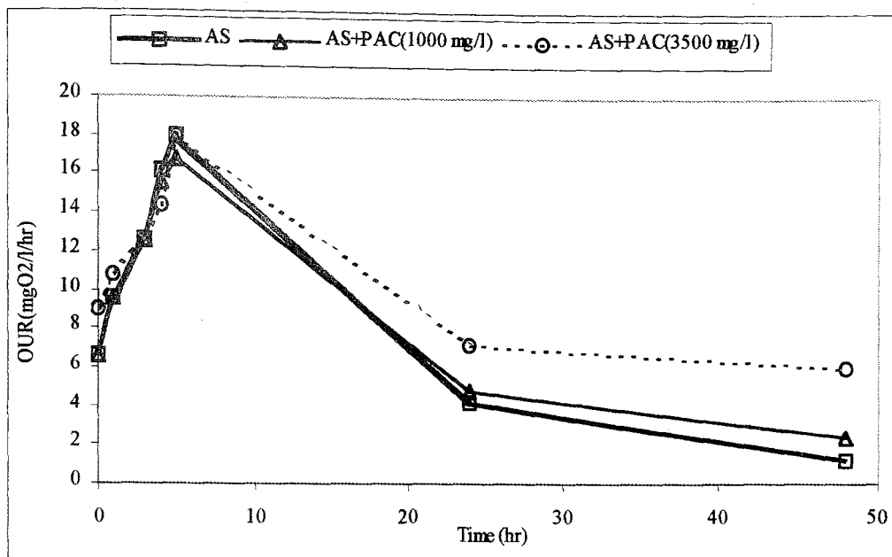
FIGURE 4.31 OUR Profiles in BATCH RUN 5.
