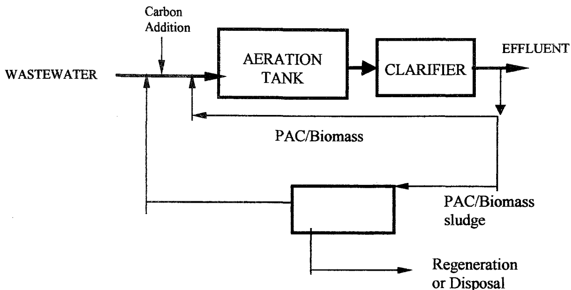
FIGURE 2.4. Schematic representation of a typical powdered activated carbon- activated sludge system (4).
