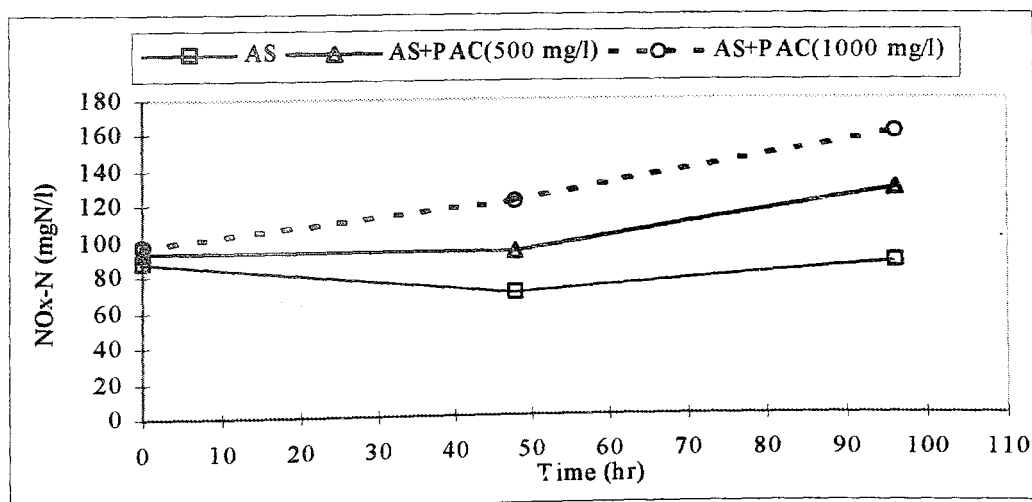
FIGURE 4.26. NO x -N Profiles in BATCH RUN 6.
