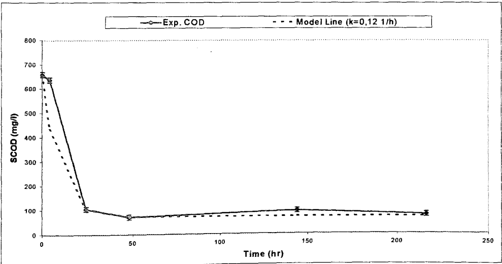
FIGURE 4.19. Braha's model for SCOD removal in BATCH RUN 5.
