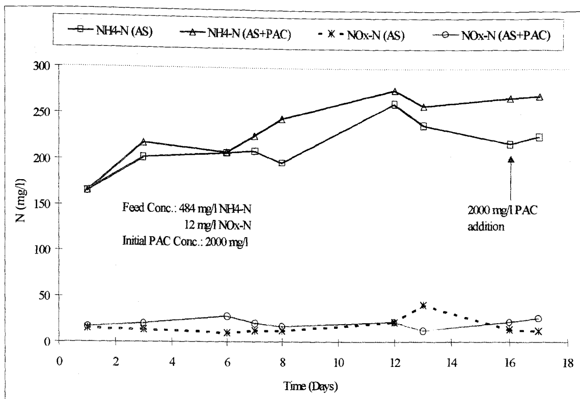
FIGURE 4.44. Nitrogen Profiles in SCFB RUN 3.
