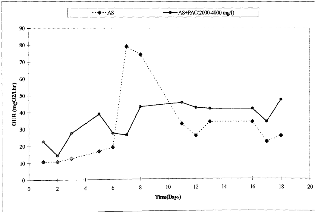
FIGURE 4.37. OUR Profiles in SCFB RUN 3.
