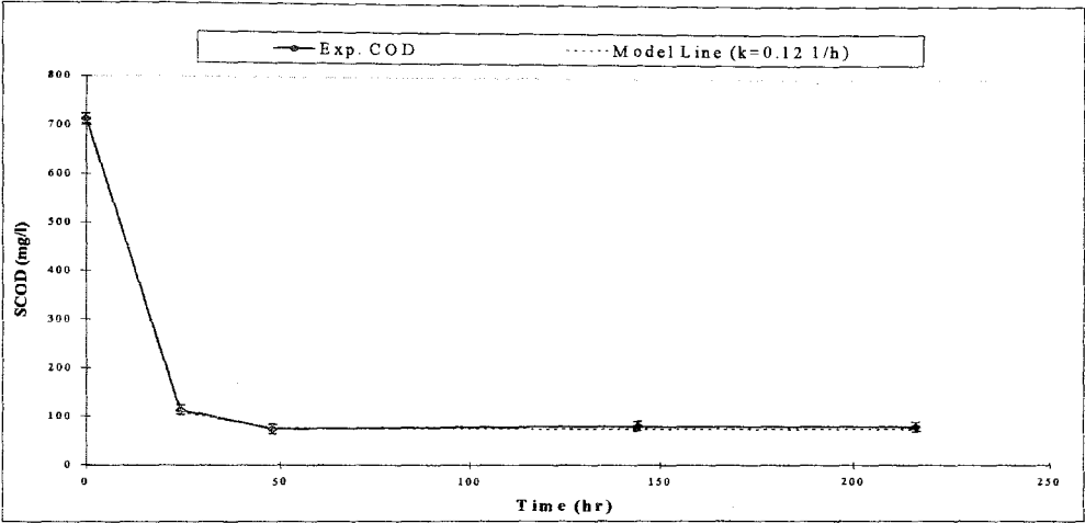
FIGURE 4.18. Braha's model for SCOD removal in BATCH RUN 4.
