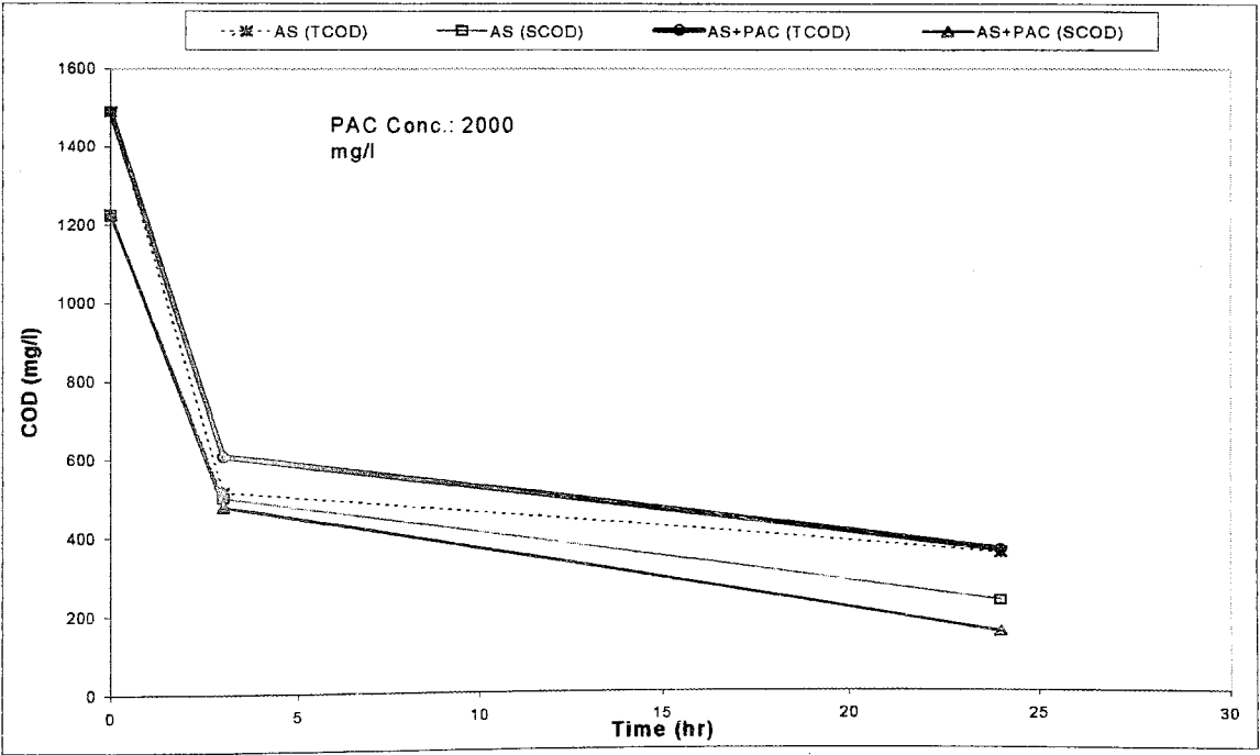
FIGURE 4.11. COD Profiles in BATCH RUN 10.
