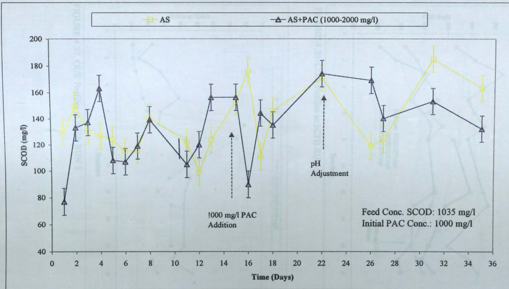
FIGURE 4.35. COD Profiles in SCFB RUN 2.
