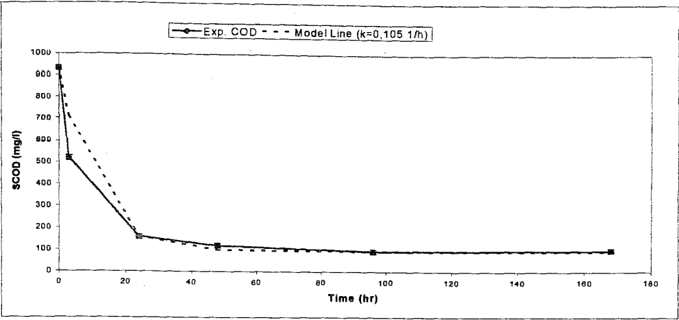
FIGURE 4.20. Braha’s model for SCOD removal in BATCH RUN 6.
