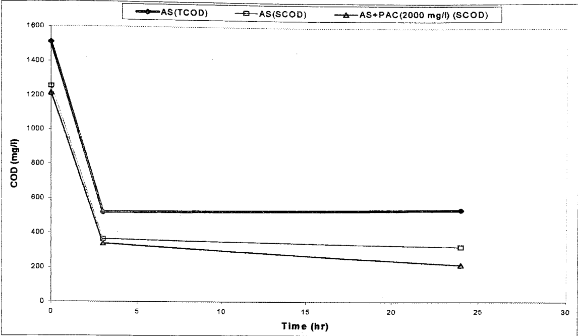
FIGURE 4.10. COD Profiles in BATCH RUN 9.
