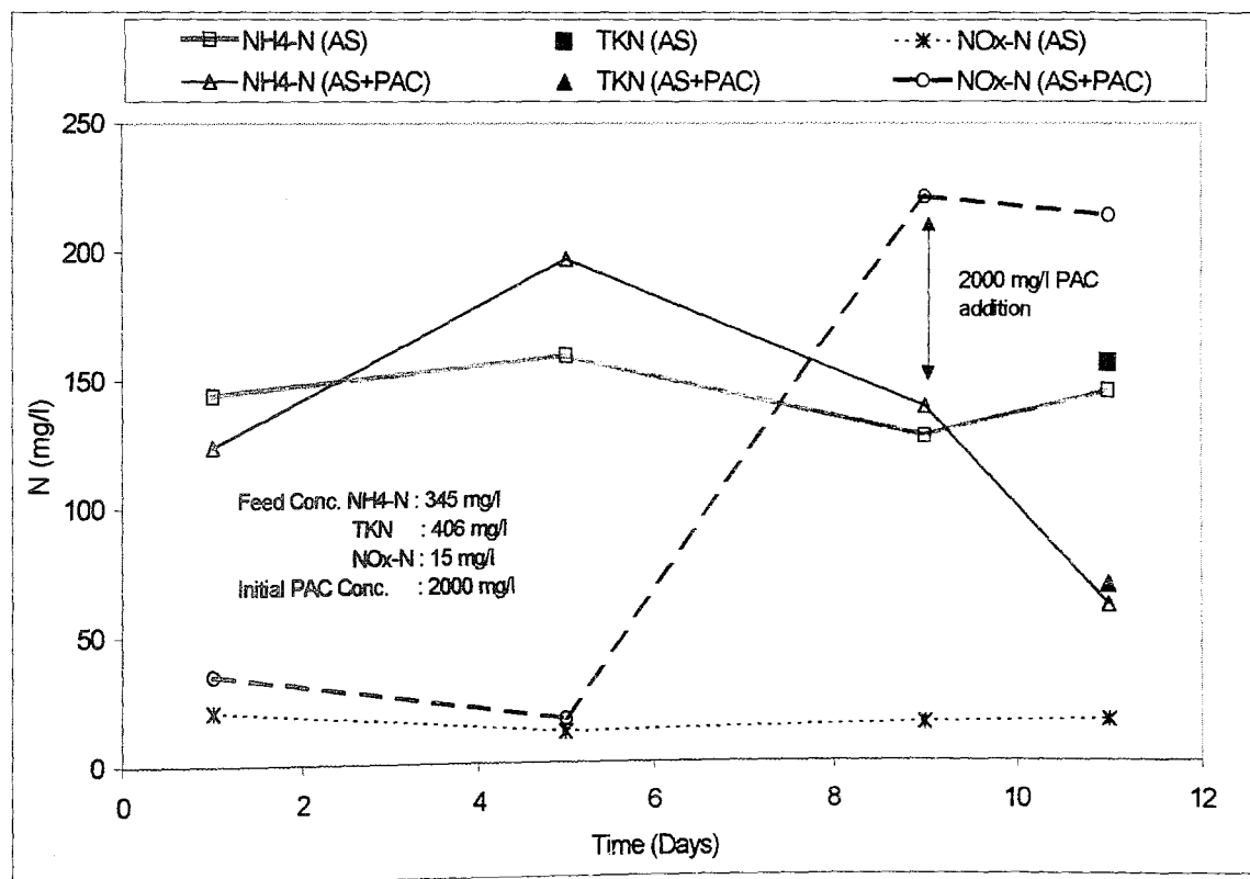
FIGURE 4.45. Nitrogen Profiles in SCFB RUN 4.
