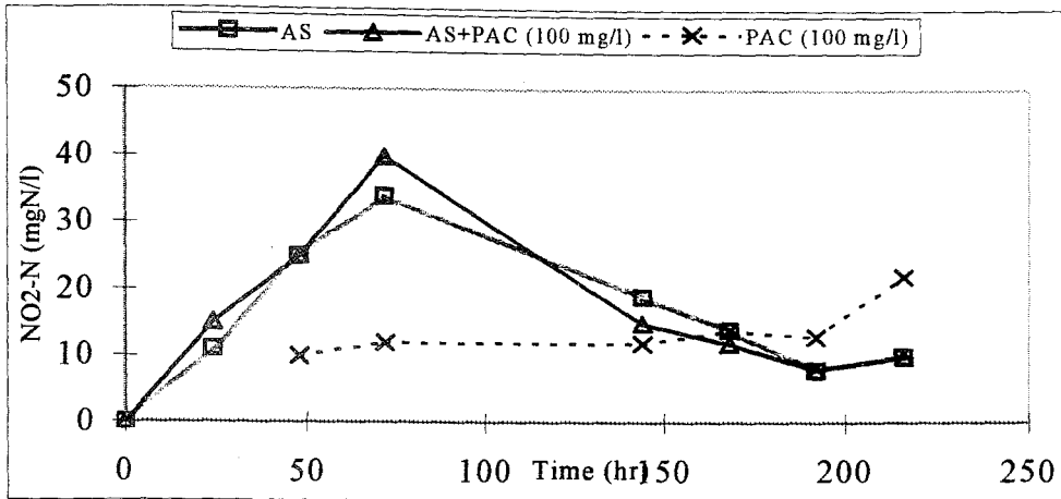
FIGURE 4.21. \text{NO}_2\text{-N} Profiles in BATCH RUN 2.
