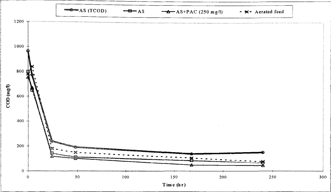
FIGURE 4.6. COD Profiles in BATCH RUN 3.
