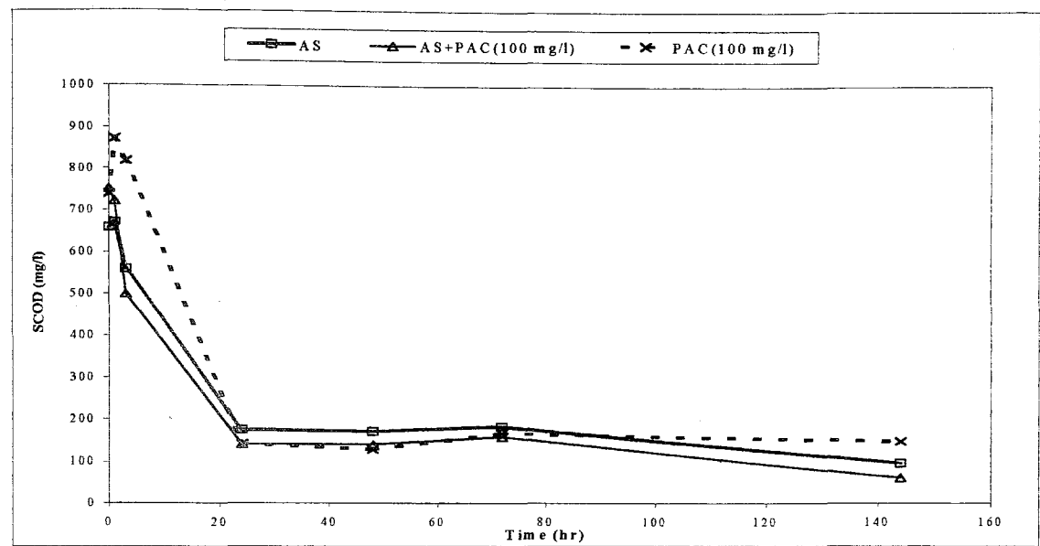
FIGURE 4.4. COD Profiles in BATCH RUN 1.
