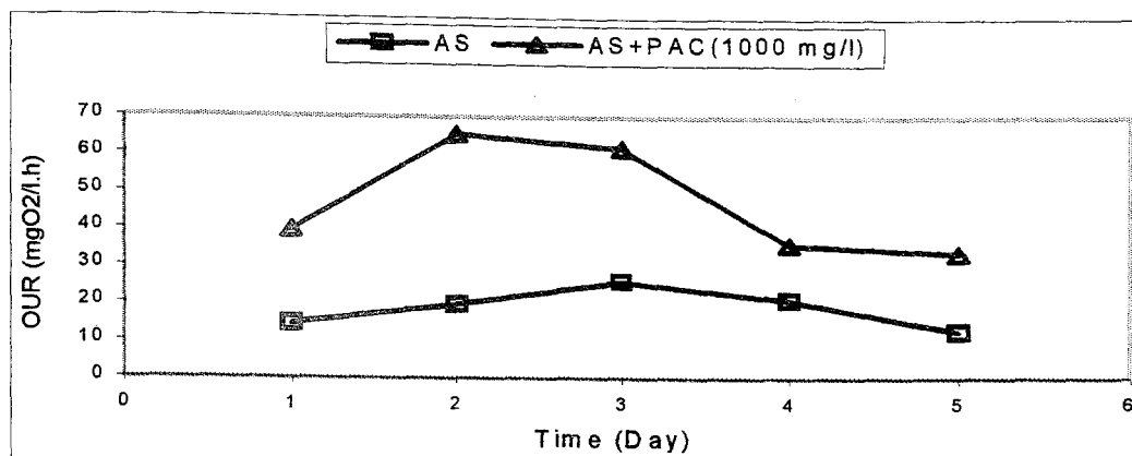
FIGURE 4.34. OUR Profiles in SCFB RUN 1.
