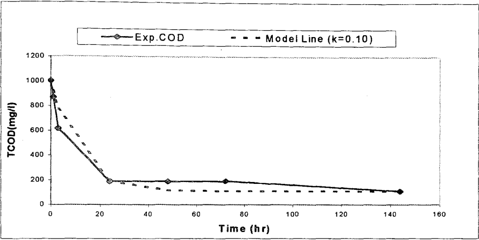
FIGURE 4.12. Braha’s model for TCOD removal in BATCH RUN 1.
