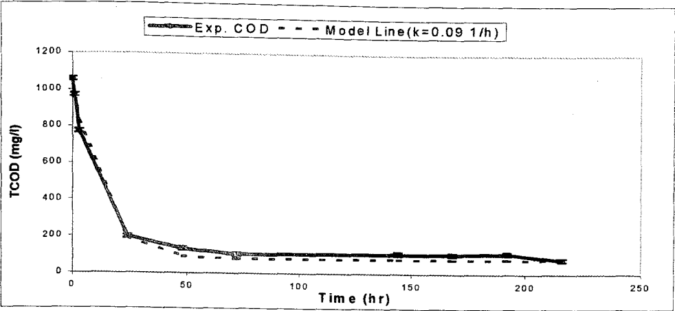
FIGURE 4.14. Braha’s model for TCOD removal in BATCH RUN 2.
