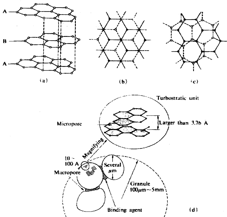
FIGURE 2.2. Graphite structure (a,b) and turbostratic structure (c) of activated carbon. Conceptual illustration of granular activated carbon (d) (8).
