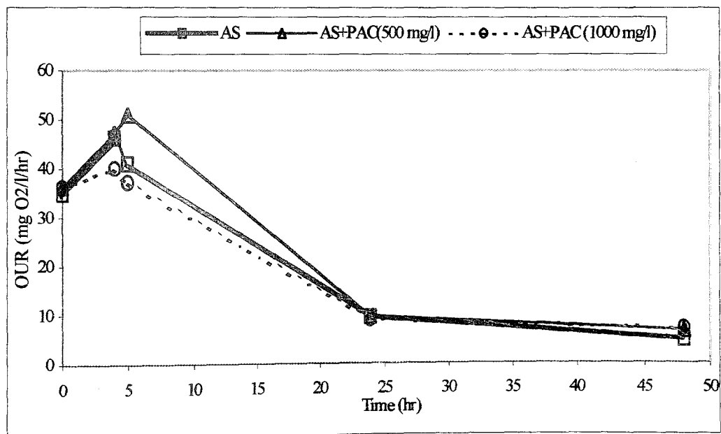
FIGURE 4.32. OUR Profiles in BATCH RUN 6.
