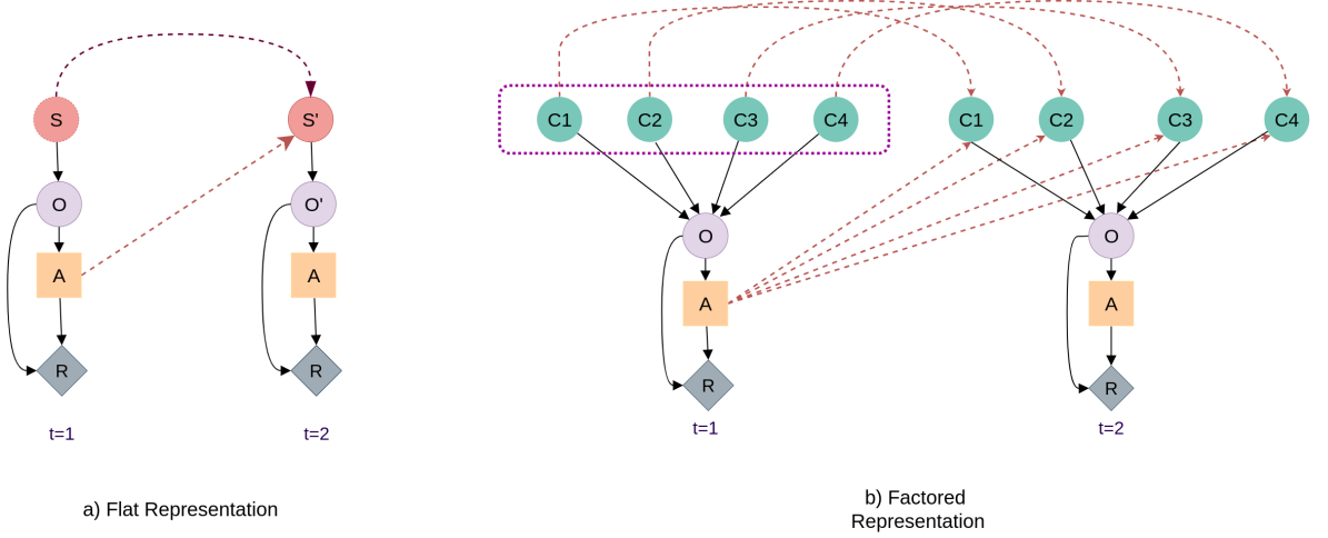
Figure 3.7: POMDP representations.
