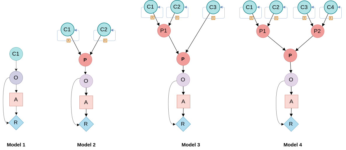
Figure 4.1: Empirical models.
