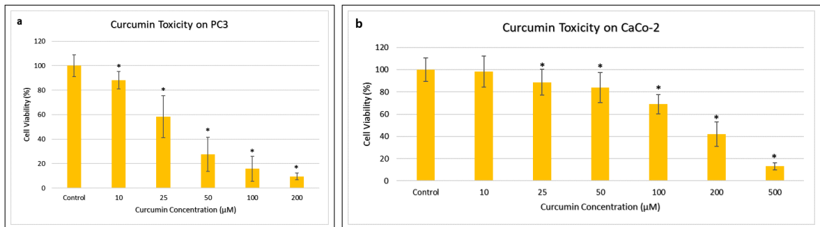
Figure 4.3 Curcumin shows dose-dependent antitumor effect on both PC-3 (a) and Caco-2 cells (b). The groups that are statistically significantly different from the Control group were labelled (*: p < 0.05 ).
