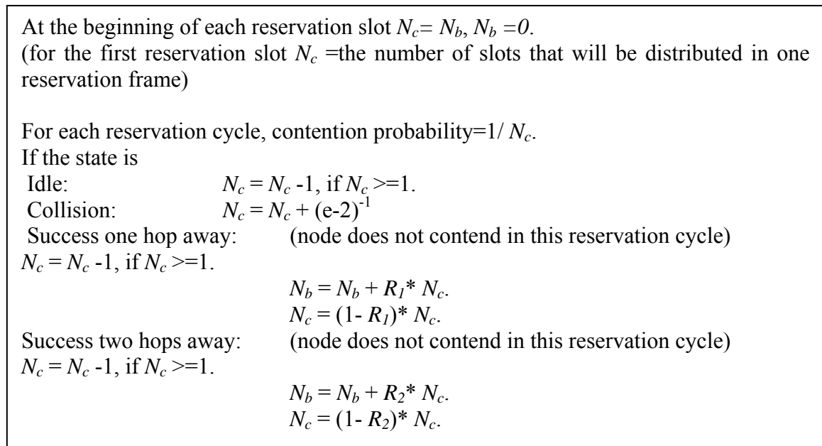
Figure 4.5. Slot request update procedure pseudocode.
