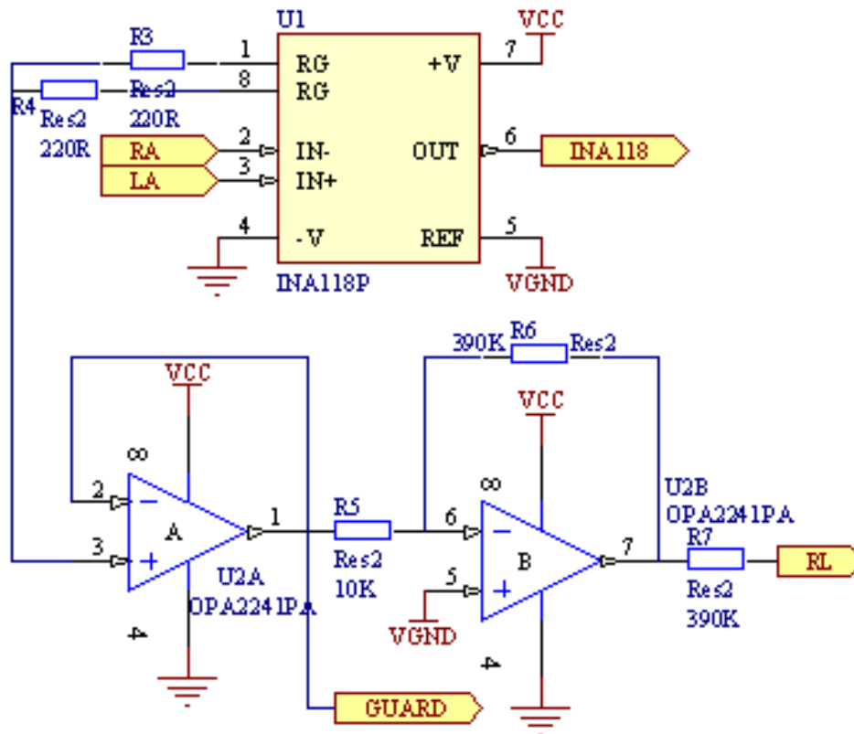
Figure 3.5 Guarding and driven right leg circuit.
