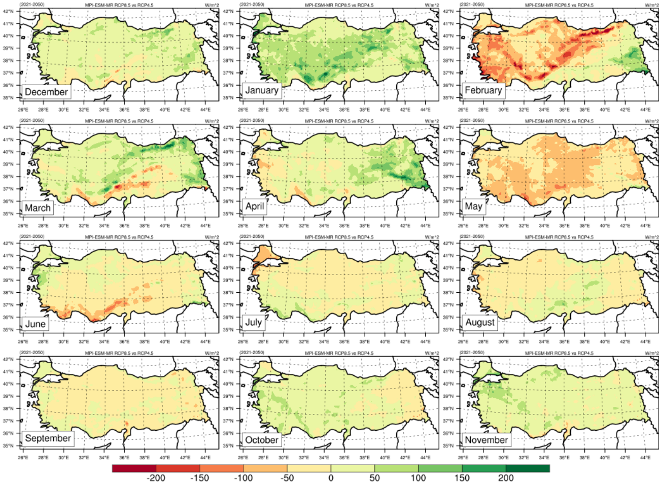
Figure 20. Turkey Monthly Average Wind Power Density Change 100m RCP8.5 Scenario vs RCP4.5 Scenario Data Results (2021-2050).
