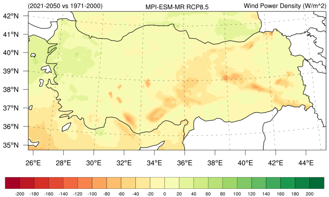
Figure C.4. Turkey Average Wind Power Density Change 100m RCP8.5 Scenario vs Historical Data Results (2021-2050 vs 1971-2000).
