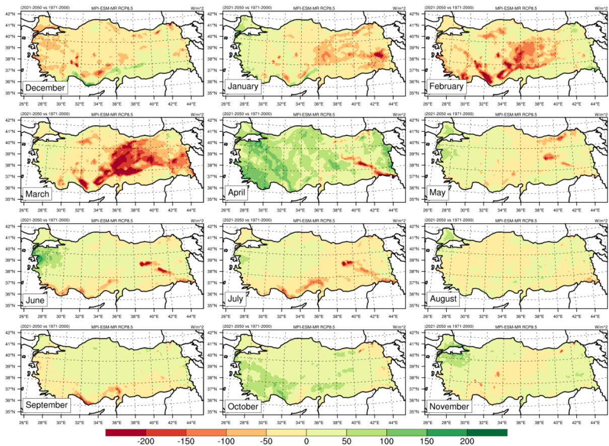
Figure 19. Turkey Monthly Average Wind Power Density Change 100m RCP8.5 Scenario vs Historical Data Results (2021-2050 vs 1971-2000).
