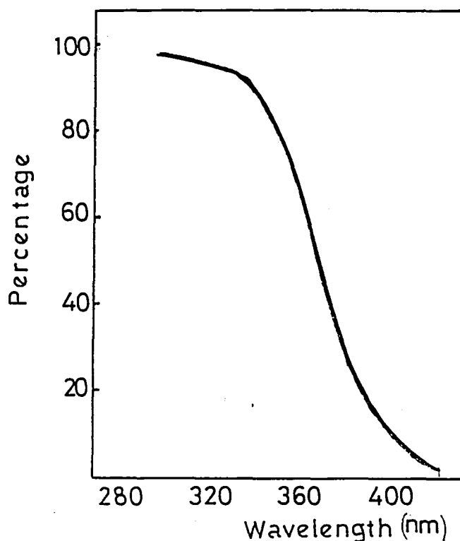
Figure 2.7. Anatase absorption
