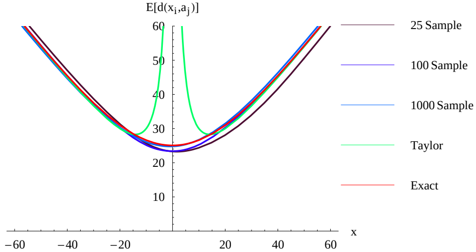
Figure 6.1. Sensitivity for sample size for symmetric distribution: Average distance vs Taylor's approximation for the Euclidean norm
