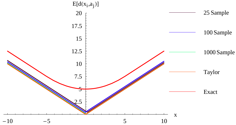
Figure 6.7. Sensitivity to sample size for symmetric distributions: Taylor approximation with exact and estimated distribution parameters for the rectilinear distance
