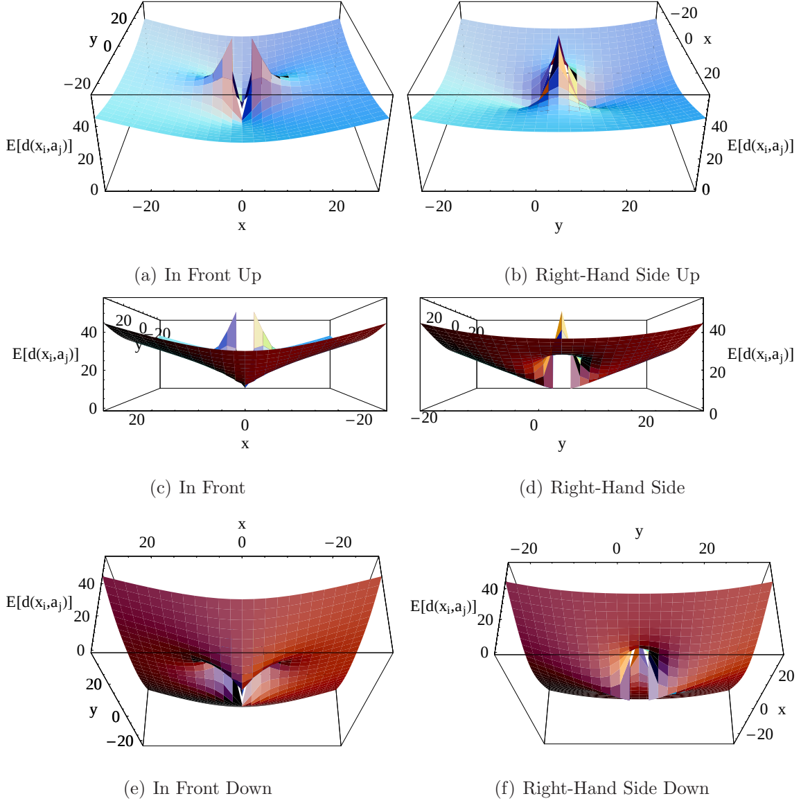
Figure 4.6. Taylor Approximation for the Euclidean distance
