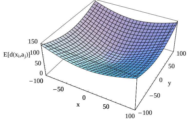
Figure 4.4. Improved Taylor Approximation for the Euclidean distance
