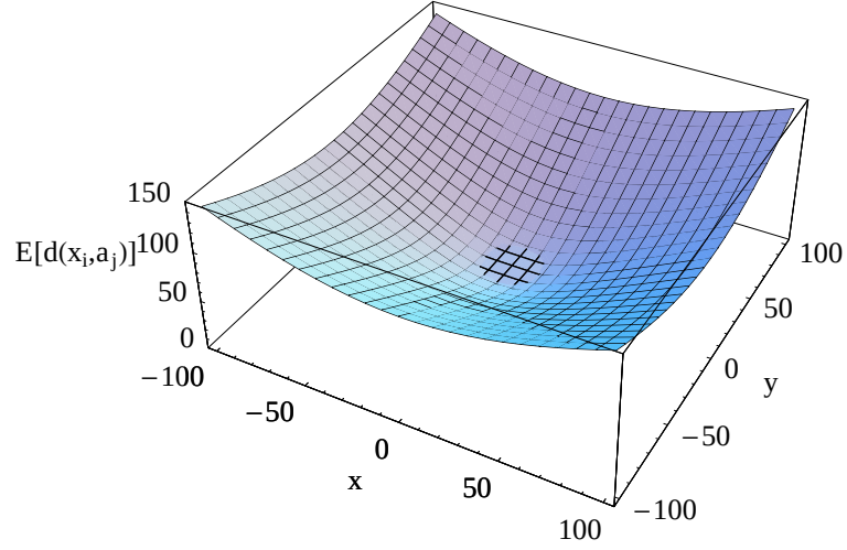
Figure 4.5. Superposition of the improved Taylor Approximation and exact expected distances for the Euclidean distance
