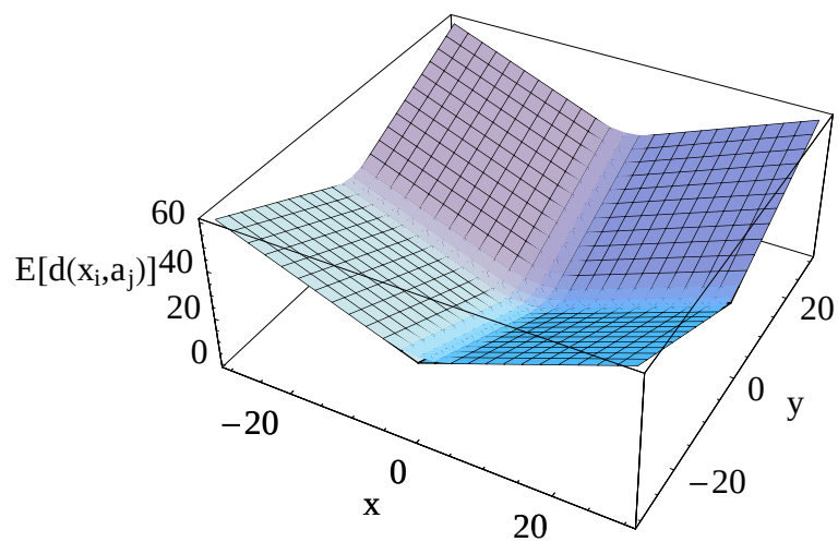
Figure 4.9. Superposition of the exact expected distances and Taylor Approximation for the rectilinear distance
