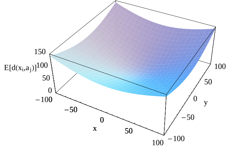
Figure 4.2. Exact expected distances for the Euclidean distance
