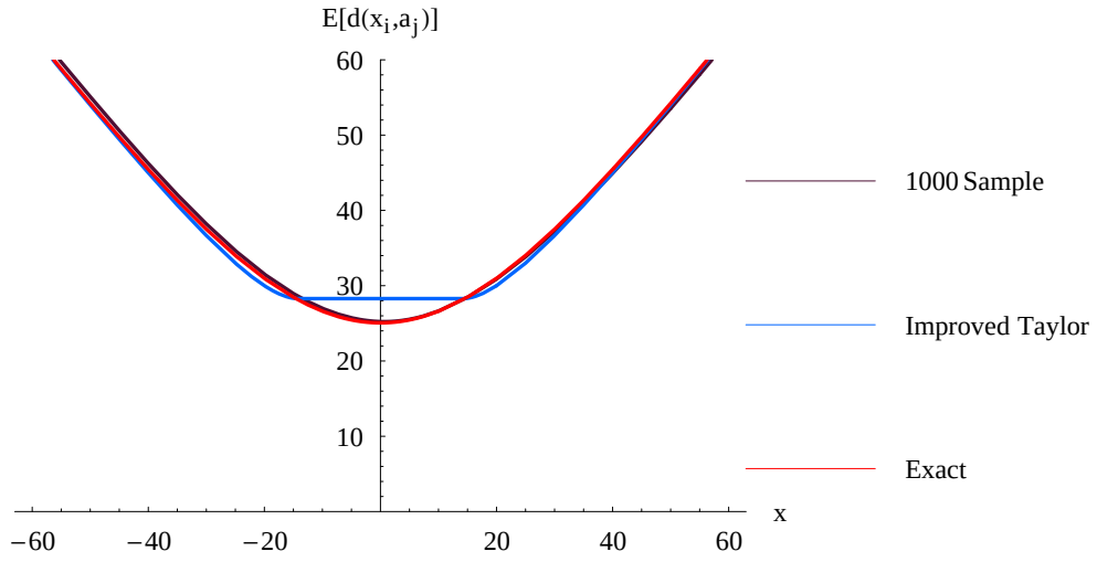
Figure 6.2. Improving Taylor approximation
