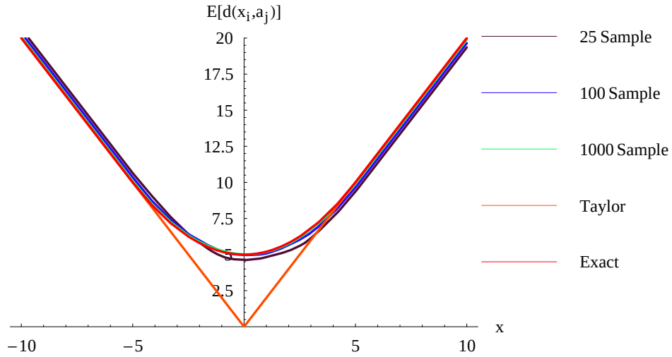
Figure 6.6. Sensitivity to sample size for symmetric distributions: Average distance vs Taylor approximation with estimated parameters
