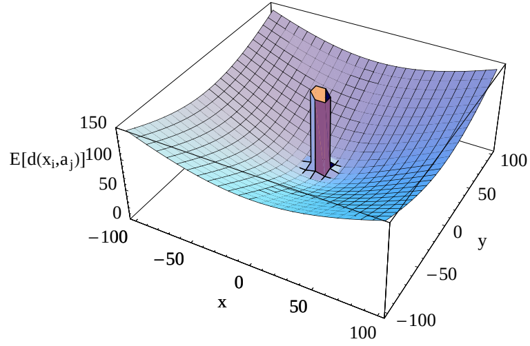
Figure 4.3. Overlapping graph of the exact expected distances and the Taylor Approximation for the Euclidean distance
