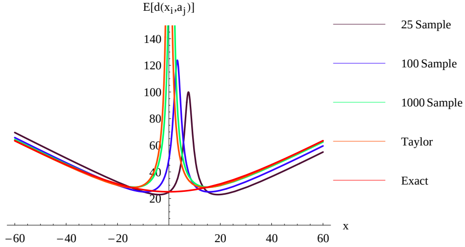
Figure 6.3. Sensitivity to sample size for symmetric distributions: Average distance vs Taylor approximation with estimated distribution parameters for the Euclidean norm
