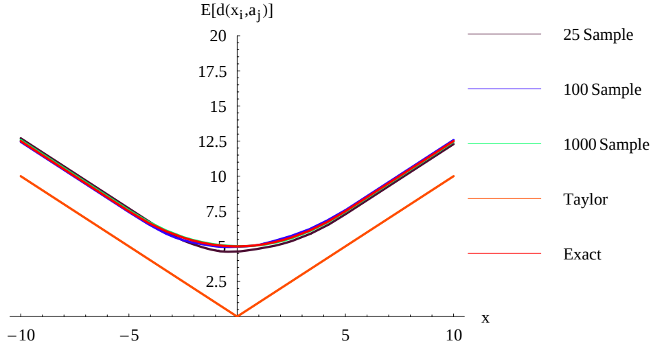
Figure 6.5. Sensitivity to sample size for symmetric distributions: Average distance vs Taylor approximation for the rectilinear norm
