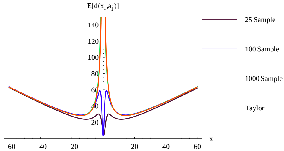
Figure 6.4. Sensitivity to sample size for asymmetric distributions: Taylor approximation with exact and estimated parameters for the Euclidean norm
