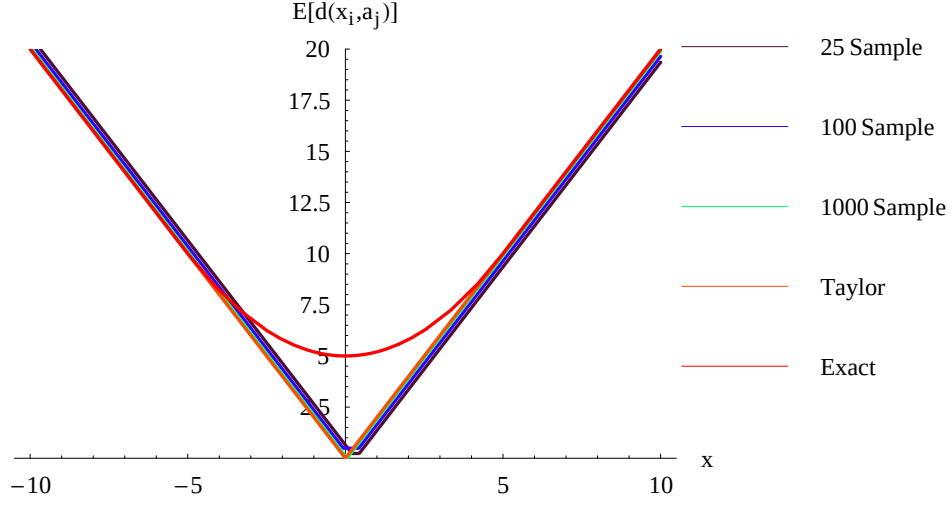
Figure 6.8. Sensitivity to sample size for symmetric distributions: Taylor approximations with exact and estimated distribution parameters
