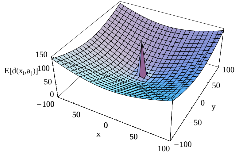
Figure 4.1. Taylor Approximation for Euclidean distance
