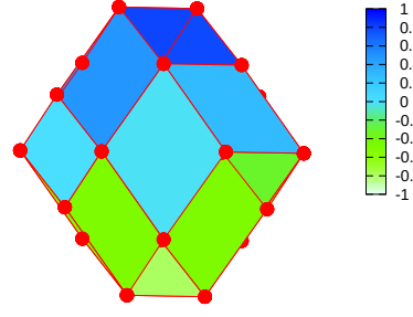
Figure 3.3. Rotated view perpendicular to a 2-fold axis of the rhombic-icosahedron
