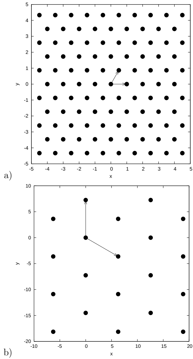
Figure 2.2. A a) triangular lattice, and b) its dual lattice
