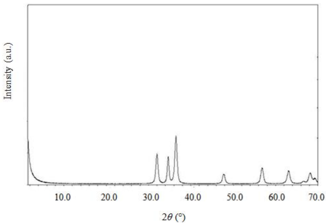
Figure 4.28. XRD pattern of 0.25M ZnO
