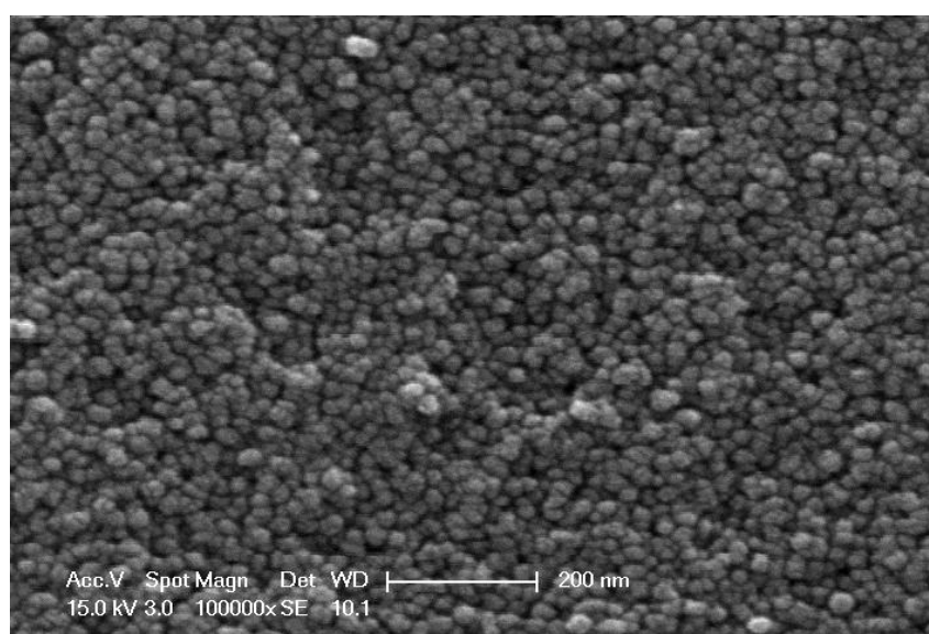
Figure 4.3. SEM image of 25% TiO 2 .
