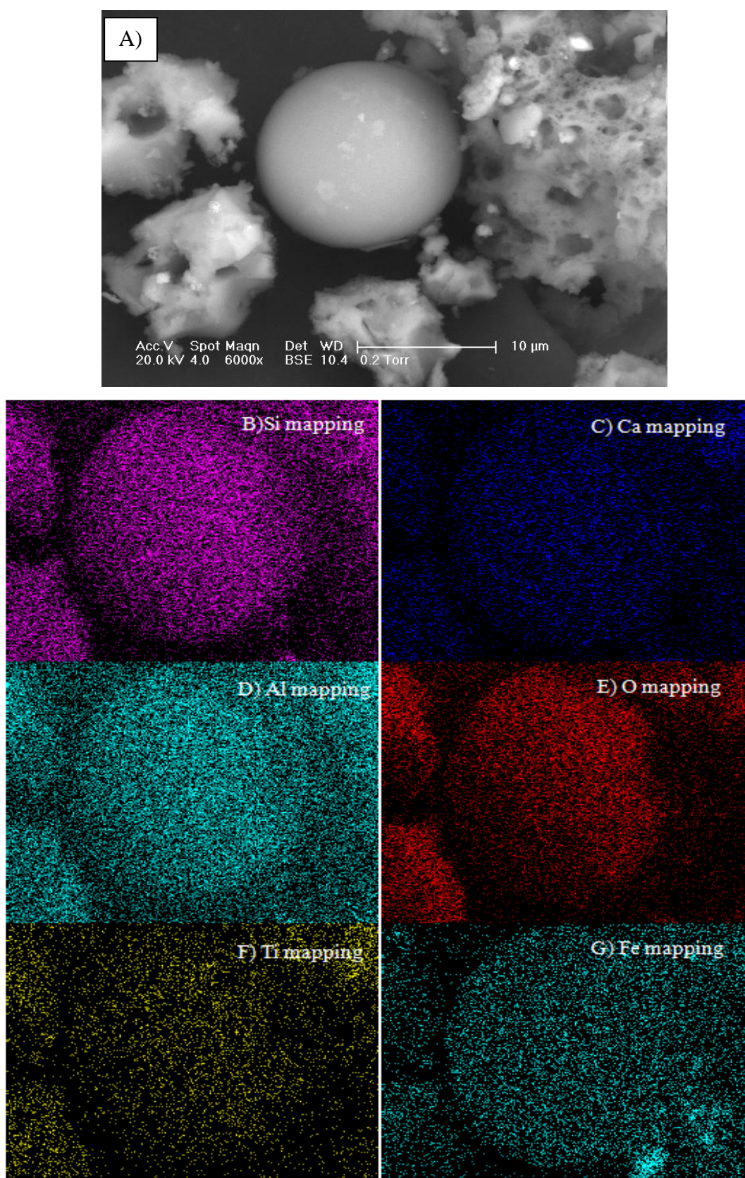
Figure 4.5. SEM and mapping images of 40% \text{TiO}_2 -FA (A), Si, Ca, Al, O, Ti and Fe (B-G).
