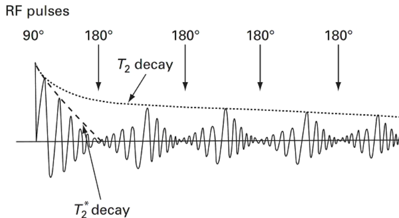
Figure 2.8 A spin echo pulse sequence, comprising a 90^\circ pulse followed by carefully timed 180^\circ pulses produces a series of spin echoes of decreasing amplitudes. Although each individual echo decays as T_2^* , the envelope decays as T_2 . Reproduced from [1].
