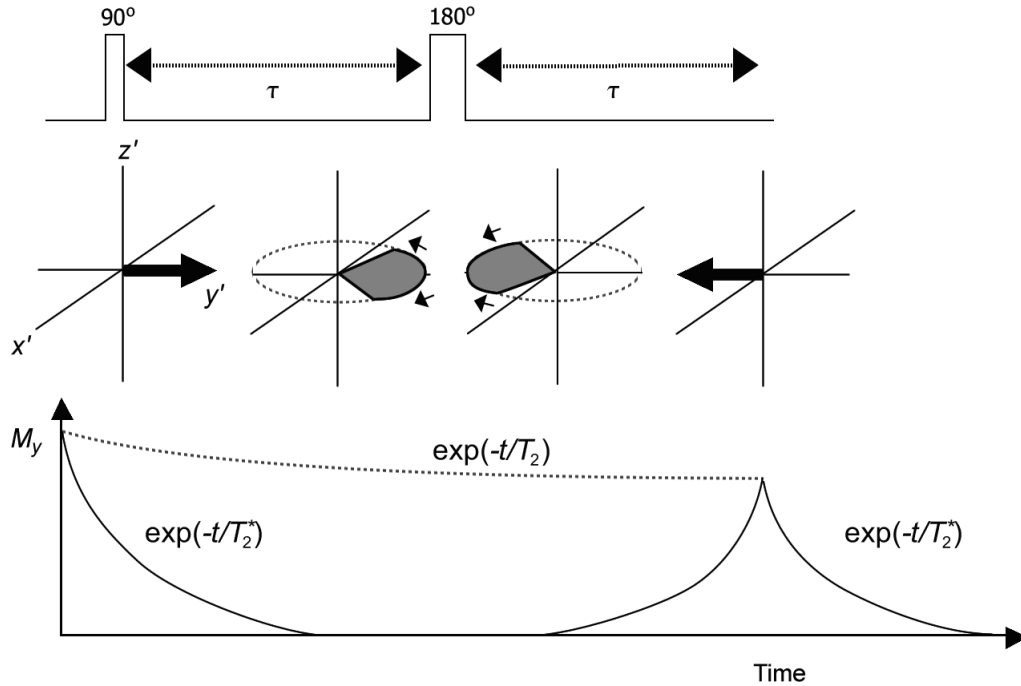
Figure 2.7 The 90^\circ pulse tips the magnetization into the x-y plane; after it finishes, de-phasing begins; the 180^\circ pulse flips the individual spins by 180^\circ in the x-y plane, so that they start moving into phase again. Reproduced from [1].
