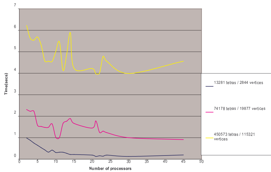
Figure 5.10. Overall Time
