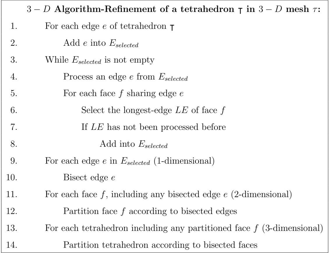
Figure 2.9. 3-D Refinement Algorithm
