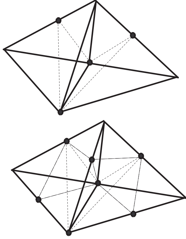
Figure 2.8. 4-Tetrahedra and 8-Tetrahedra
