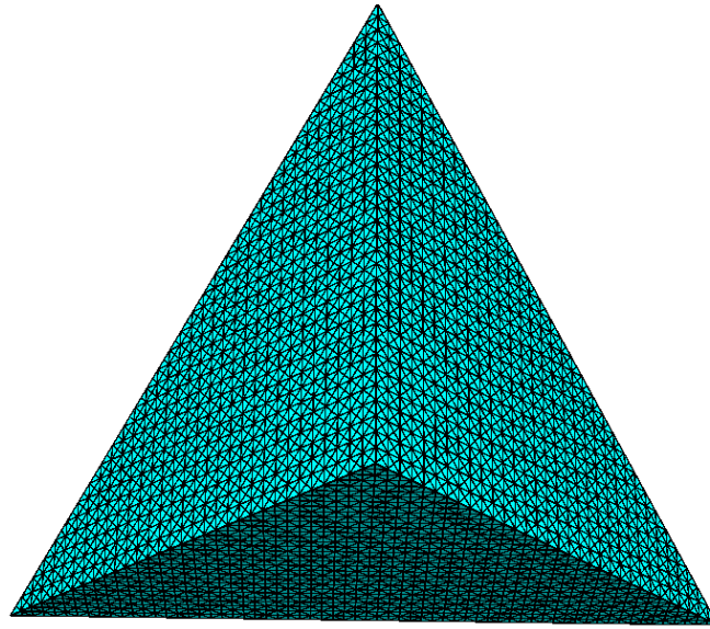
Figure 5.5. 99121 tetrahedra / 23351 vertices
