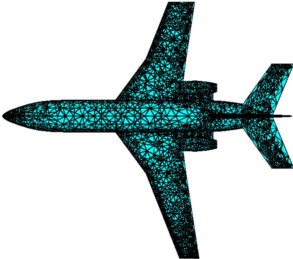
Figure 5.7. 79263 tetrahedra / 33098 vertices
