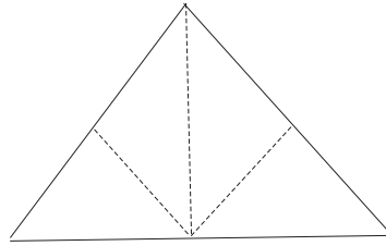
Figure 2.4. 4T\text{-}LE Refinement
