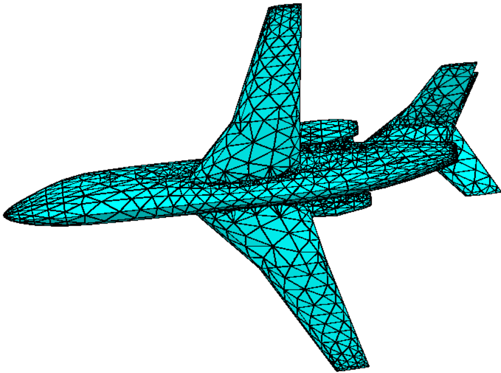
Figure 5.4. 12586 tetrahedra / 3644 vertices
