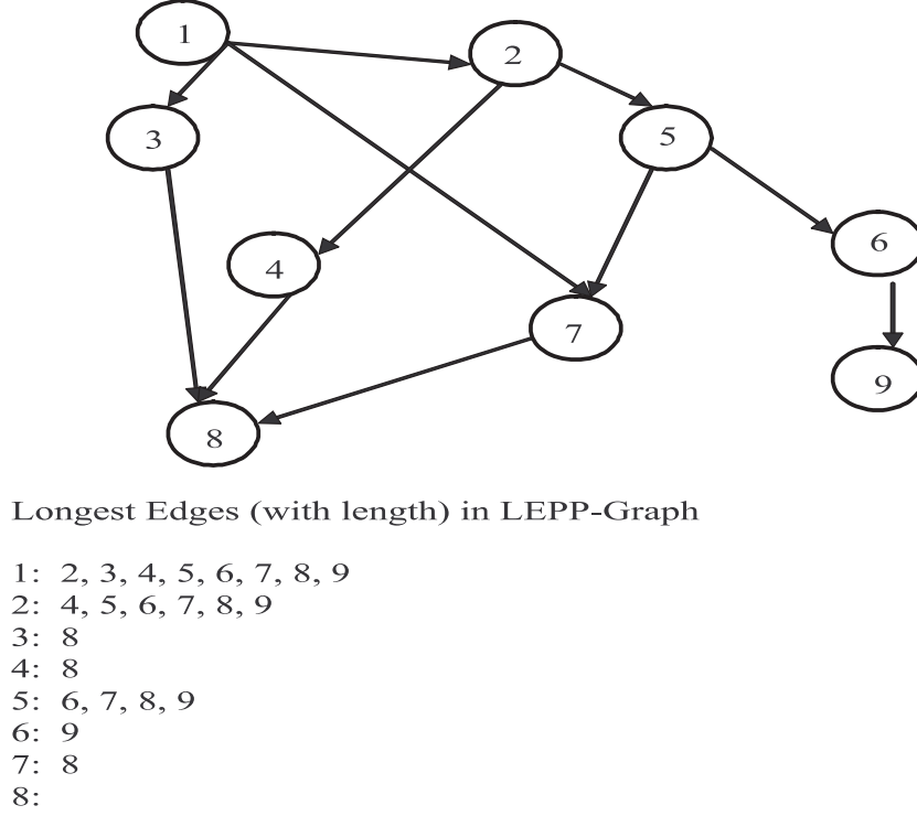
Figure 3.1. LEPP -Graph
