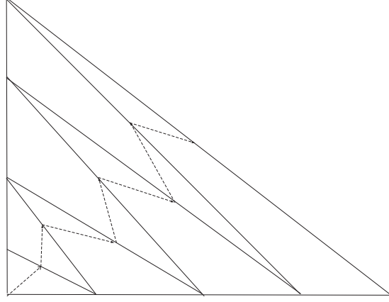
Figure 2.3. Longest-Edge Propagation
