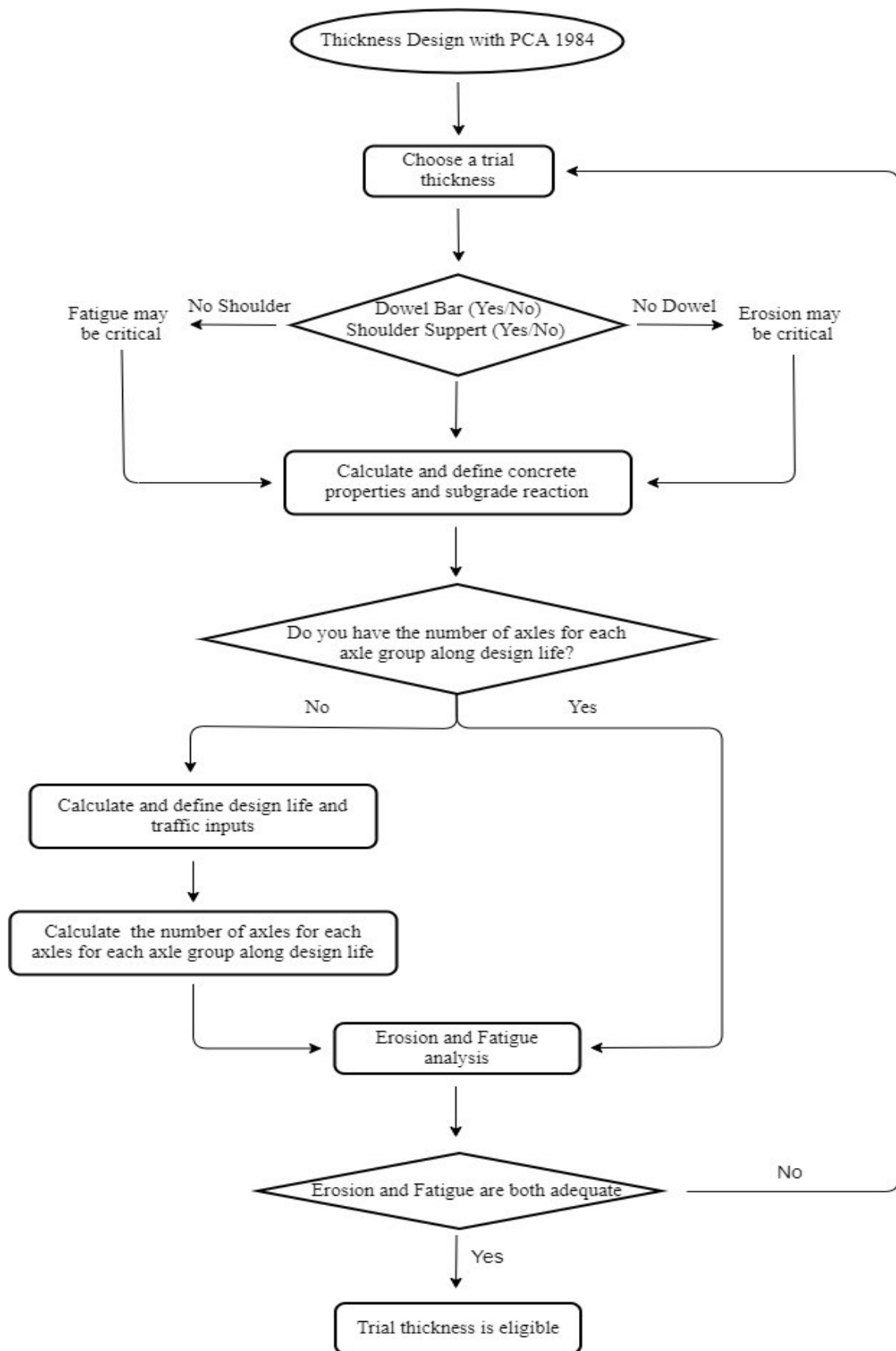
Figure 3.3. PCA (1984) flow chart (Kııcı and Tıgdemir, 2017).
