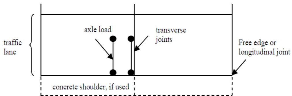
Figure 2.19. Most critical loading position for erosion failure (Huang, 2004).
