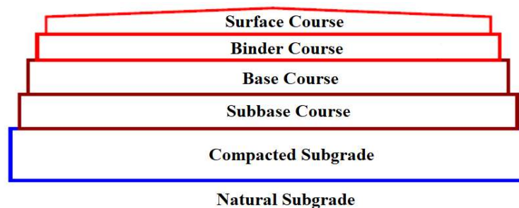
Figure 2.2. Typical cross-section of a flexible pavement (Huang, 2004).
