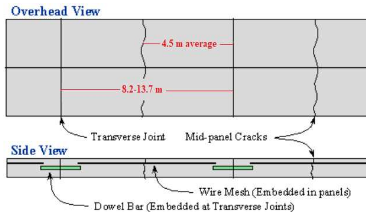
Figure 2.5. Jointed reinforced concrete pavement (Huang, 2004).
