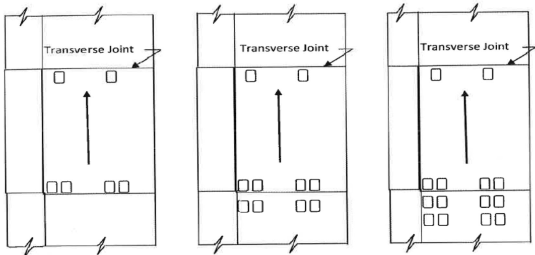
Figure 2.15. Different axle load positions causing tensile stress at the top fiber of the slab with tied concrete shoulder (IRC 58, 2015).
