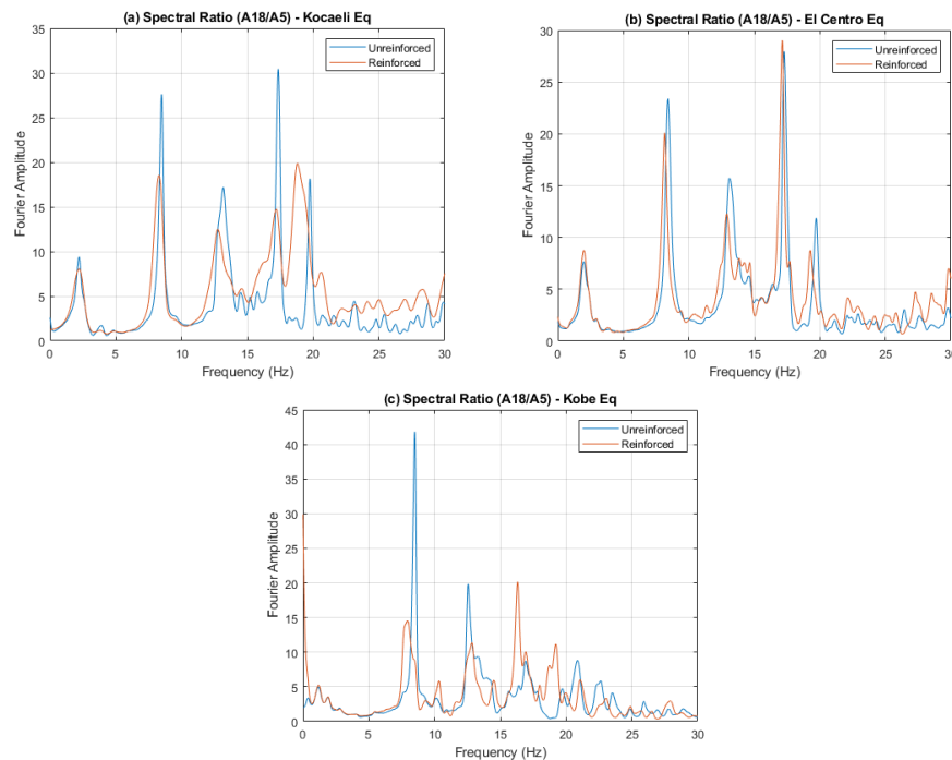
Figure 5.9. Spectral Ratio Comparisons for Case 1 – Kocaeli Earthquake (a), El Centro Earthquake (b), Kobe Earthquake (c).
