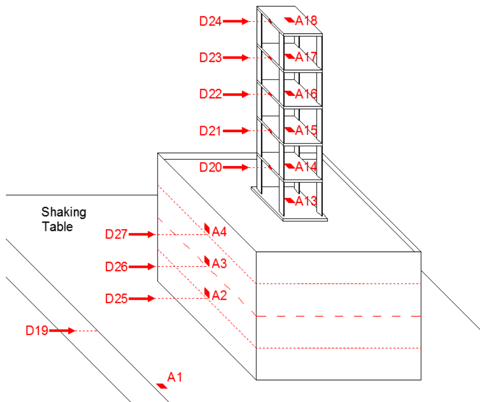
Figure 3.19. A sketch of test setup for the geogrid reinforced soil system for the 5-story model.
