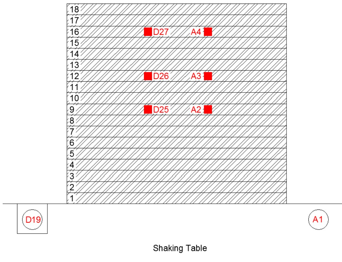
Figure 3.7. A sketch of instrumentation layout of laminar box without soil – Front view.
