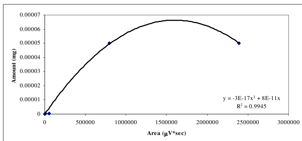
Figure A.2. Calibration curve for C2-Cer
