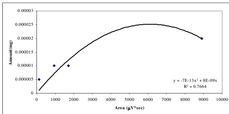
Figure A.5. Calibration curve for C18-DHS
