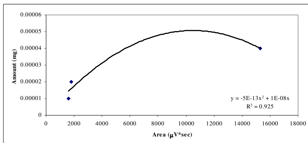
Figure A.3. Calibration curve for P-Cer
