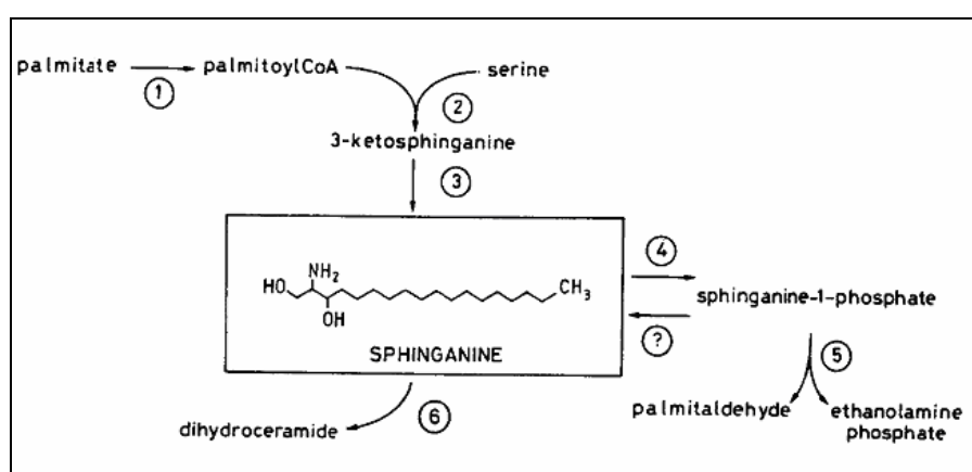
Figure 4.4. Sphinganine metabolism
