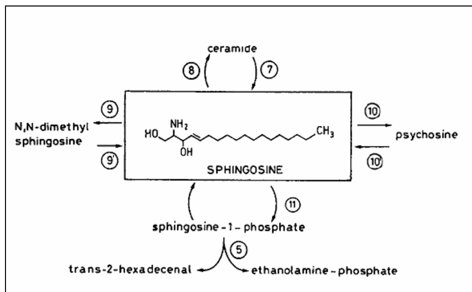
Figure 4.5. Sphingosine metabolism
