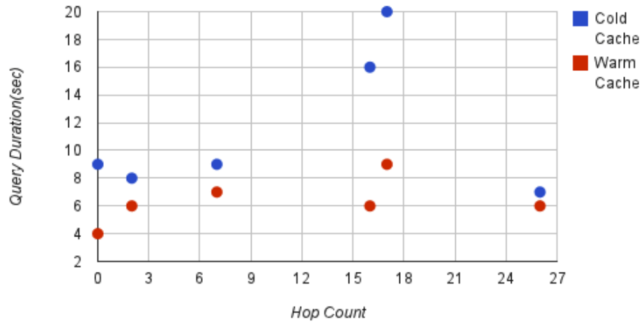
Figure 4.5. APWEP 3 depth query performance results with extra traffic.
