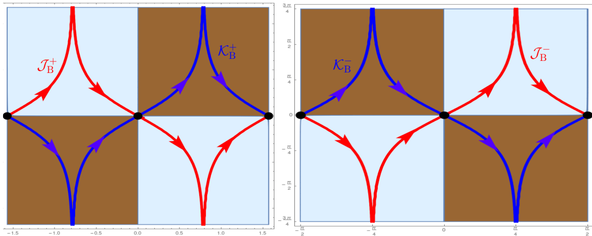
Figure 4.4. Lefschetz thimbles for the magnetic case.
