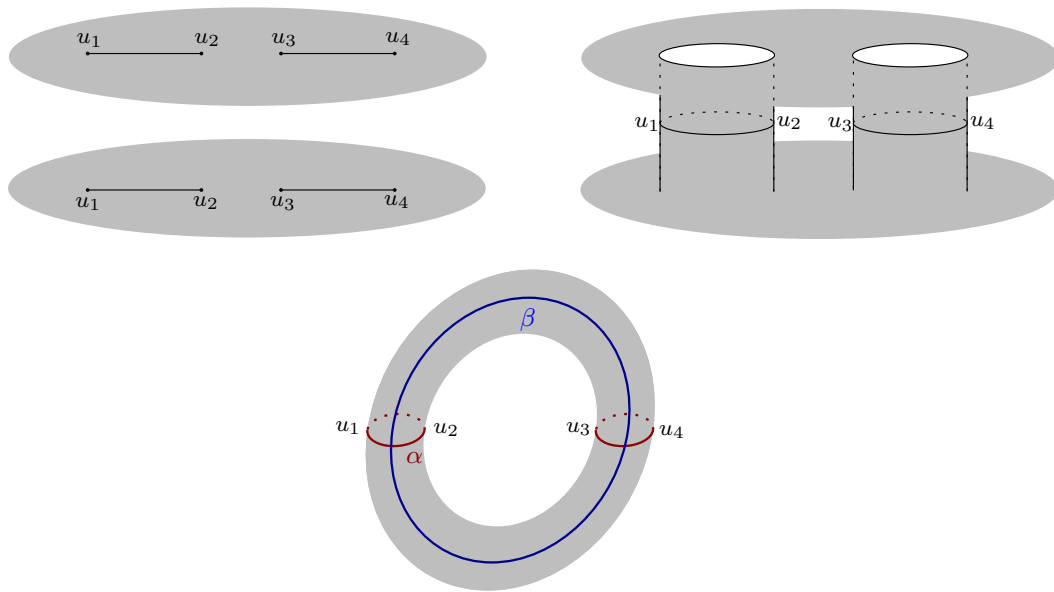
Figure 2.6. Formation of torus from a two sheeted Riemann surface.
