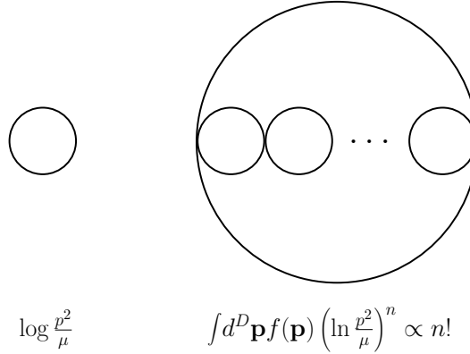
Figure 2.1. Left: A renormalized 1-loop diagram with logarithmic momentum dependence. Right: n renormalized diagram inserted in a larger loop.
