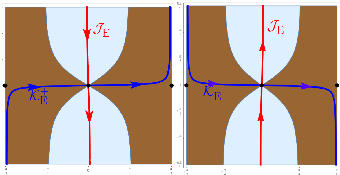
Figure 4.5. Lefschetz thimbles for the electric case.
