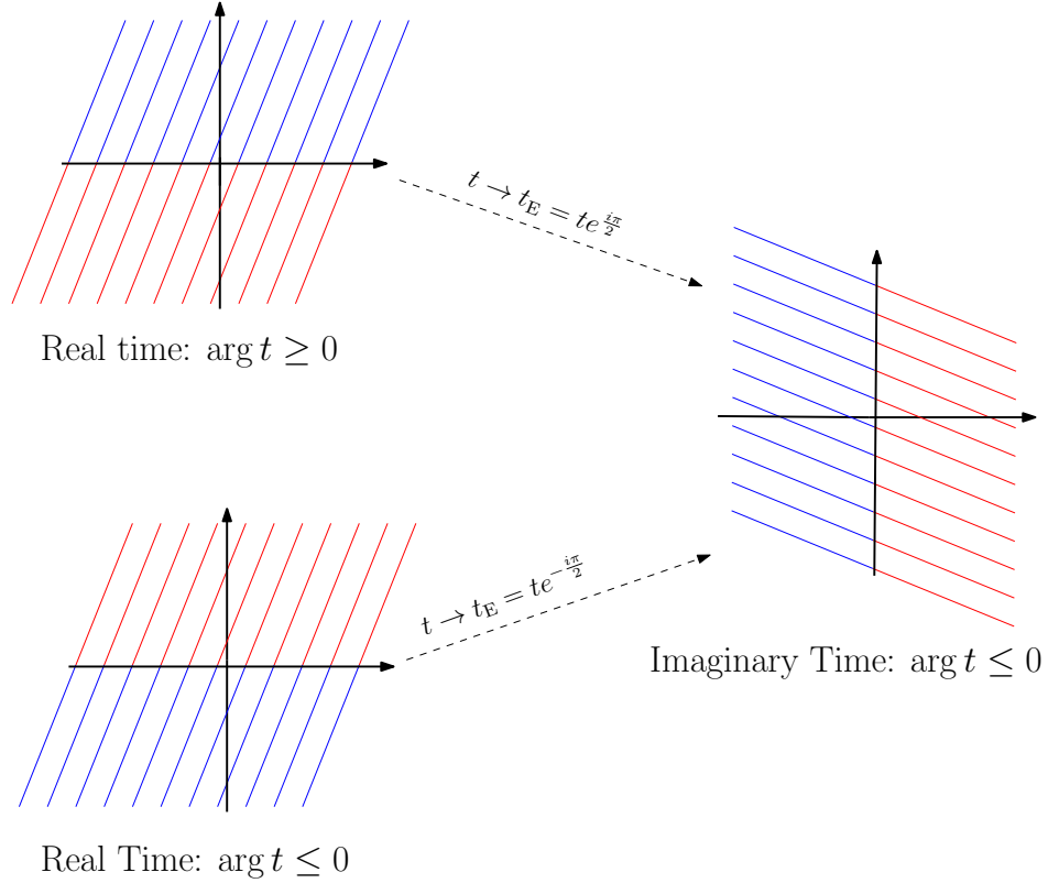
Figure 4.1. Complex t planes. (Left) Real time cases. (Right) Imaginary time case.
