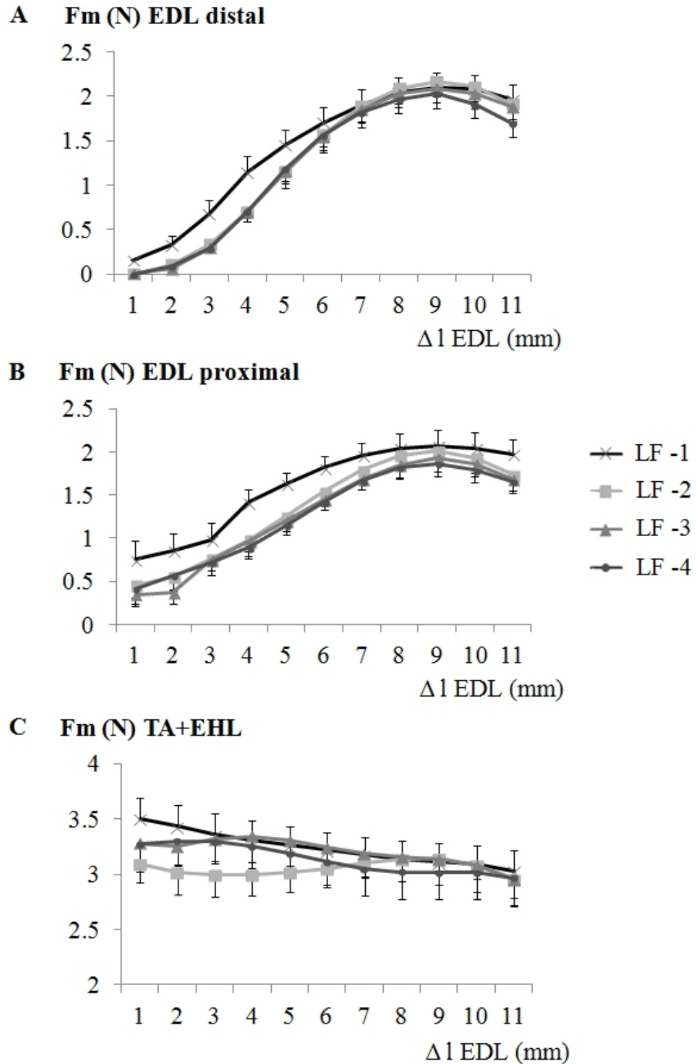
Figure A.2 Force-length characteristics of (a) EDL distal, (b) EDL proximal, and (c) TA+EHL muscles obtained after distal lengthening. Total isometric forces are shown as mean values \pm SD for FL1, FL2, FL3, and FL4 conditions. Muscle-tendon complex length is expressed as a deviation from EDL optimum length ( \Delta l EDL=10mm) at FL1.
