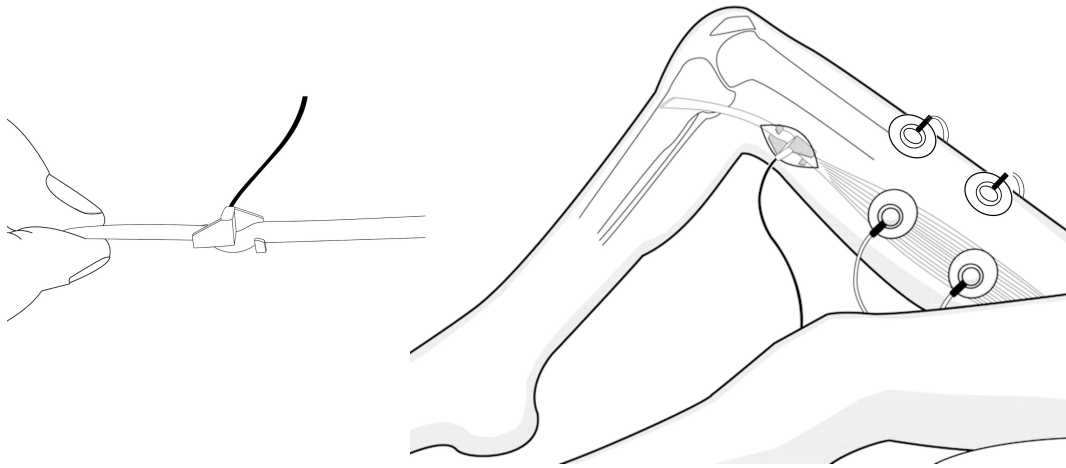
Figure 4.1 Usage of buckle force transducer and stimulation electrodes. Illustrations of how (A) the buckle force transducer is mounted over tendon strips, and (B) the skin electrodes are mounted over the GRA and VM muscles are shown.
