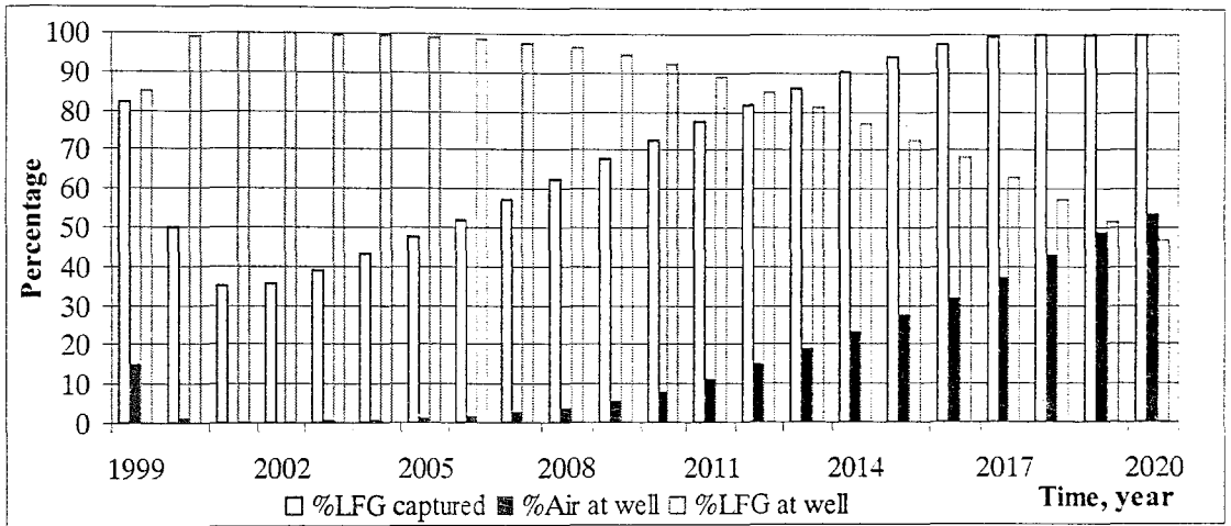
Figure 5.12. LFG and air percentages for Case 6
