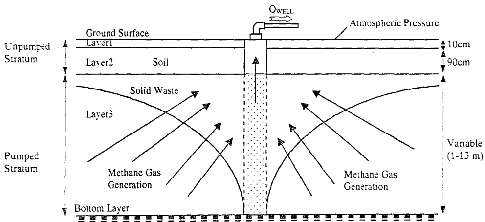
Figure 4.4. Model cross section of the extraction wells for gas flow model
