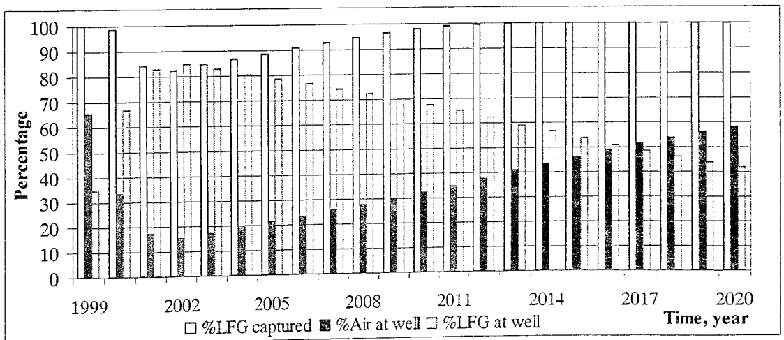
Figure 5.7. LFG and air percentages for Case 3
