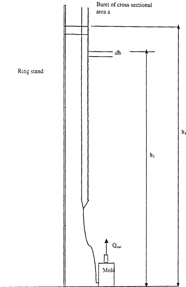
Figure 4.3. Line details of the falling head test equipment
