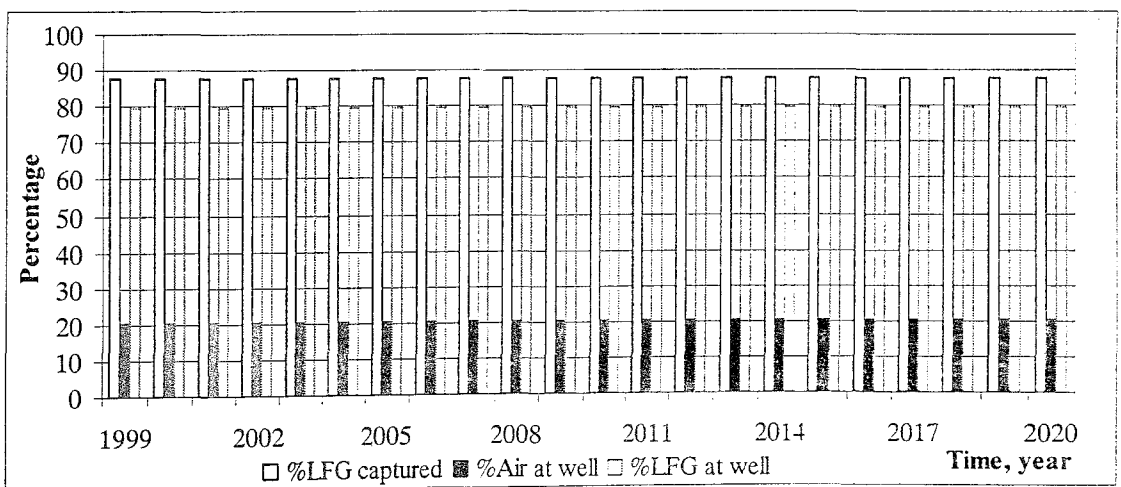
Figure 5.11. LFG and air percentages for Case 5
