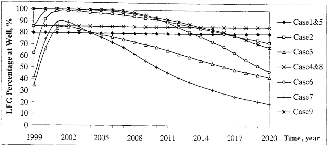
Figure 5.18. LFG percentages at wells (comparison for all cases)
