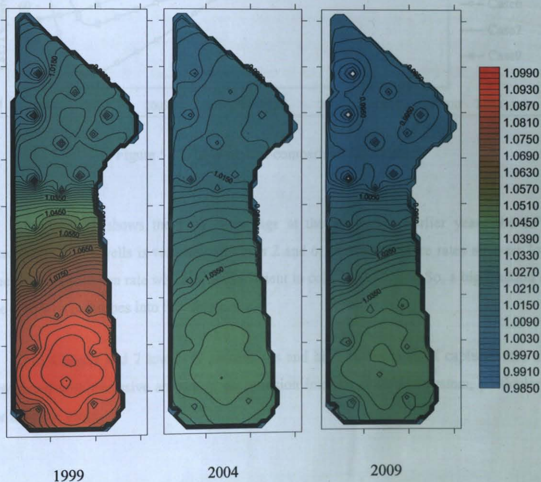
Figure 5.16. Pressure distribution (in atm) for years 1999, 2004 and 2009 of Case 9
