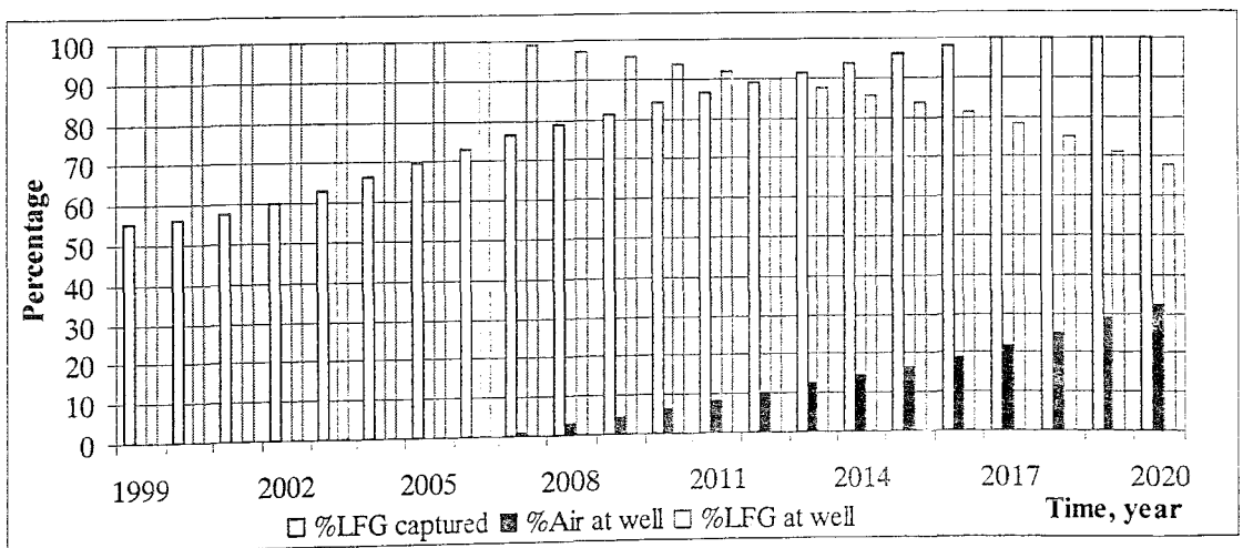
Figure 5.15. LFG and air percentages for Case 9
