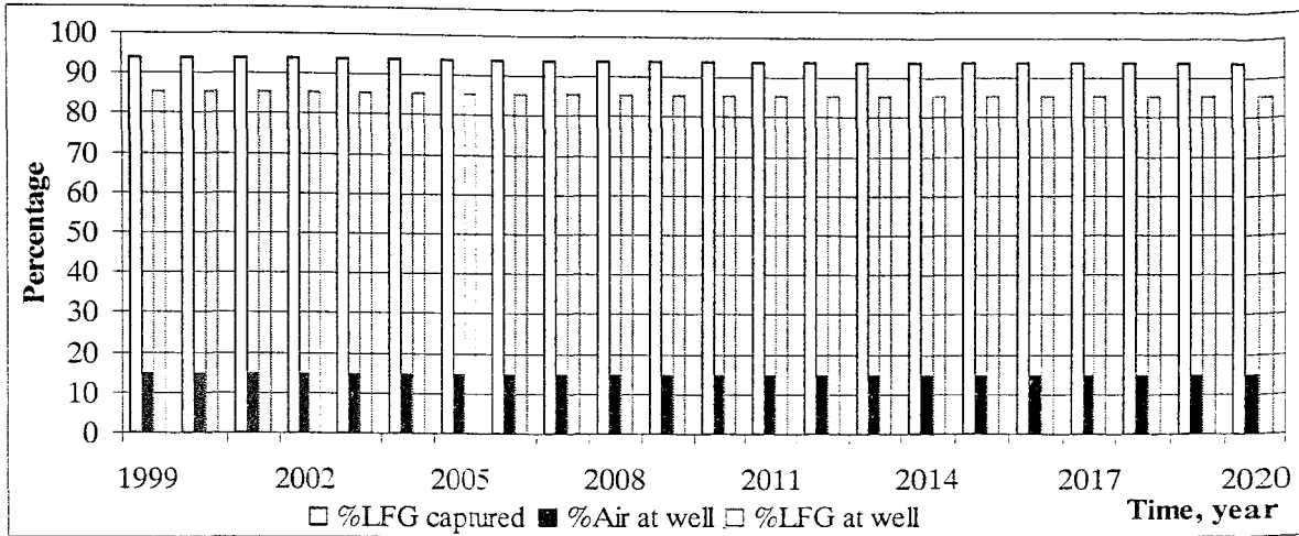
Figure 5.14. LFG and air percentages for Case 8
