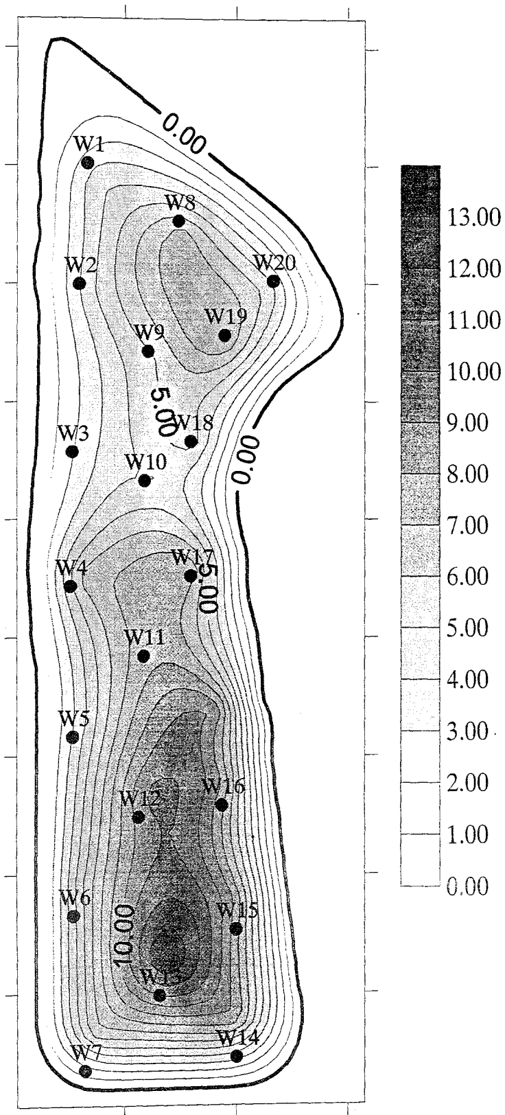
Figure 4.6. Contour plot of the waste thickness in meters used in the gas flow model
