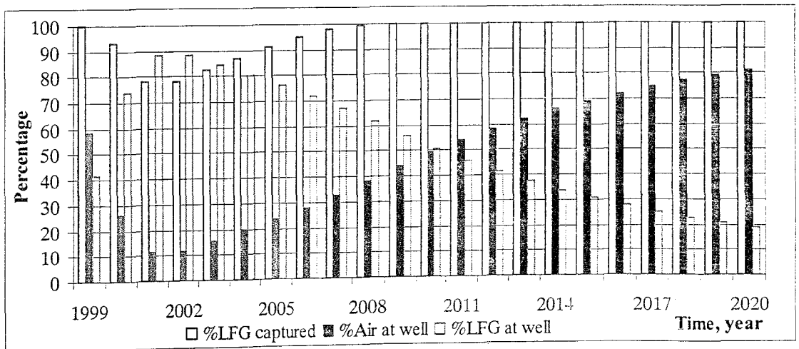
Figure 5.13. LFG and air percentages for Case 7
