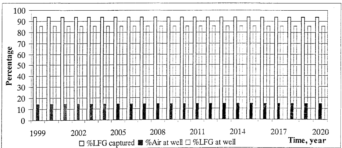
Figure 5.10. LFG and air percentages for Case 4
