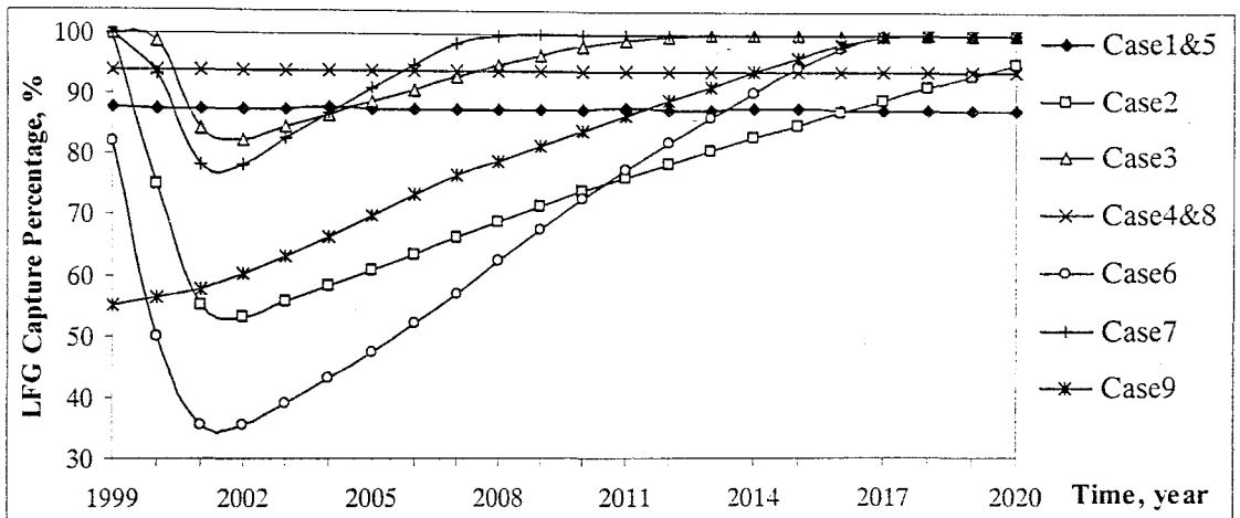
Figure 5.17. LFG capture comparison for all cases
