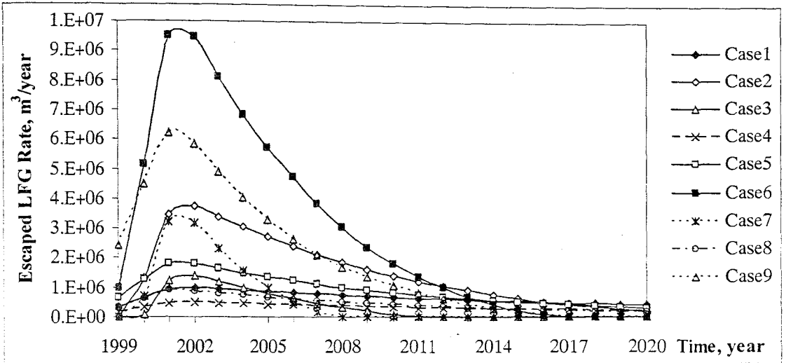
Figure 5.21. Escaped LFG rates (comparison for all the cases)
