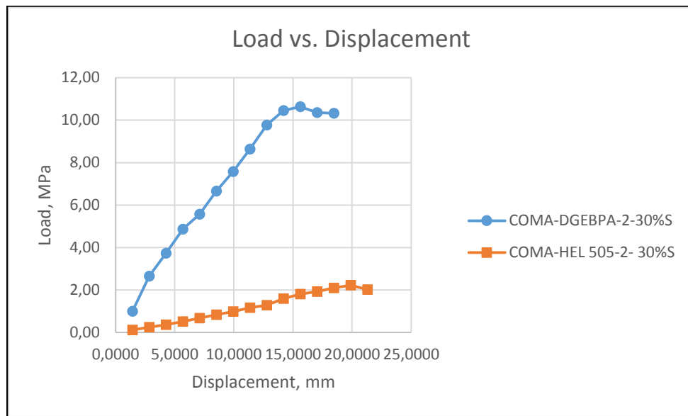
Figure 4.24. Load vs. Displacement Curve of Second Networks.
