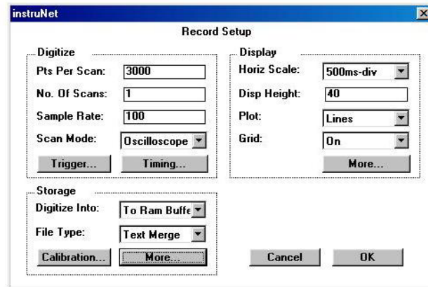
Figure 4.6a Instrunet Setup-1
