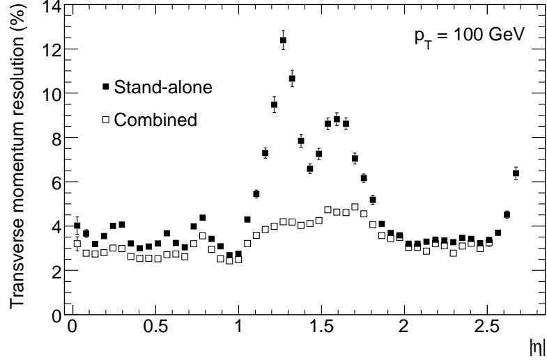
Figure 4.1. For muons with p_T = 100 \text{ GeV}/c , expected fractional momentum resolution as a function of |\eta| for stand-alone and combined reconstruction [28].
