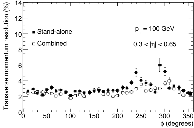
Figure 4.2. For muons with p_T = 100 \text{ GeV}/c , expected fractional momentum resolution as a function of \phi for stand-alone and combined reconstruction [28].
