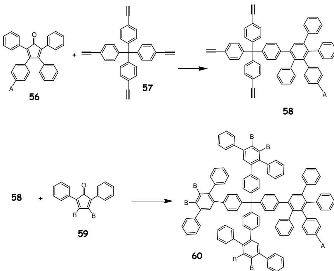
Figure 2.14. 'Desymmetrized' dendrimers
