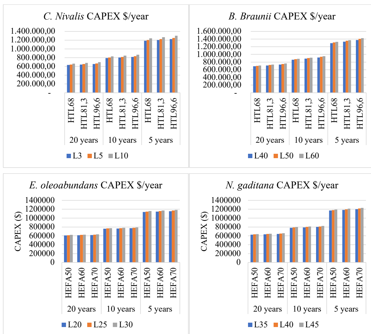
Figure 4.11. Capital expenditures of C. nivalis , B. braunii , E. oleoabundans and N. gaditana with respect to lipid content, conversion rate and installment plan.
