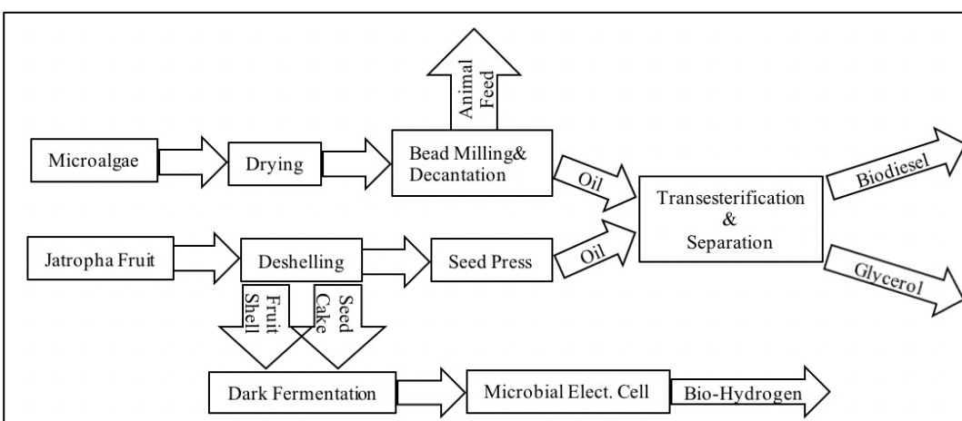
Figure 2.6. Flow diagram of Scenario 3 (adopted from Giwa et al., 2018).
