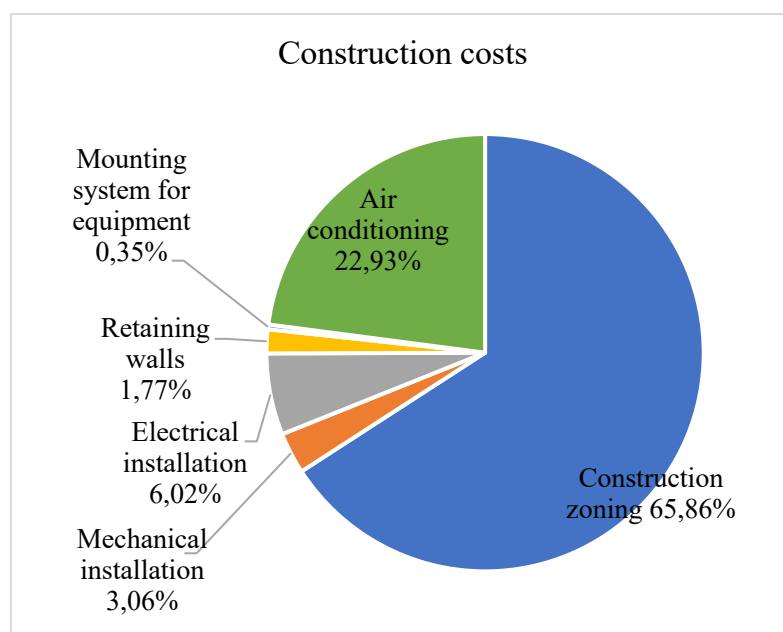
Figure 4.5. Contributors to capital cost of construction.
