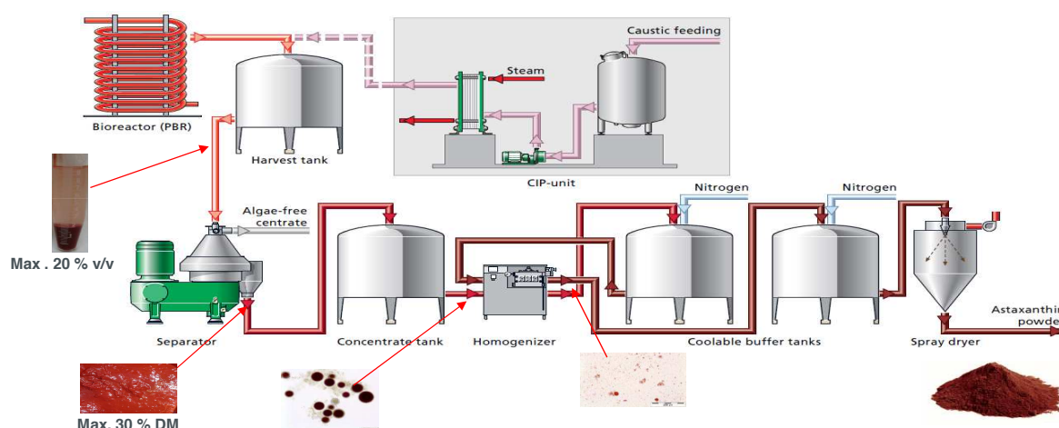
Figure 4.16. Process flow for Astaxanthin powder from PBR at IMBIYOTAB.
