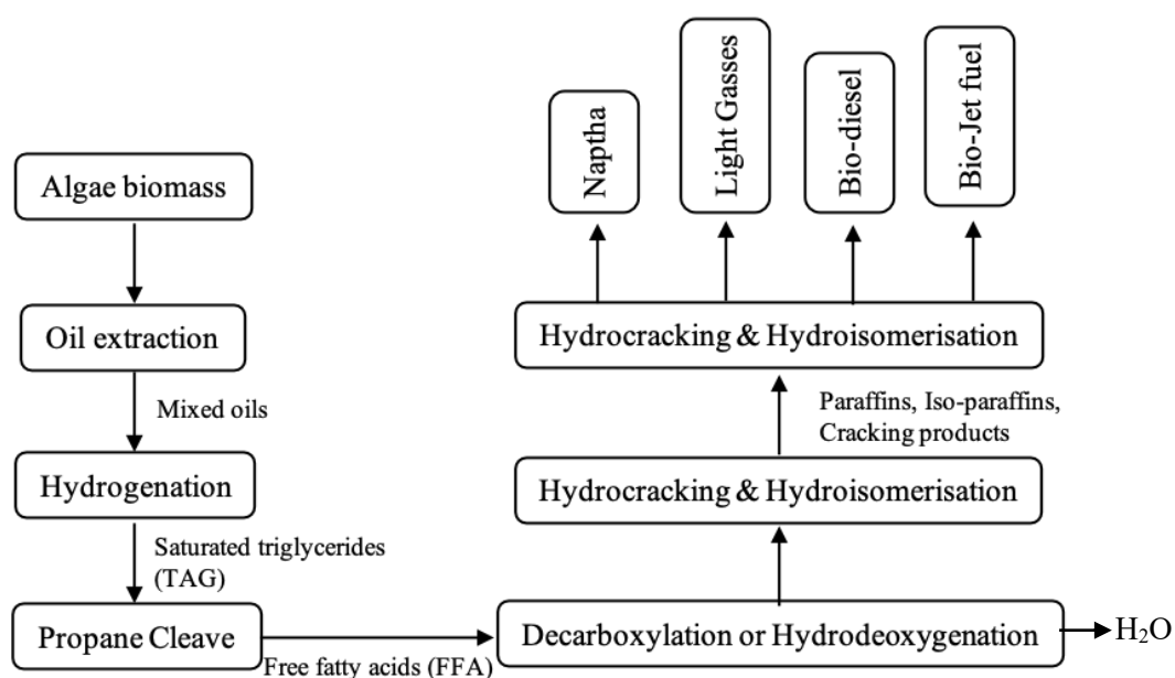
Figure 4.3. Process flow diagram of HEFA technology (adopted from Wang and Tao, 2016).
