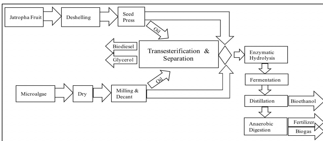
Figure 2.5. Flow diagram of Scenario 2 (adopted from Giwa et al., 2018).
