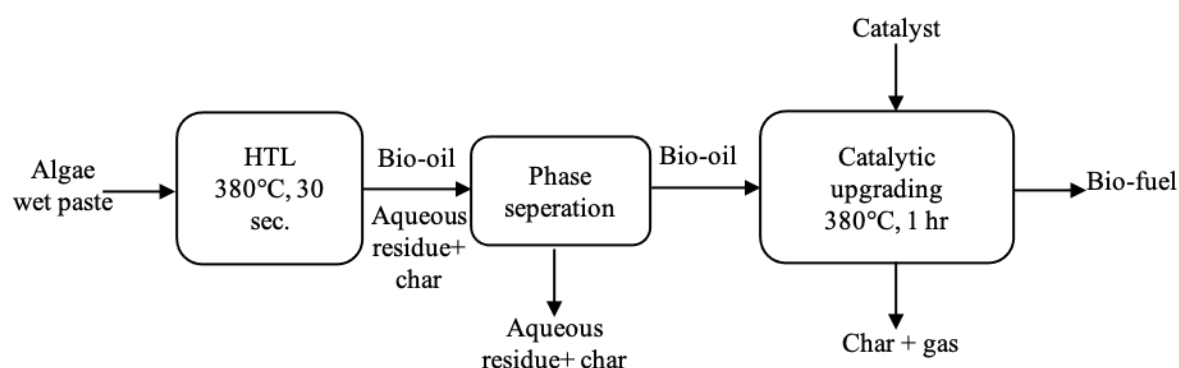
Figure 4.2. HTL process flow diagram.
