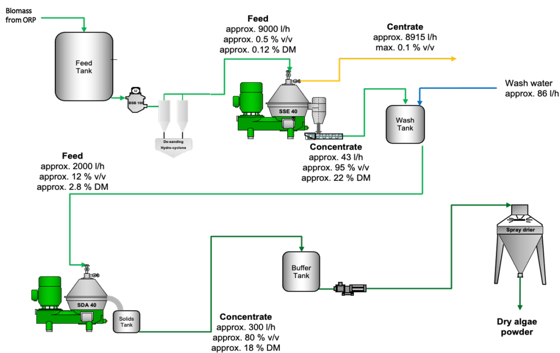
Figure 1.7. Algae processing in open raceway pond (ORP) system at IMBIYOTAB.
