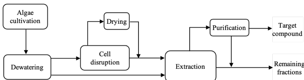
Figure 1.9. General process flow diagram of an algae extraction process (adopted from Bastiaens et al., 2017).
