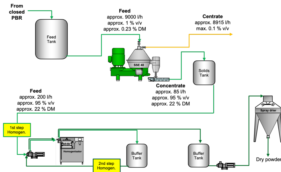
Figure 1.8. Algae processing closed photo-bio-reactor (PBR) at IMBIYOTAB.
