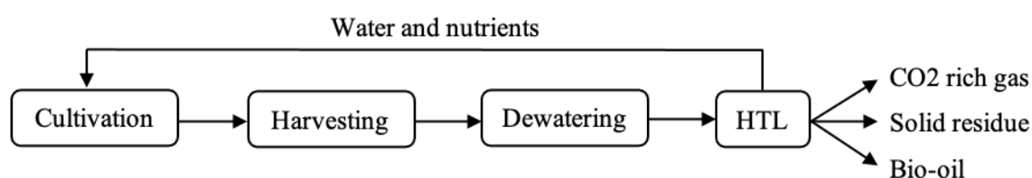
Figure 4.1. Conceptual scheme of HTL in an algae biorefinery.
