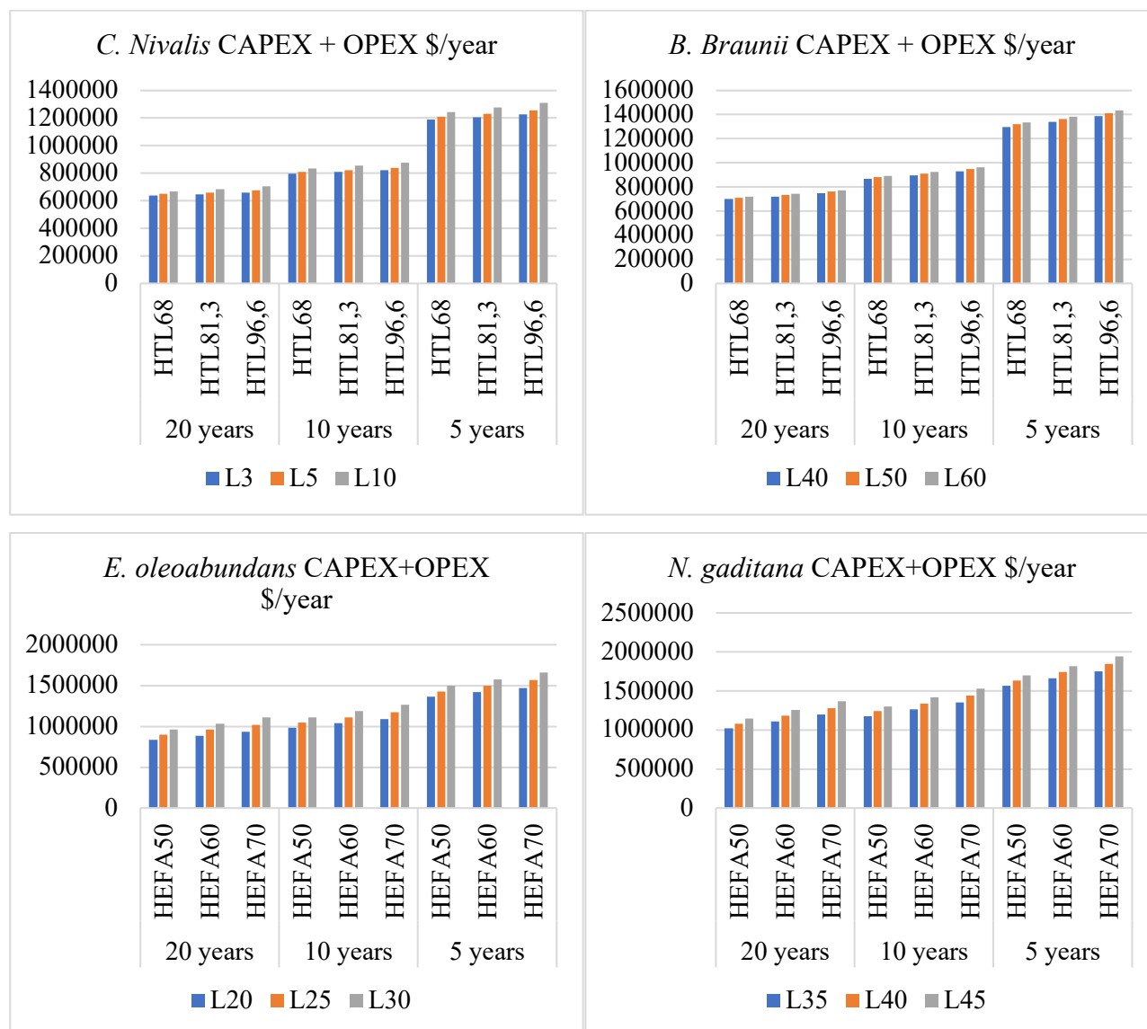
Figure 4.14. Annual production costs of each species with respect to lipid content, conversion efficiencies and installment plans.
