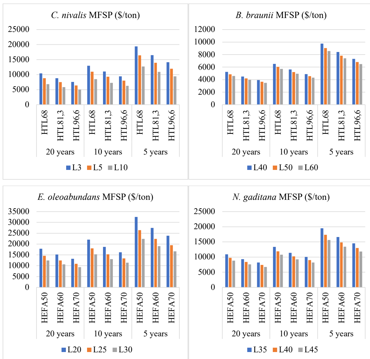
Figure 4.15. Minimum fuel selling prices of each species with respect to lipid content, conversion efficiencies and installment plans.
