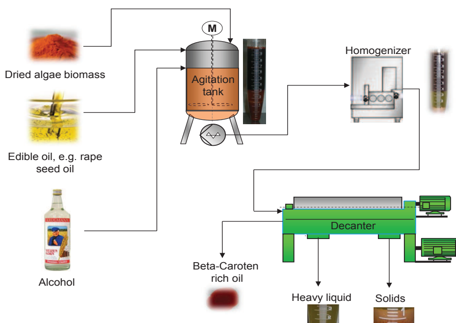
Figure 4.18. Process flow for beta-Carotene extraction at IMBIYOTAB.
