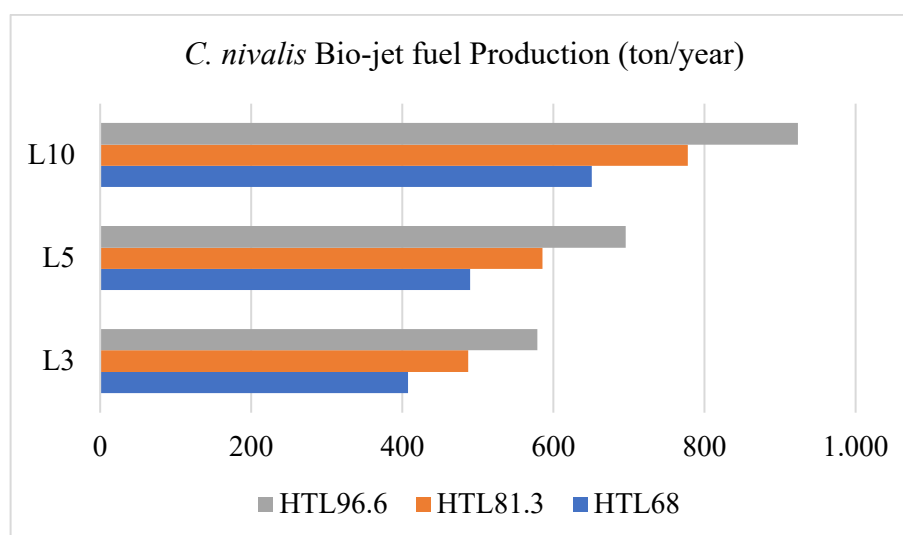
Figure 4.7. Bio-jet fuel production of C. nivalis with HTL technology with respect to different lipid and conversion rates.
