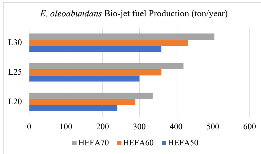
Figure 4.9. Bio-jet fuel production of E. oleoabundans with HTL technology with respect to different lipid and conversion rates.
