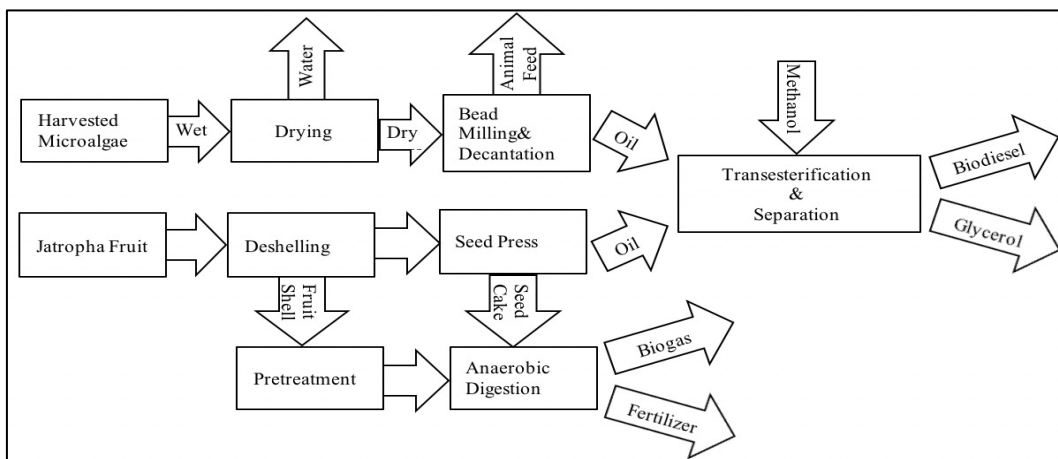
Figure 2.4. Flow diagram of Scenario 1 (adopted from Giwa et al., 2018).
