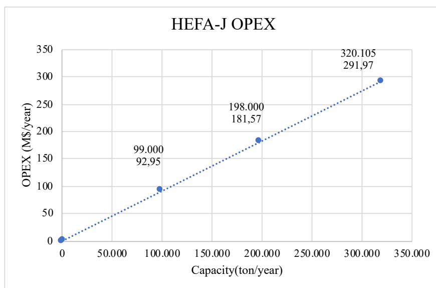
Figure 4.13. Operational HEFA expenses regarding annual production capacity.
