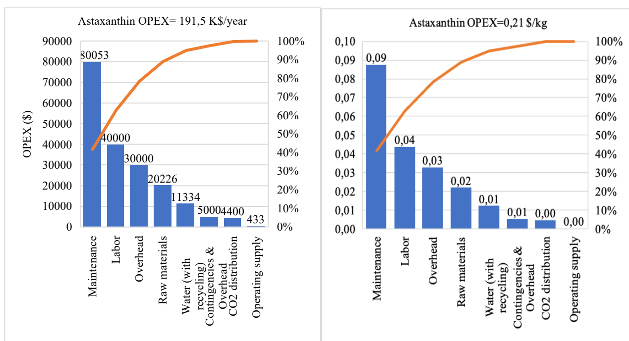
Figure 4.17. Major contributors to annual operational expenses and operational cost per kg astaxanthin.
