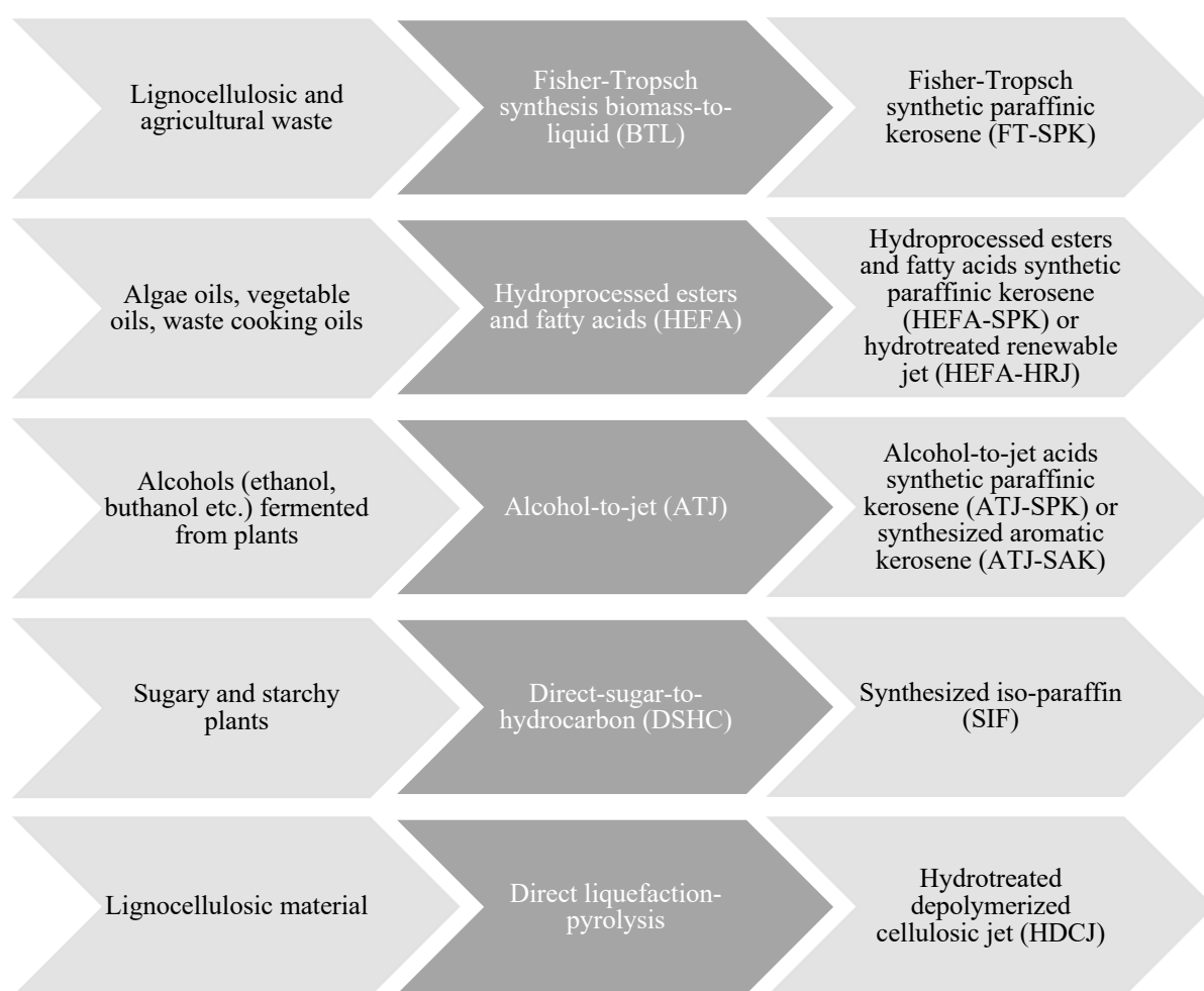
Figure 1.10. Conversion of biomasses to alternative biofuel by various technologies: Fisher-Tropsch biomass-to-liquid (BTL), hydrogenation (HEFA), alcohol-to-jet (ATJ), direct liquefaction-pyrolysis.
