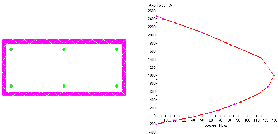
Figure 4.8. 55x25 column p-m relationship for 45°
