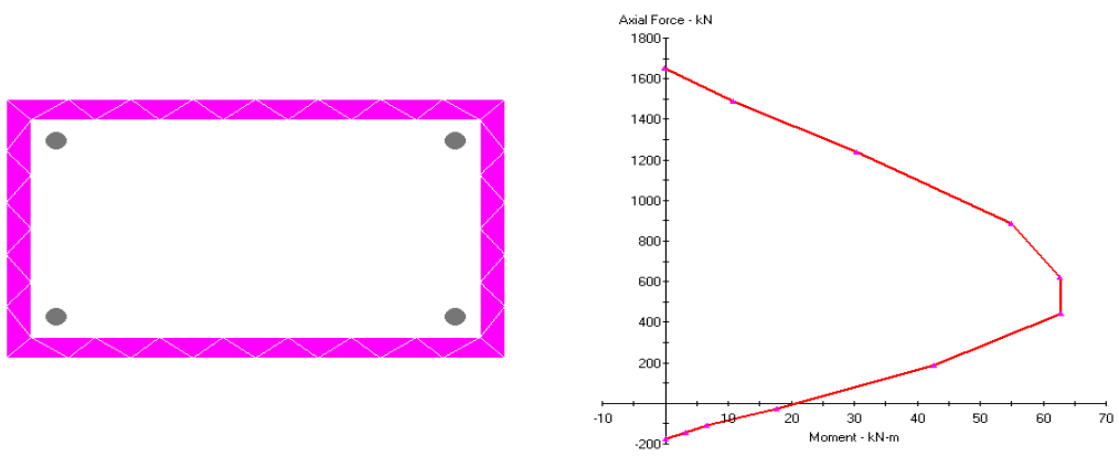
Figure 4.6. 40x25 column p-m relationship for 45°
