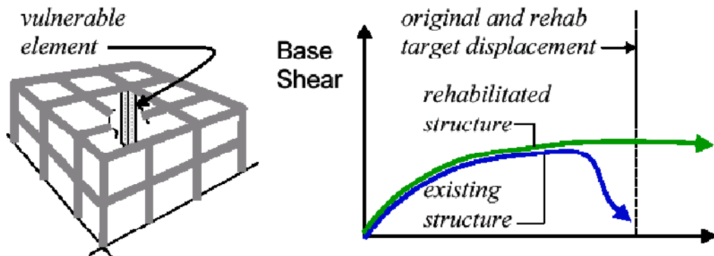
Figure 1.5. Local modification of the structural system
