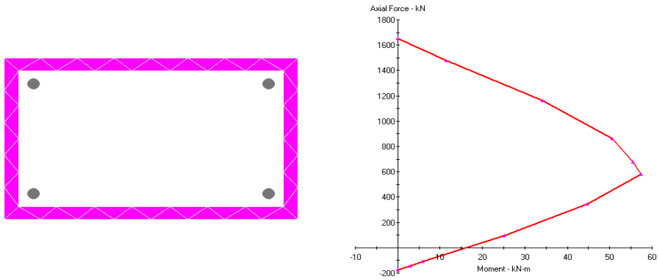
Figure 4.5. 40x25 column p-m relationship for 0°
