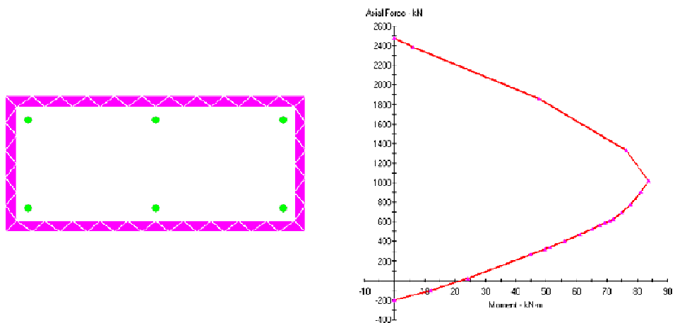
Figure 4.7. 55x25 column p-m relationship for 0°
