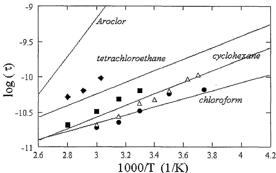
FIGURE 2.3. Comparison of experimental and simulation results for the correlation times of cis -PIP \text{CH}^a vectors in various solvents.
