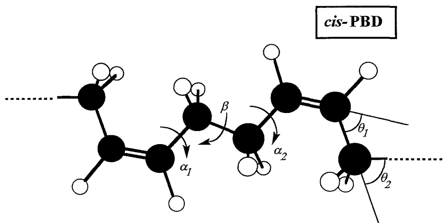
FIGURE 3.5. A segment of cis -PBD chain.
