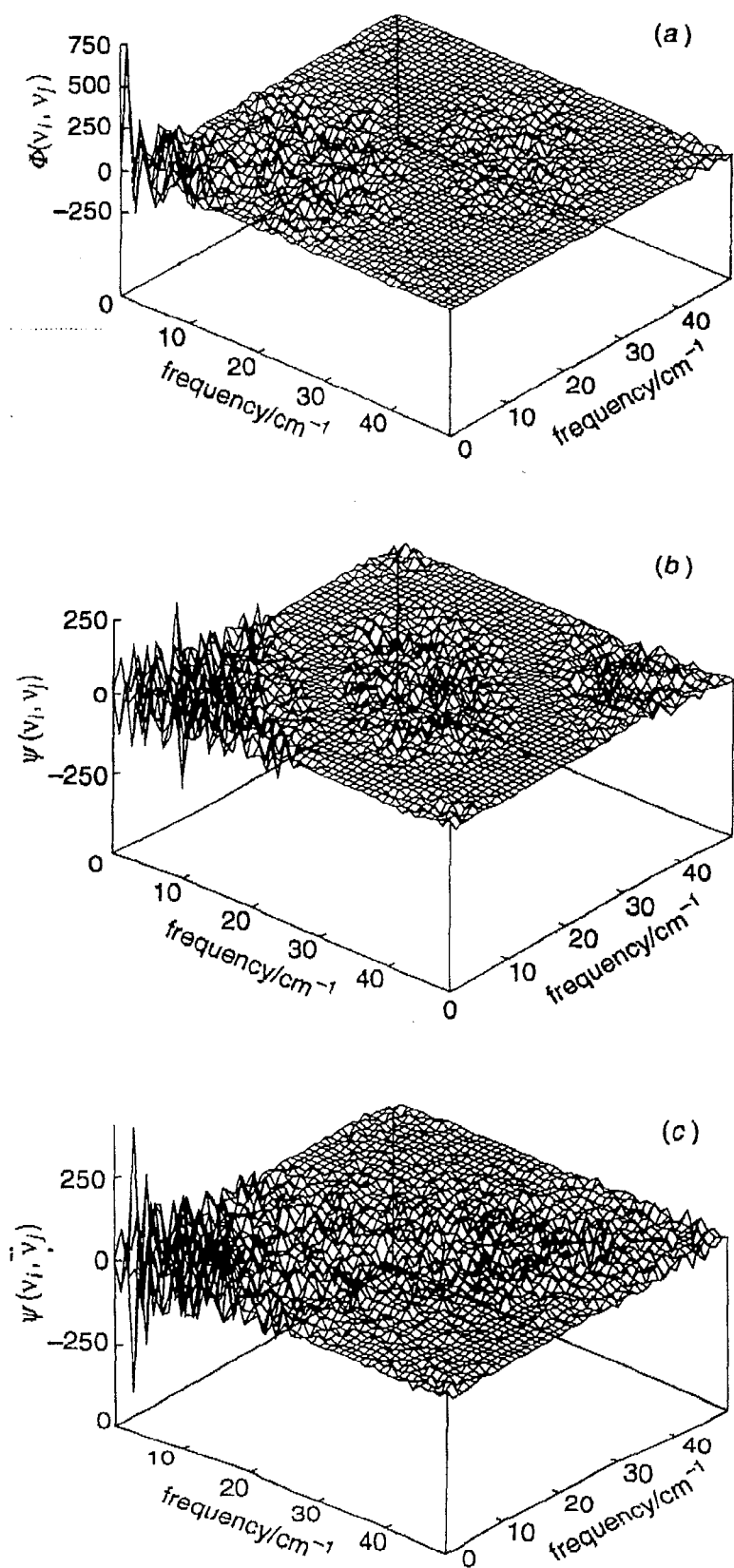
FIGURE 3.21. Symmetric and antisymmetric parts of the modal correlation matrix: (a) \Phi(v_i, v_j) , l=0 and \tau=1 ps; (b) \Psi(v_i, v_j) , l=0 and \tau=1 ps; (c) \Psi(v_i, v_j) , l=2 and \tau=1 ps;
