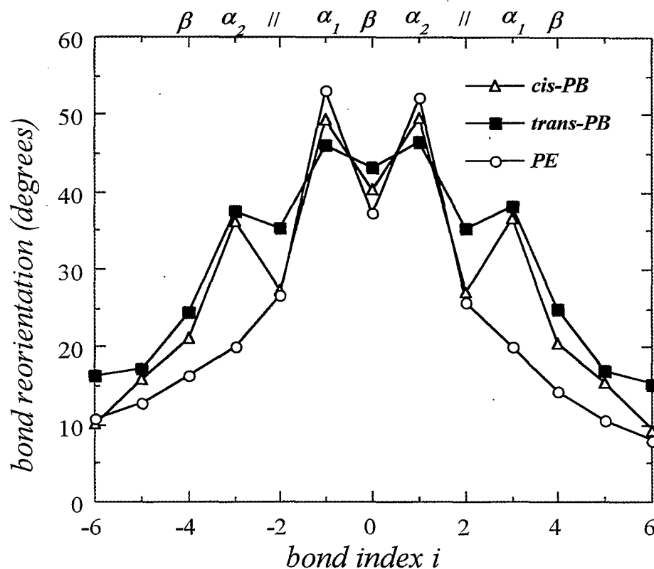
FIGURE 3.7. Average spatial reorientations of bond vectors in response to the rotation of \beta bonds.
