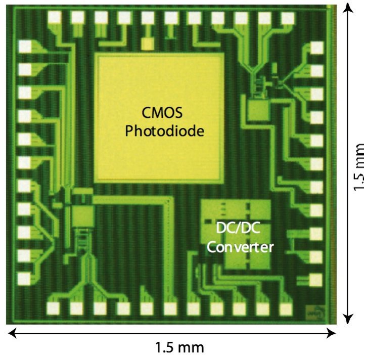
Figure 2.6. Micrograph of the second generation CMOS based optical power supply and transceiver chip.
