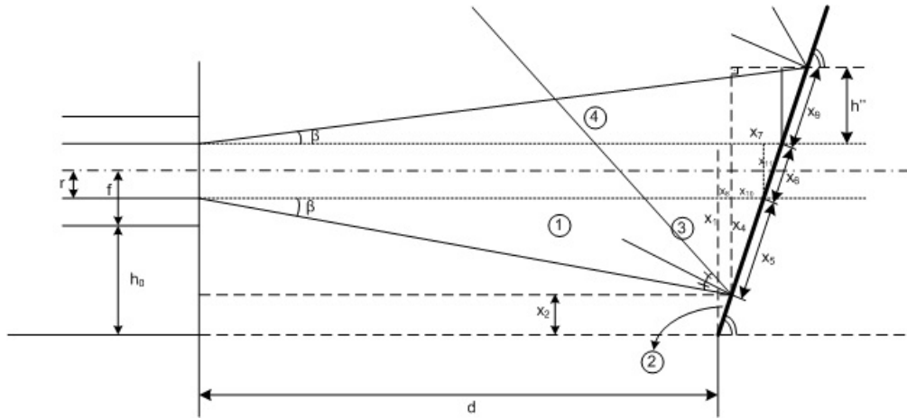
Figure 3.5. Rays leaving the optical fiber and reflecting from the mirror surface.
