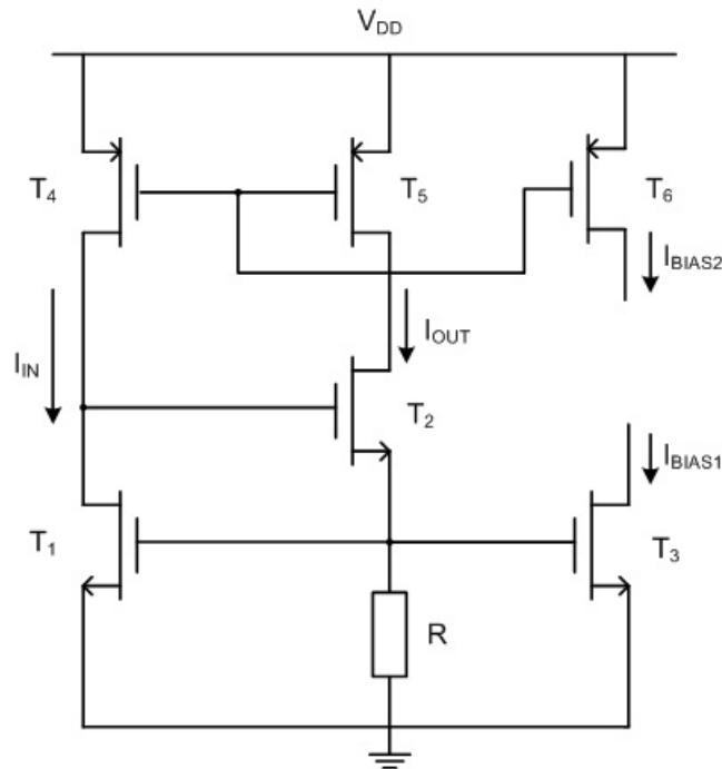
Figure 2.19. Self-biased current source.
