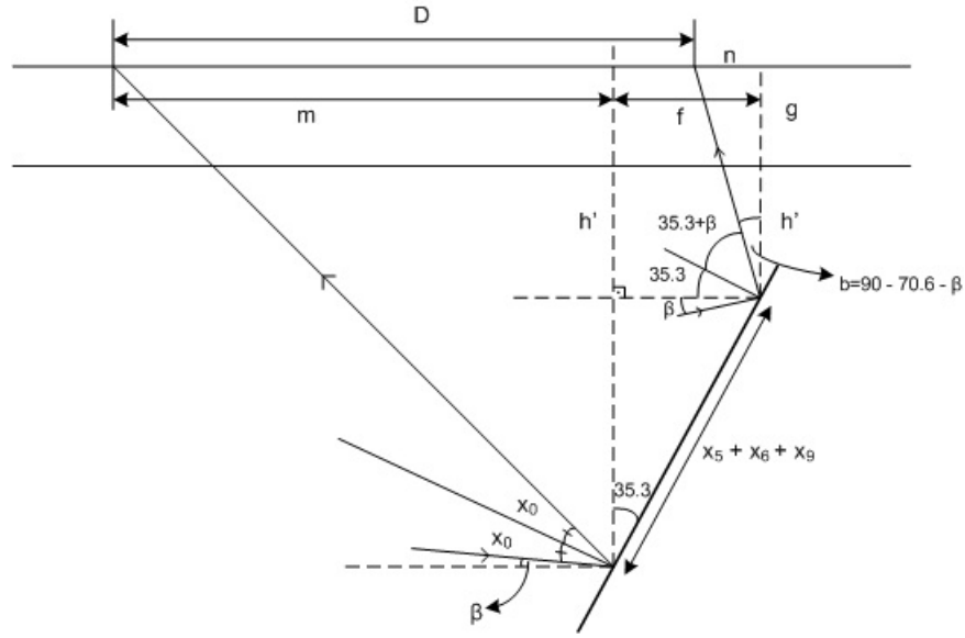
Figure 3.10. Reflected light beam from the mirror surface illuminates the surface of the IC.
