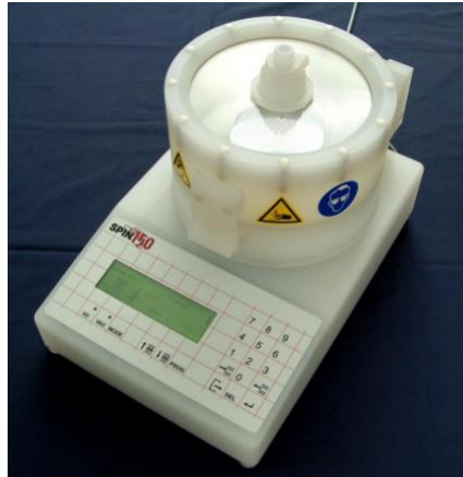
Figure 3.16. Spin coater.
