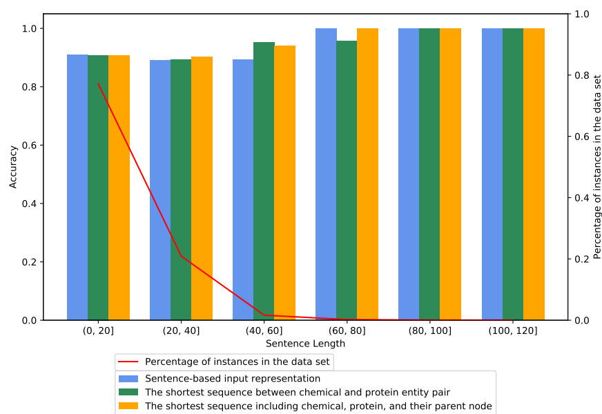
Figure 4.5. Accuracy scores for the distance between entity markers in sequences with our multi-class models.
