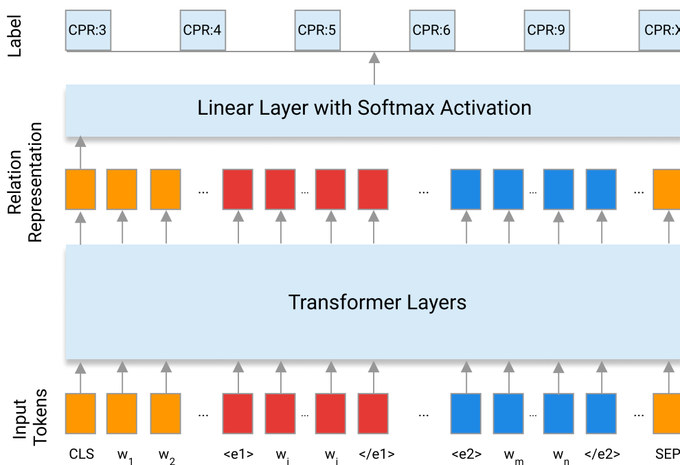
Figure 3.5. Multi-class Relation Extraction Model. The model is composed of a transformer-based model and a linear layer with softmax activation.
