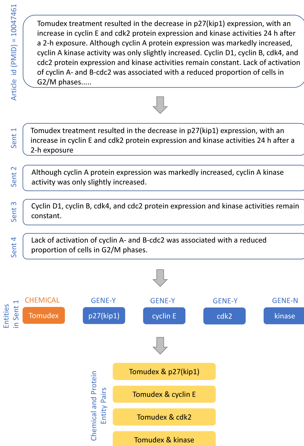
Figure 3.1. Examples of chemical and protein entity pair construction in an abstract with 10047461 PMID. Chemical (orange) and protein (blue) entity pairs constructed are colored in yellow.
