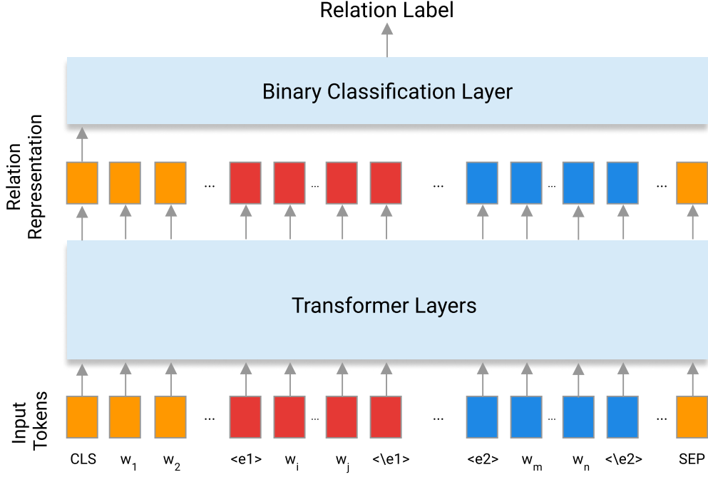
Figure 3.4. Binary Relation Extraction Model. The model is composed of a transformer-based model and a binary classification layer.
