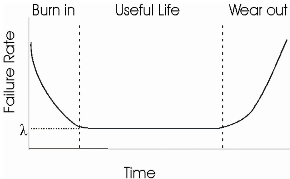
Figure 2.1. Hardware reliability
