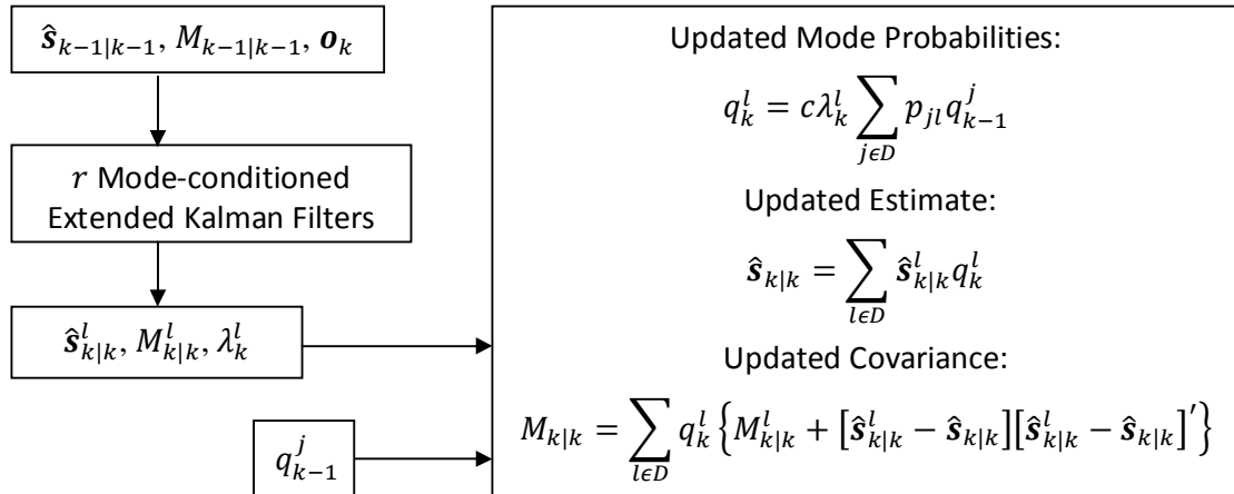
Figure 5.8. NOCM algorithm
