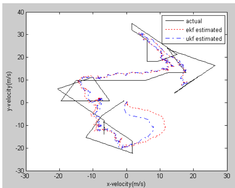
Figure 6.12. Actual velocities(solid line) and NOCN-estimated velocities(dotted line for EKF estimation, dashed line for UKF estimation) of a sample trajectory for high mobility model
