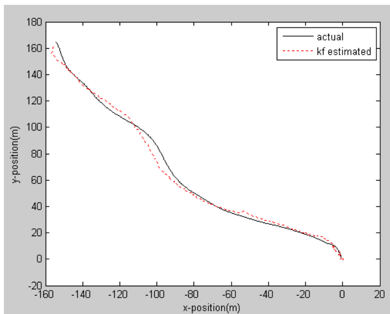
Figure 6.1. Actual positions(solid line) and LOCN-estimated positions(dotted line) of a sample trajectory for low mobility model
