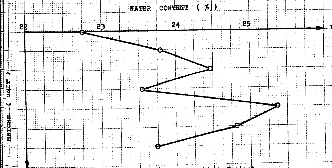
Fig 4.25 Height ( Unit ) versus Water Content
