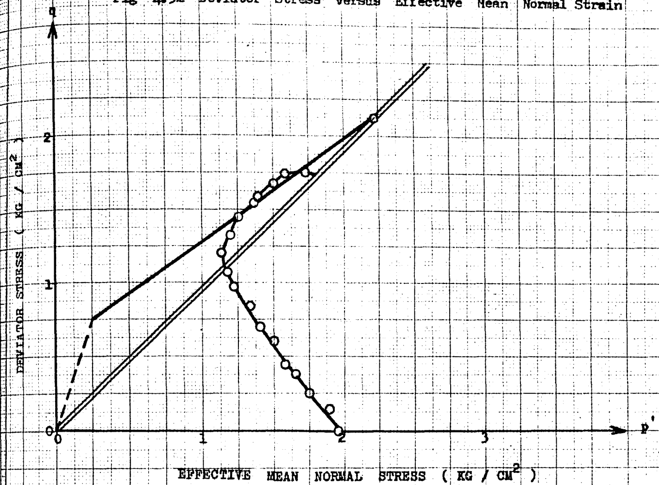
Fig 4.32 Deviator Stress versus Effective Mean Normal Strain
