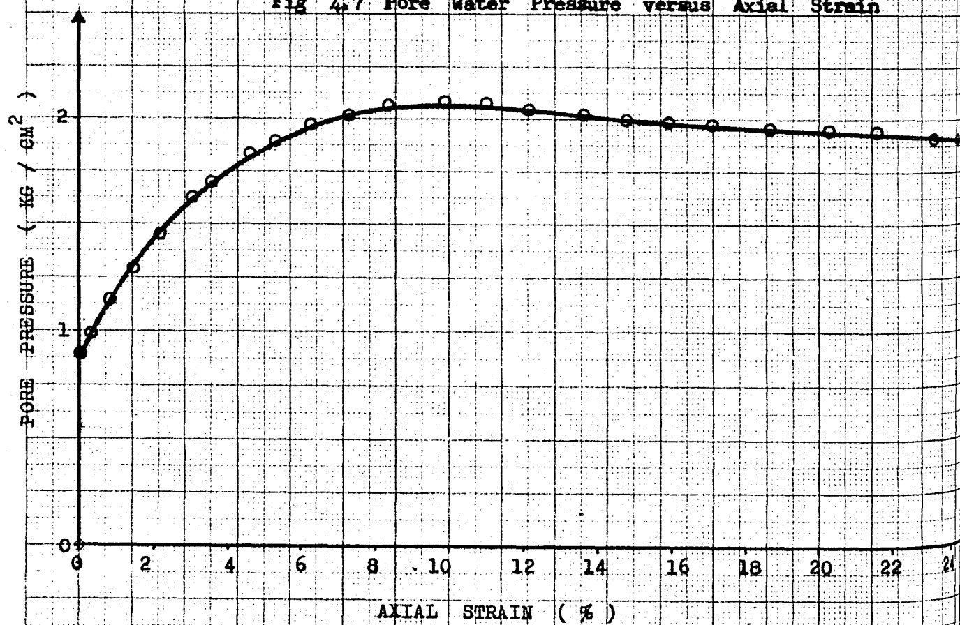
Fig 4.7 Pore Water Pressure versus Axial Strain
