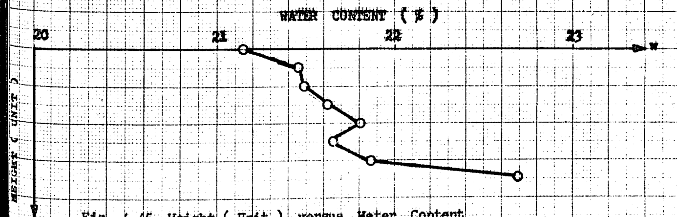
Fig 4.45 Height (Unit) versus Water Content
