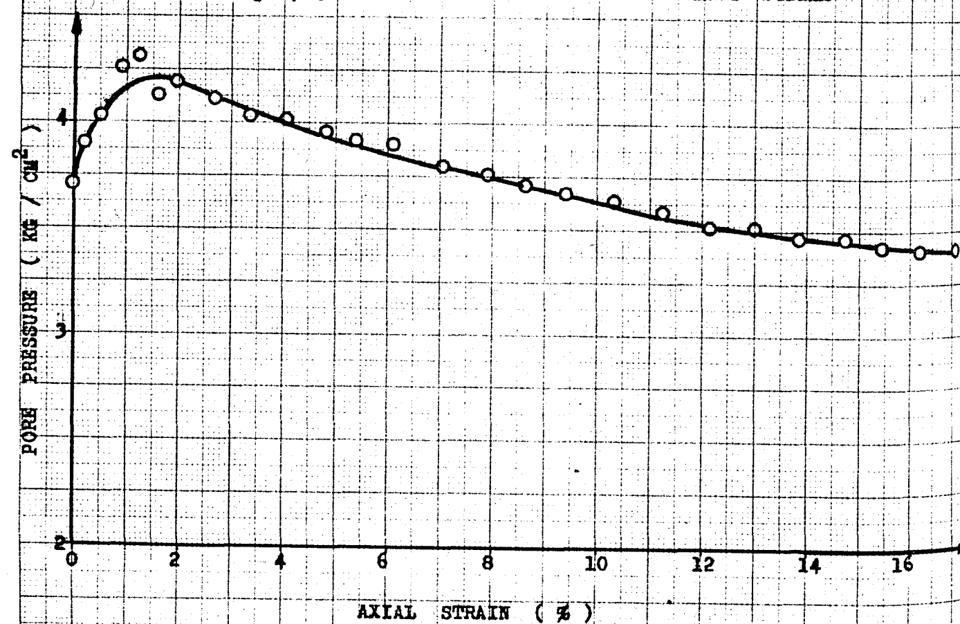
Fig 4.15 Pore Water Content versus Axial Strain
