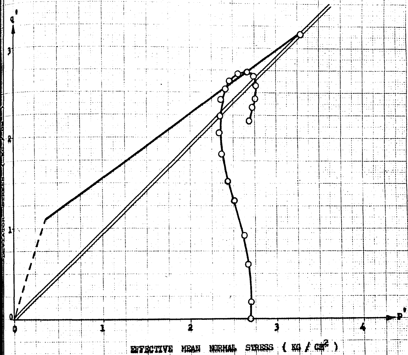
Fig 4. 48 Deviator Stress versus Effective Mean Normal Stress
