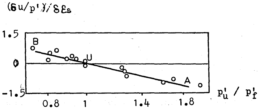
Fig 2.18 Rate of pore pressure change in undrained test ( After Parry, 1958 )
