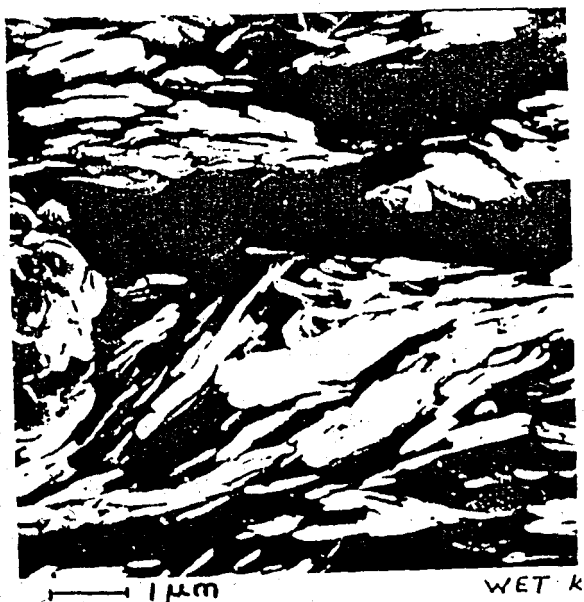
Fig 2.3 (b) Microstructure of Kaolin compacted wet of optimum
