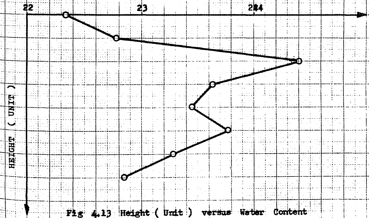
WATER CONTENT (%)
