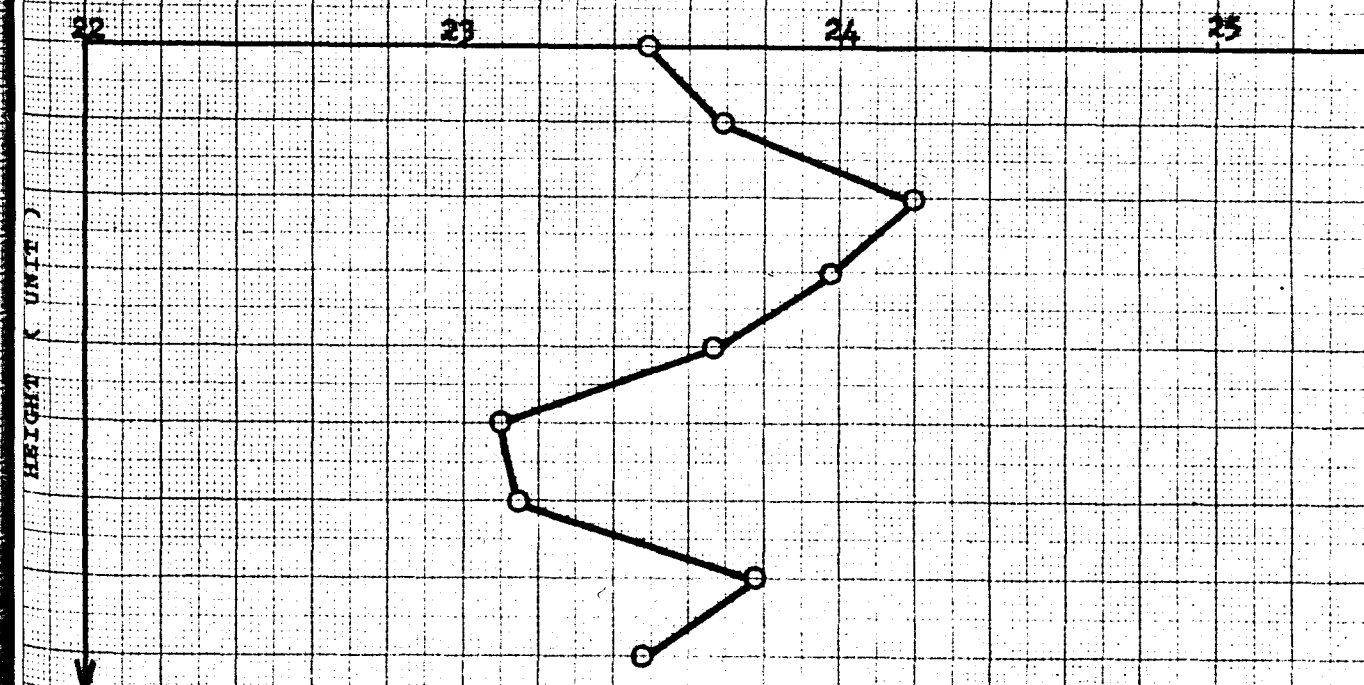
Fig 4.85 Height (Unit) versus Water Content
