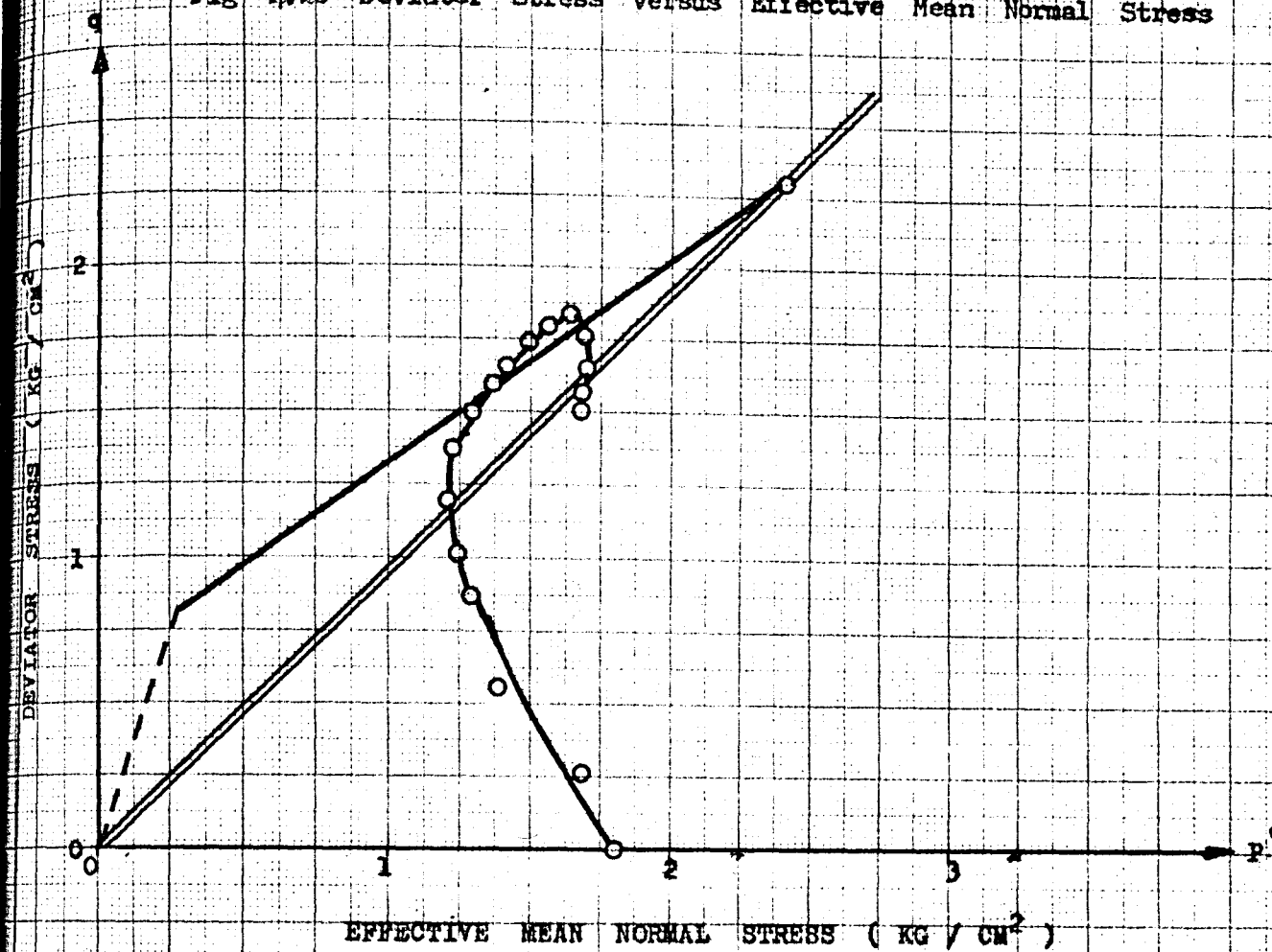
Fig 4.28 Deviator Stress versus Effective Mean Normal Stress
