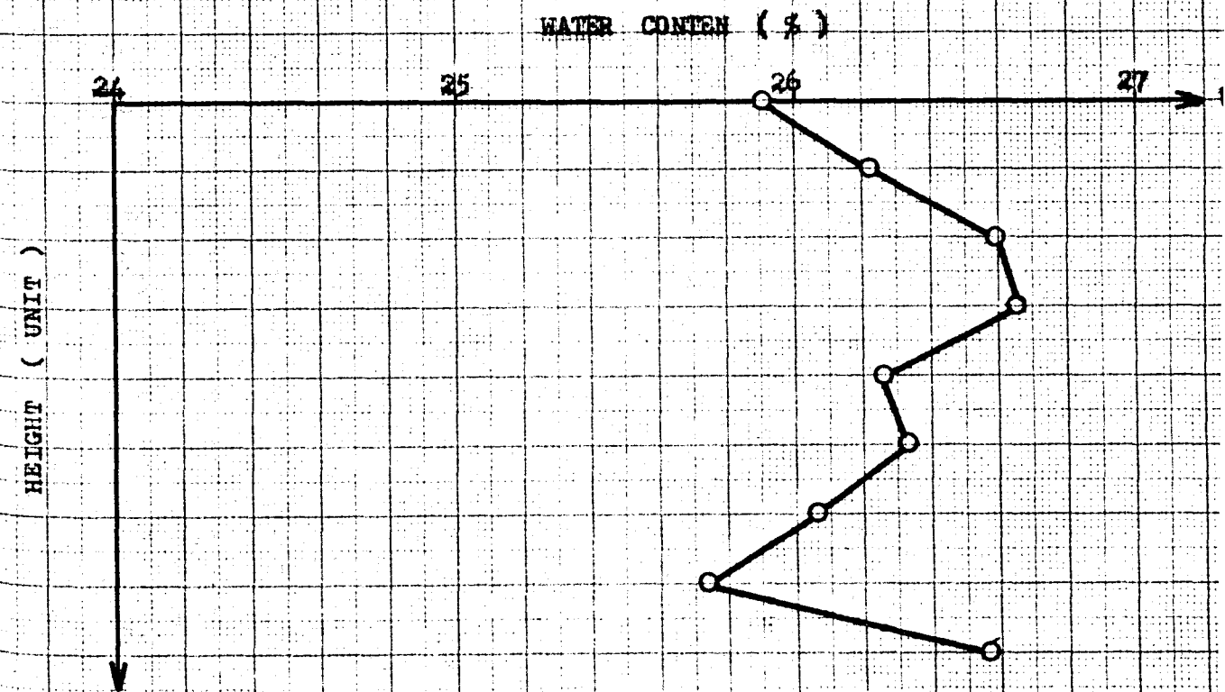
Fig 4.73 Height (Unit) versus Water Content
