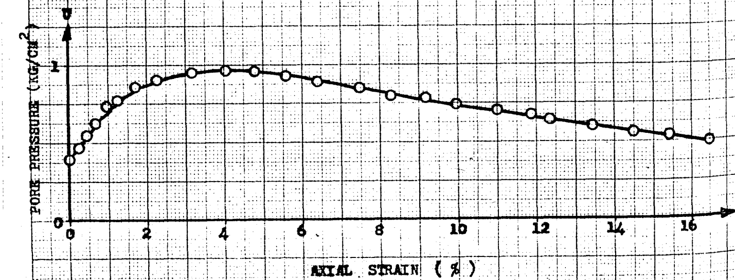
Fig 4.51 Pore Water Pressure versus Axial Strain
