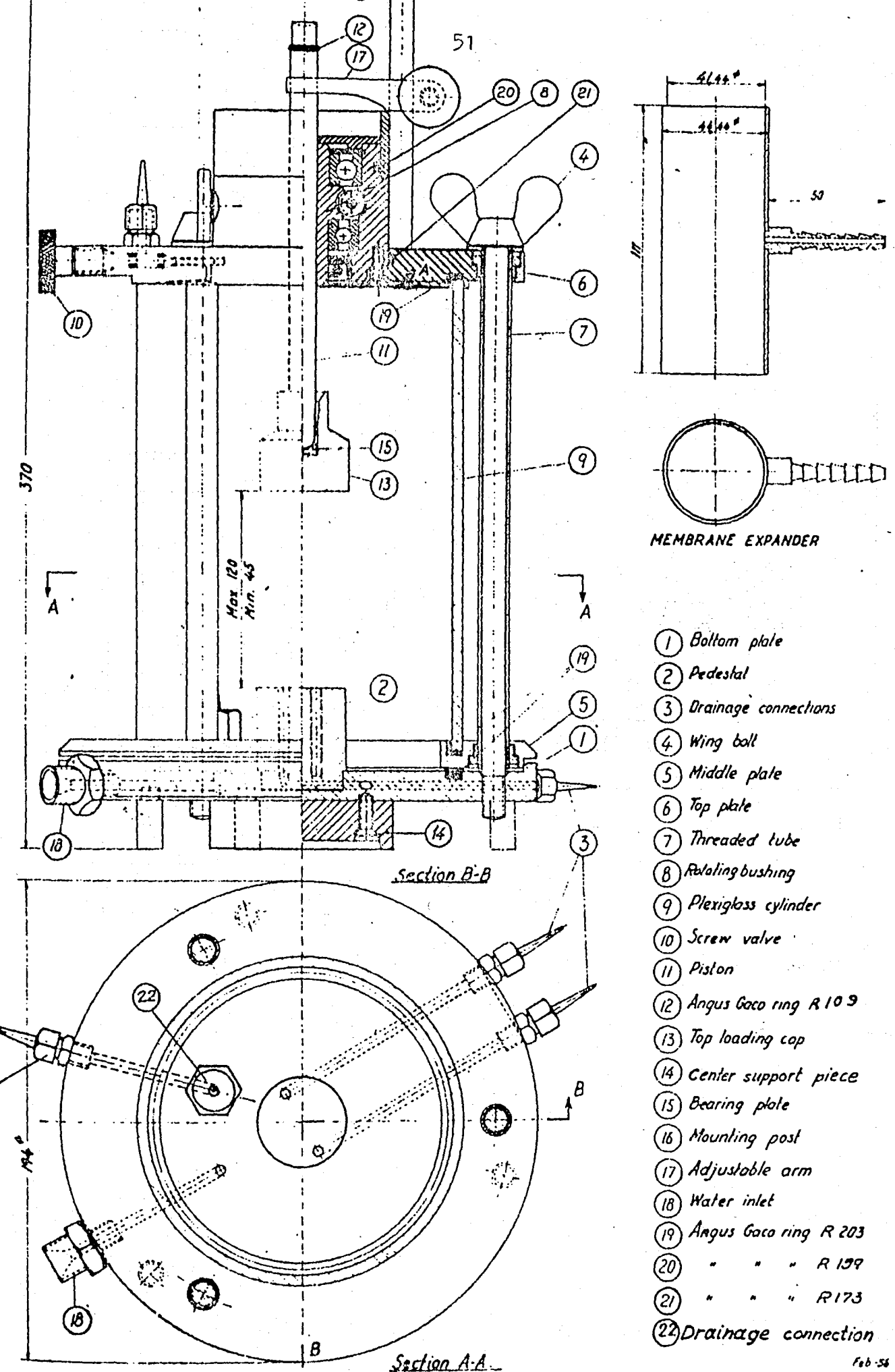
Fig 3.1 Triaxial Cell
