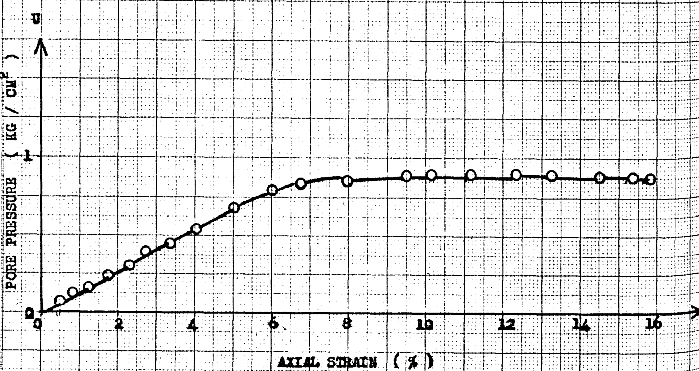
Fig 4.63 Pore Water Pressure versus Axial Strain
