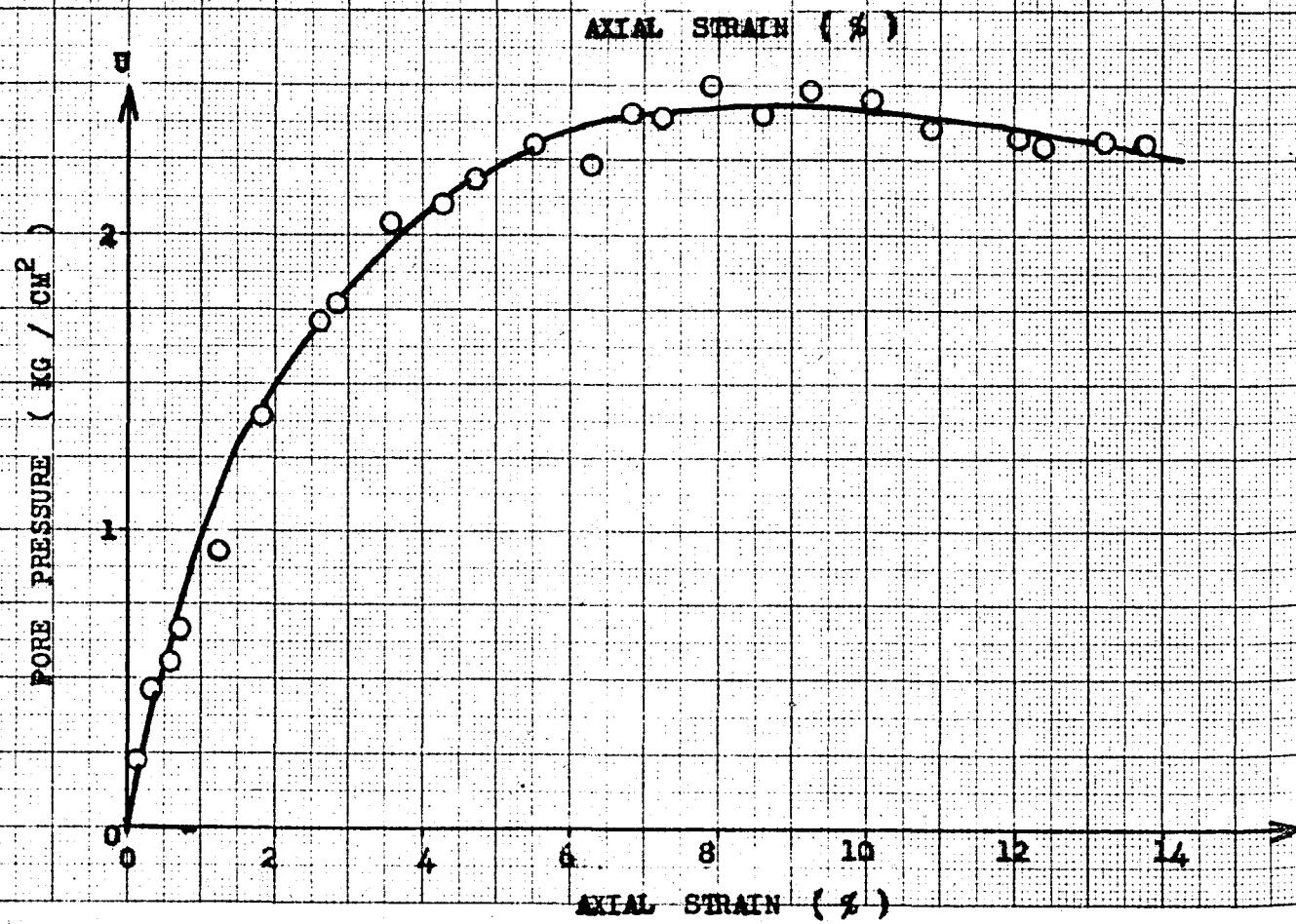
Fig 4.75 Pore Water Pressure versus Axial Strain
