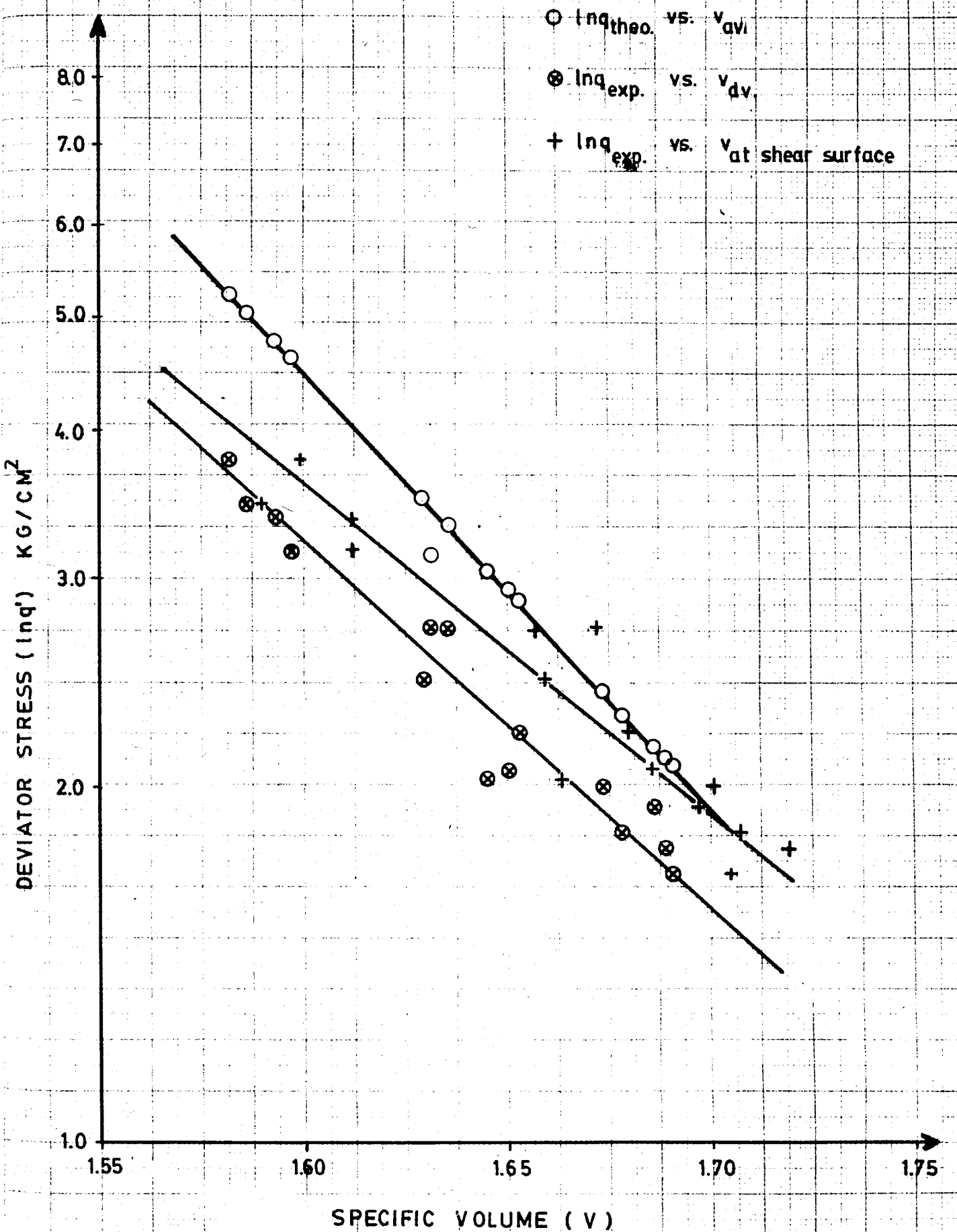
Fig 5.2 Deviator Stress ( \ln q' ) vs. Specific Volume
