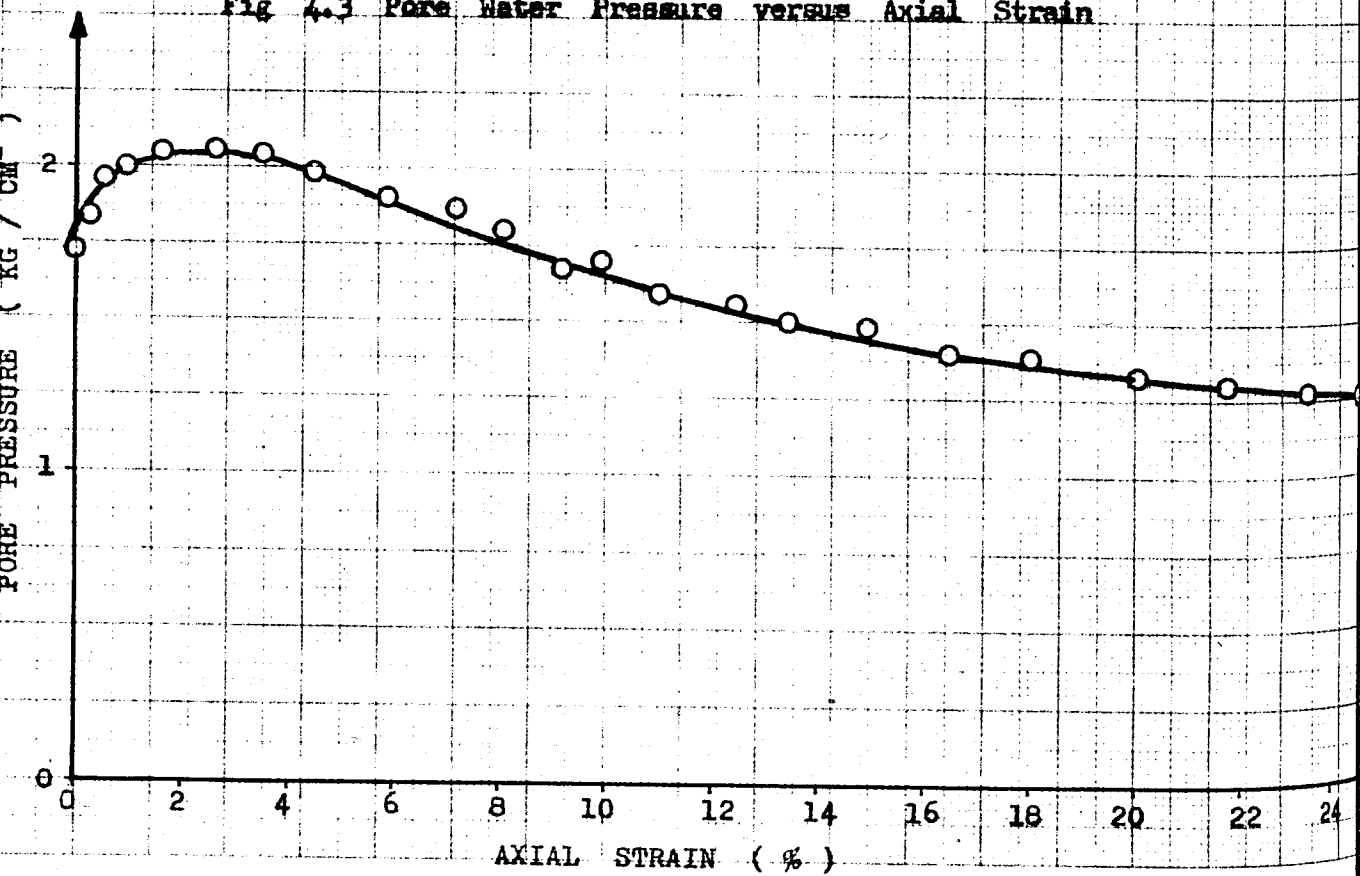
Fig 4.3 Pore Water Pressure versus Axial Strain
