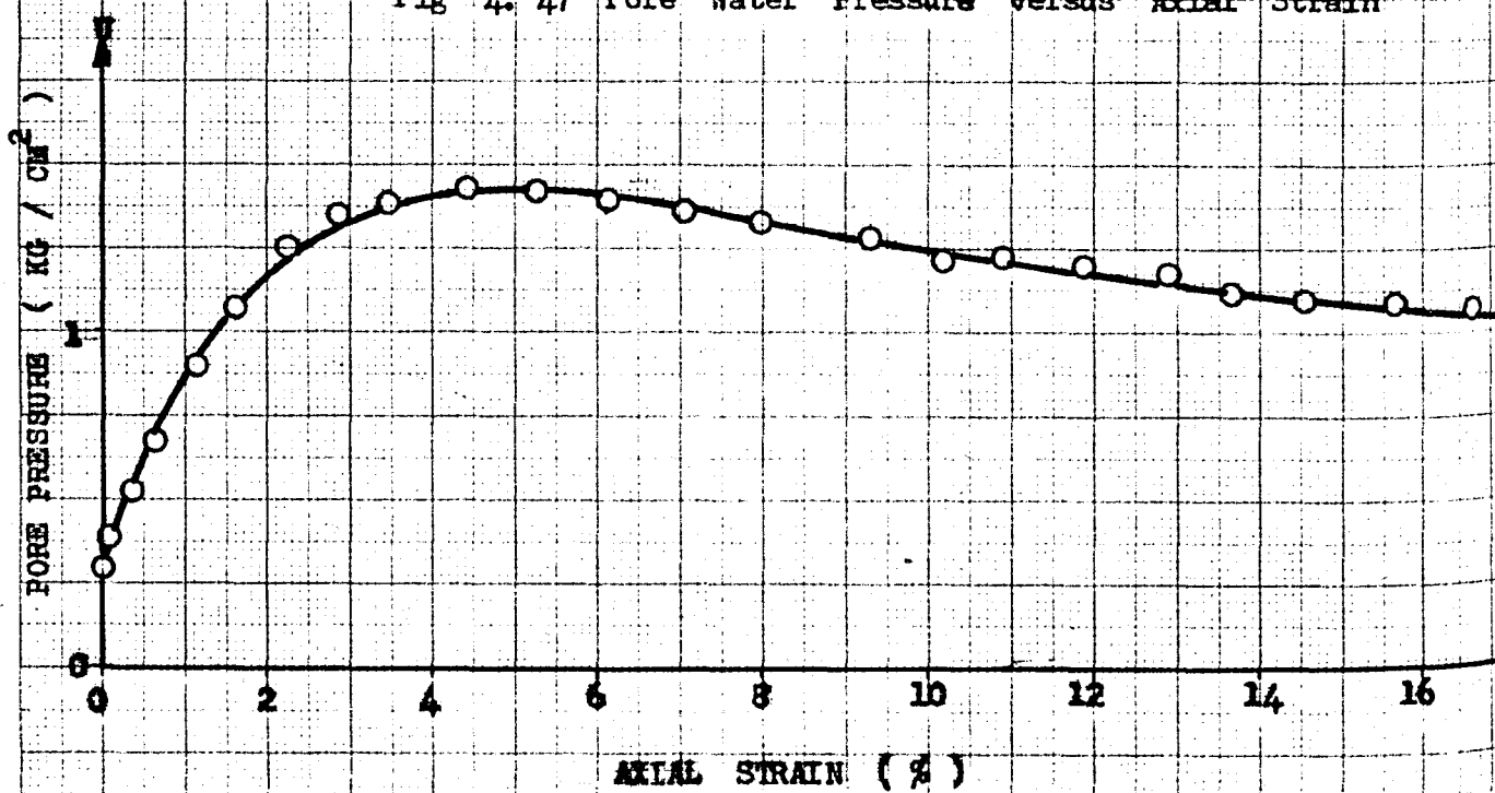
Fig 4. 47 Pore Water Pressure versus Axial Strain
