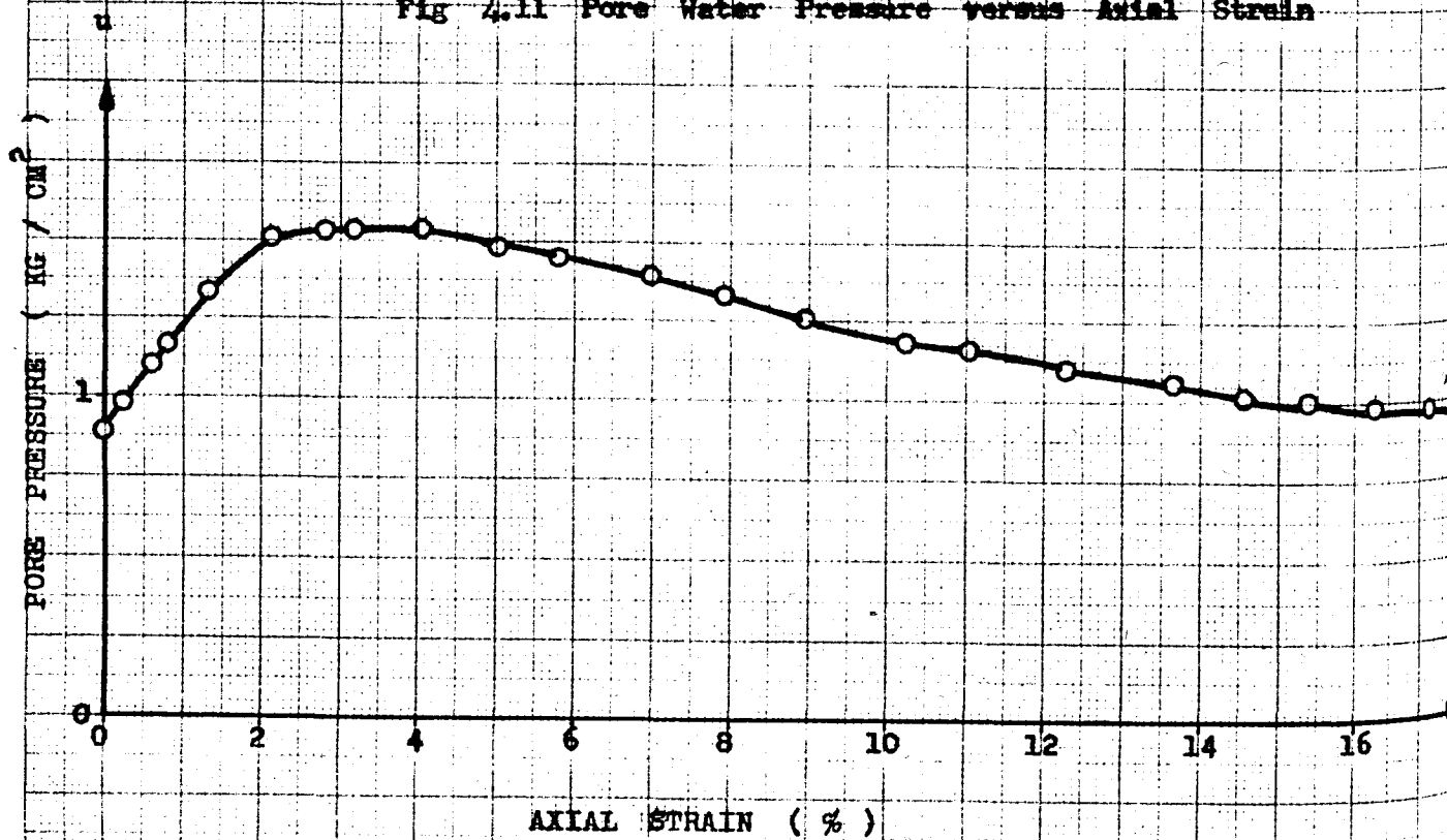
Fig 4.11 Pore Water Pressure versus Axial Strain
