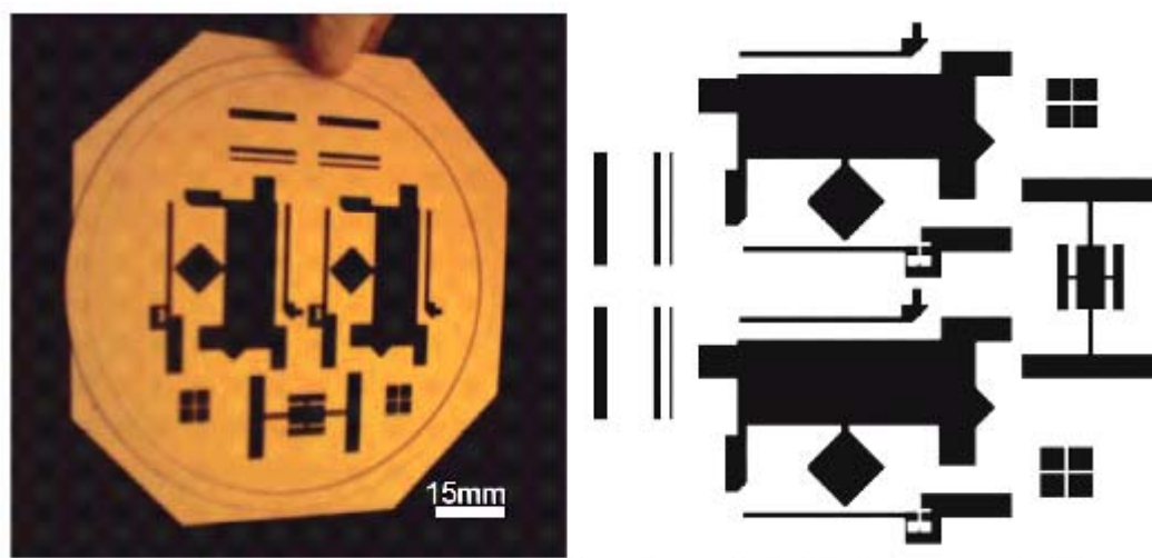
Figure 2.24. Shadow mask prepared by laser cutter (left) and its CAD design (right)
