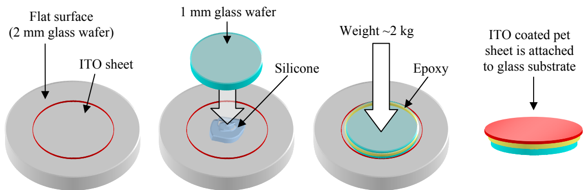
Figure 2.2. The attachment of ITO coated PET to the 1 mm glass substrate
