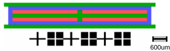
Figure 2.8. Alignment marks for four layer micro fabrication process
