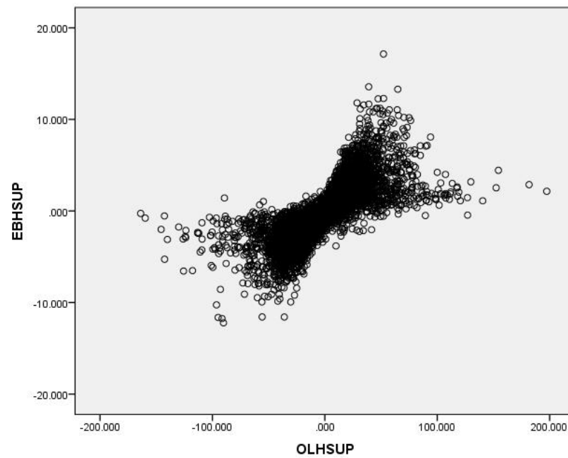
Figure B4. EB versus OL residuals for the home study support (HSUP) slopes in Level-2
