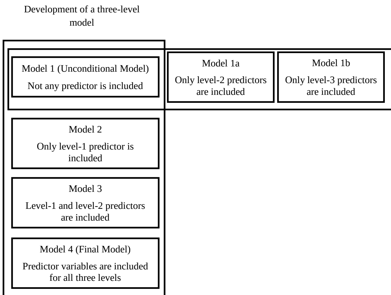
Figure 3. Development scheme of the models
