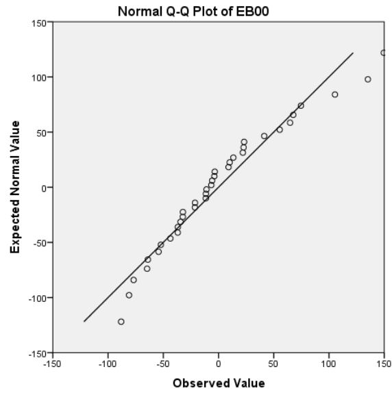
Figure B3. Normal Q-Q curve of Level-3 residuals for 36 countries based on the final fitted model
