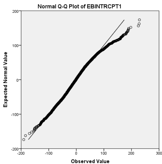
Figure B2. Normal Q-Q curve of Level-2 residuals for 6,586 schools based on the interception model
