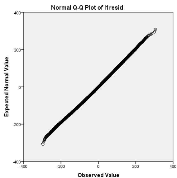
Figure B1. Normal Q-Q curve of Level-1 residuals for 219,788 students based on the final fitted model
