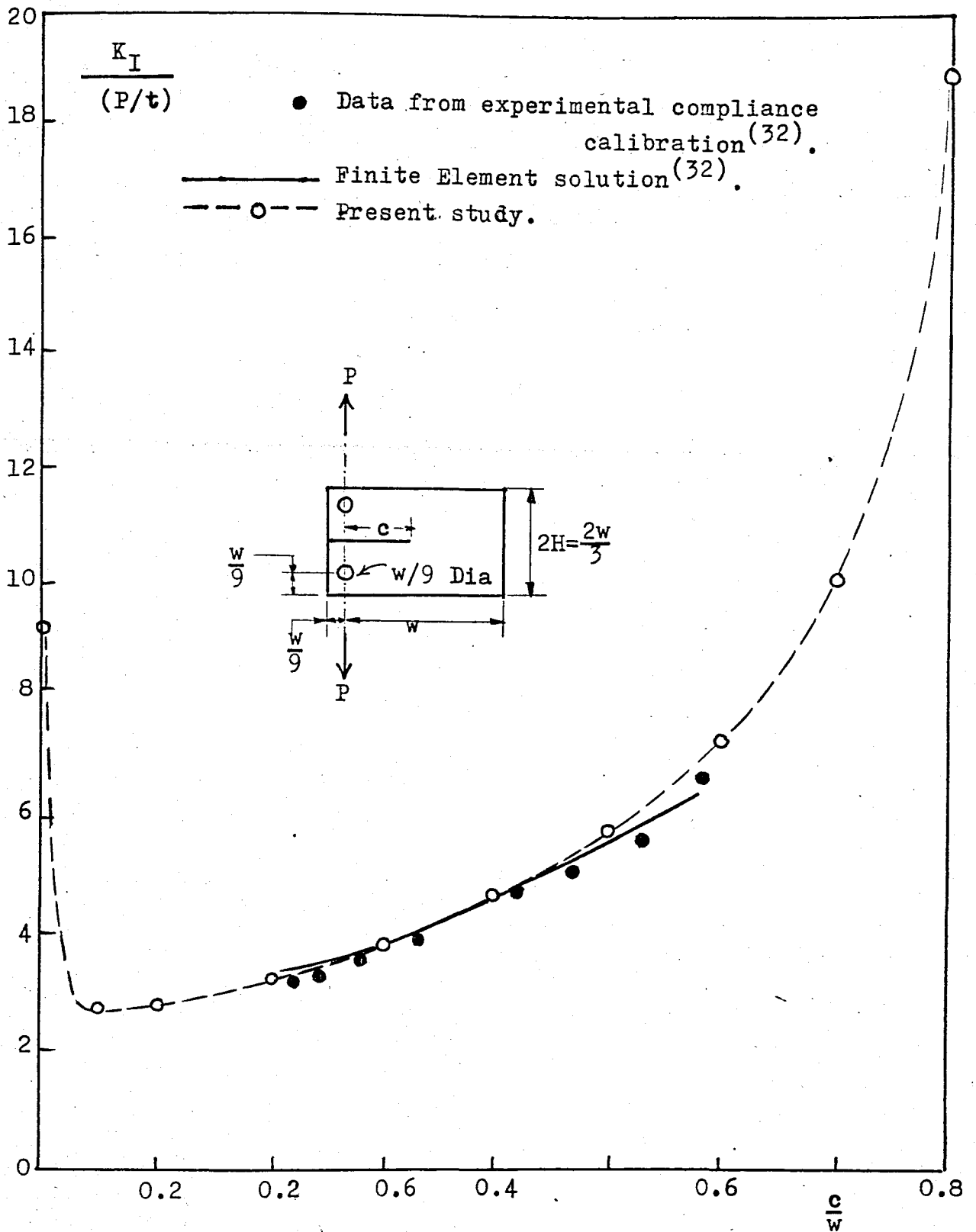
Figure 25. Comparison of the experimental data points and the finite element solution of Mandell et. al. (32) with the present study for the stress intensity factors in a Double Centilever Beam specimen subjected to a concentrated force P .
