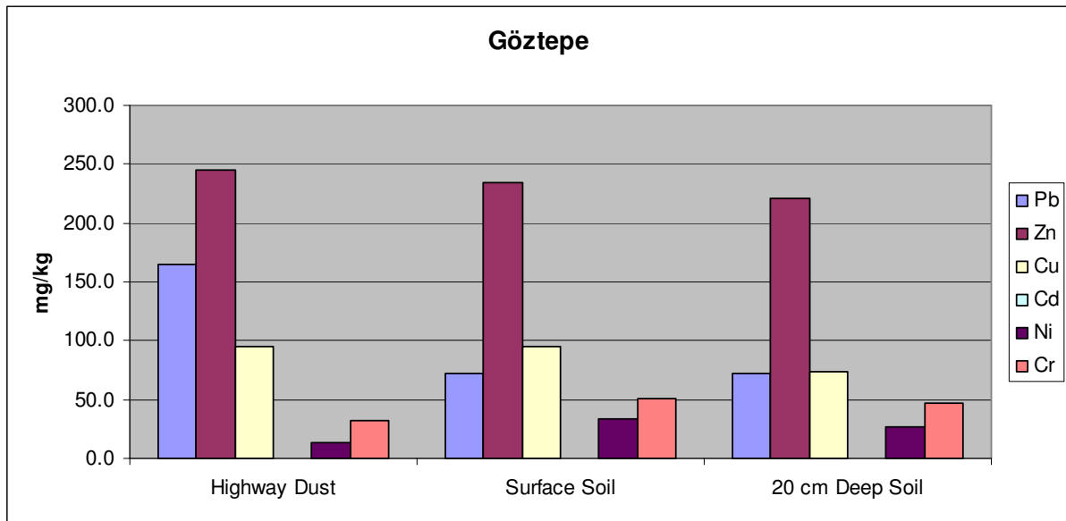
Figure 5.4. Pollution Distribution in Göztepe
