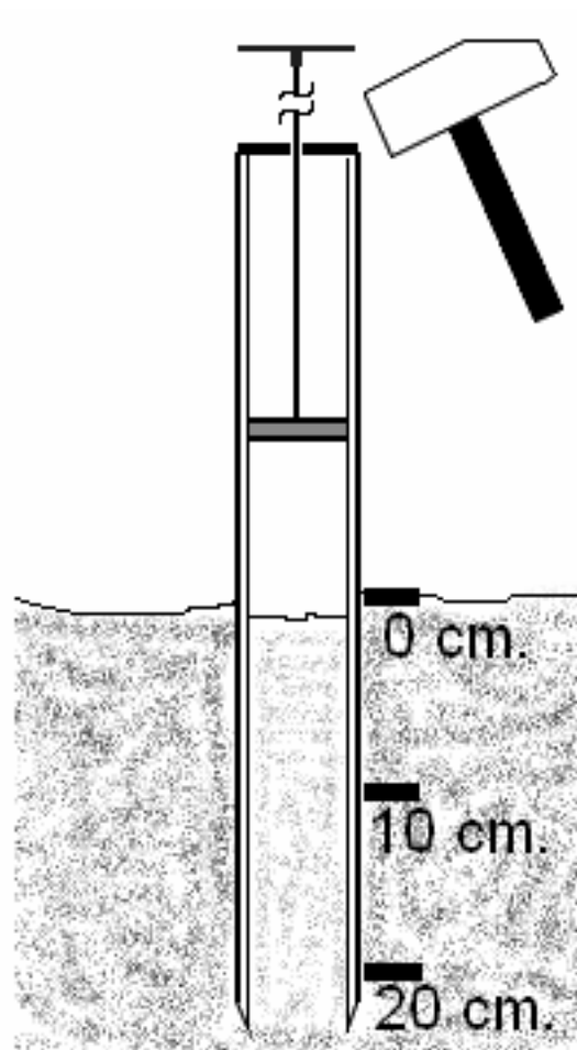
Figure 4.2. Schematics of Sampling Operation
