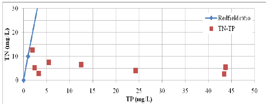
Figure 5.27. TN over TP ratios for Station 13
