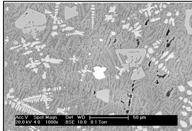
Figure 5.17. SEM of 05/709-2
