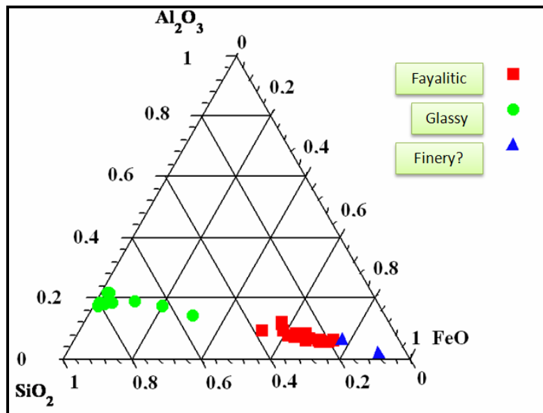
Figure 5.13. SEM (EDAX) data of slags plotted on ternary diagram (mass fraction)
