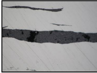
Figure 5.29. Microstructure of polished sample 06/119A
