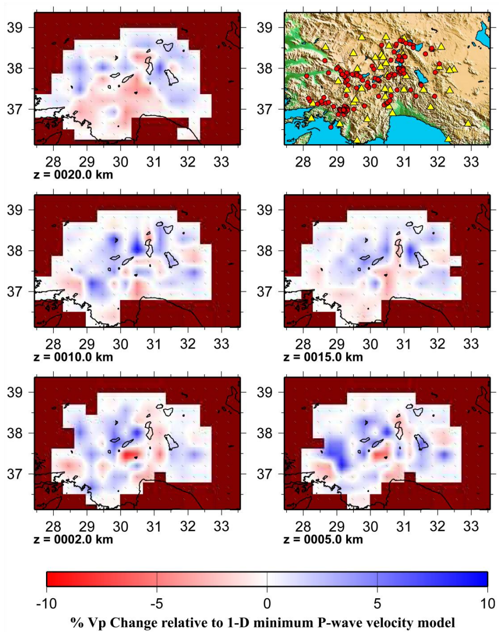
Figure 6.10. Horizontal plane views of Vp perturbations (per cent) relative to the initial 1-D minimum velocity model for different layers down to 20 km. Red circles and yellow triangles represent the events and stations, respectively
