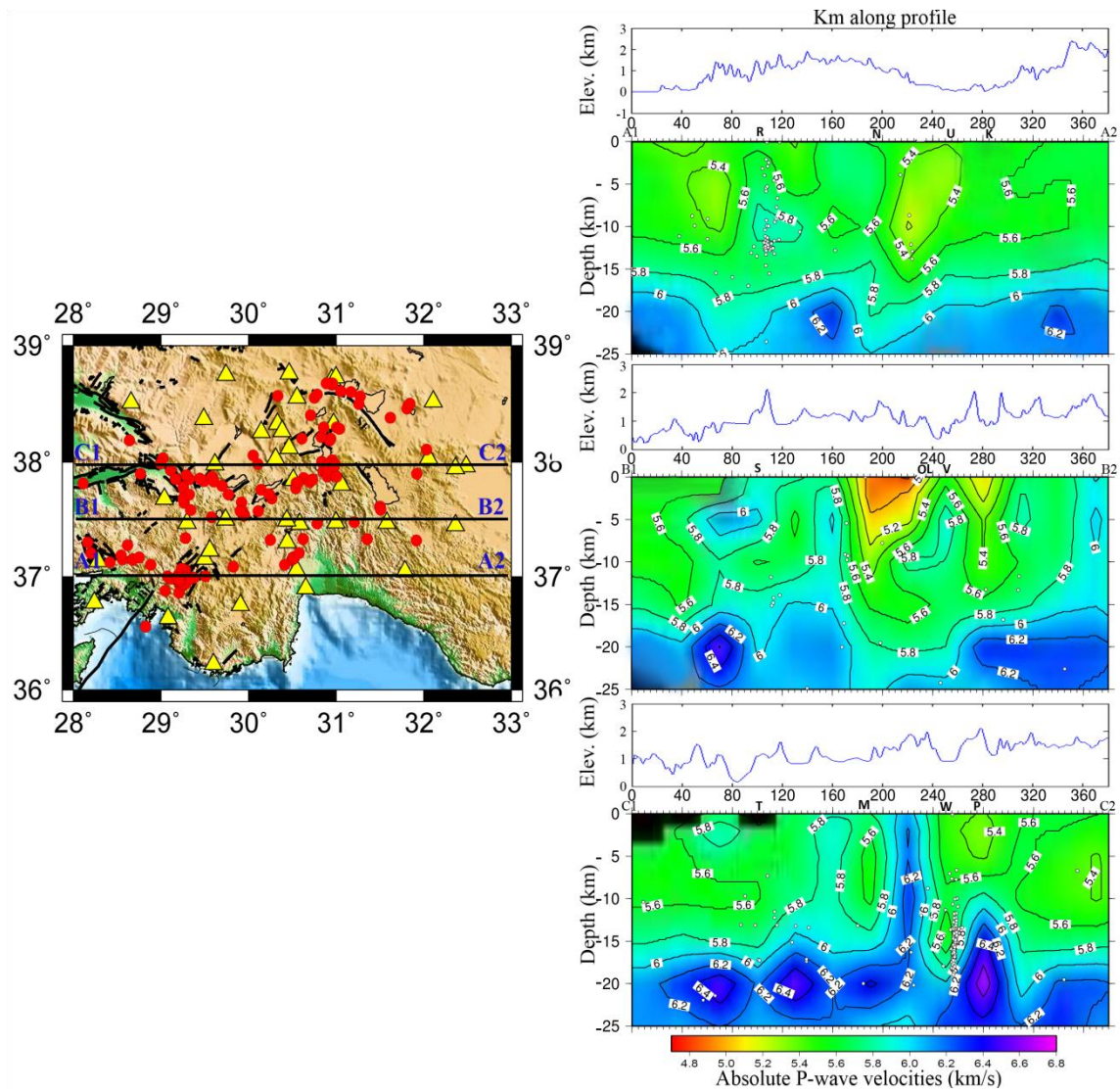
Figure 6.12. P-wave velocity distribution along three profiles (A1-A2 (right up), B1-B2 (right middle), C1-C2 (right down)) for constant latitude values. Yellow triangles denote stations, red and white circles denote earthquake locations
