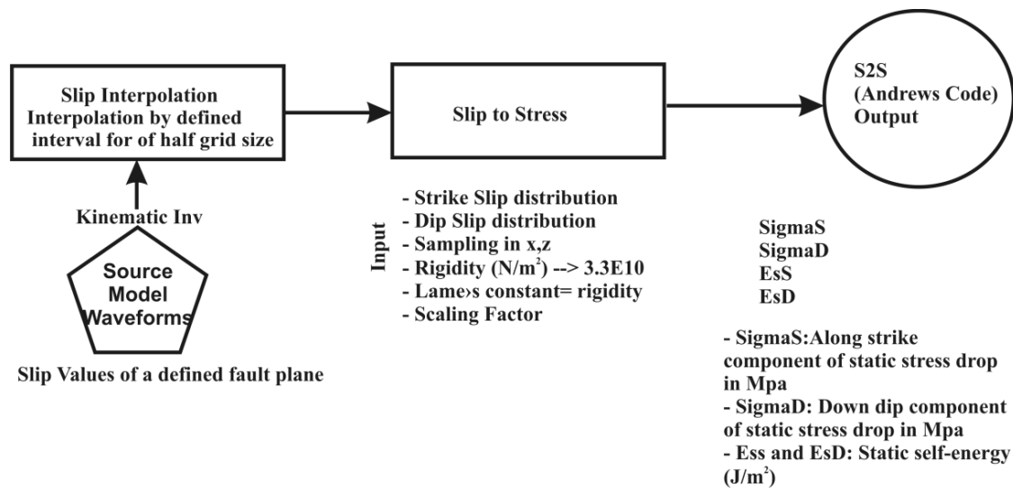
Figure 4.7. Schematic diagram to prepare SORD input.
