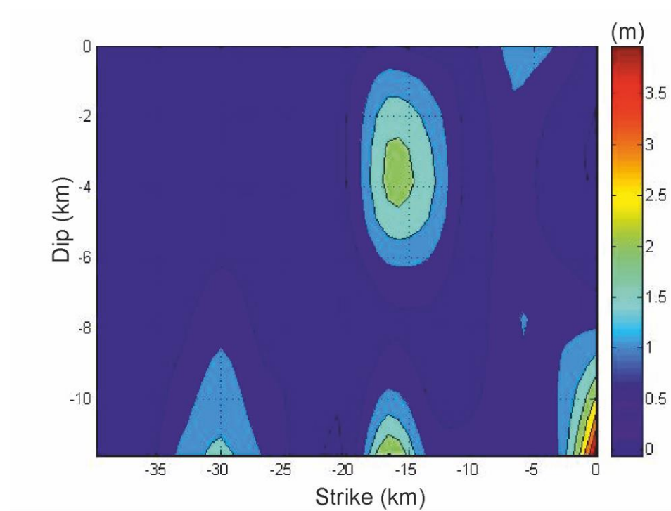
Figure 2.5. The slip distribution for the Duzce earthquake faulting area. A band-pass filter with 0.01-0.5 Hz applied to the to the observed data.
