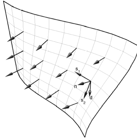
Figure 4.6. Slip vectors on a non-planar fault. Instead of classical source representation, vectors (unit normal \hat{n} ) downward unit vector ( \hat{d} ) specify the strike and dip in coordinate system ( \hat{s}_1, \hat{s}_2 \times \hat{n} ).
