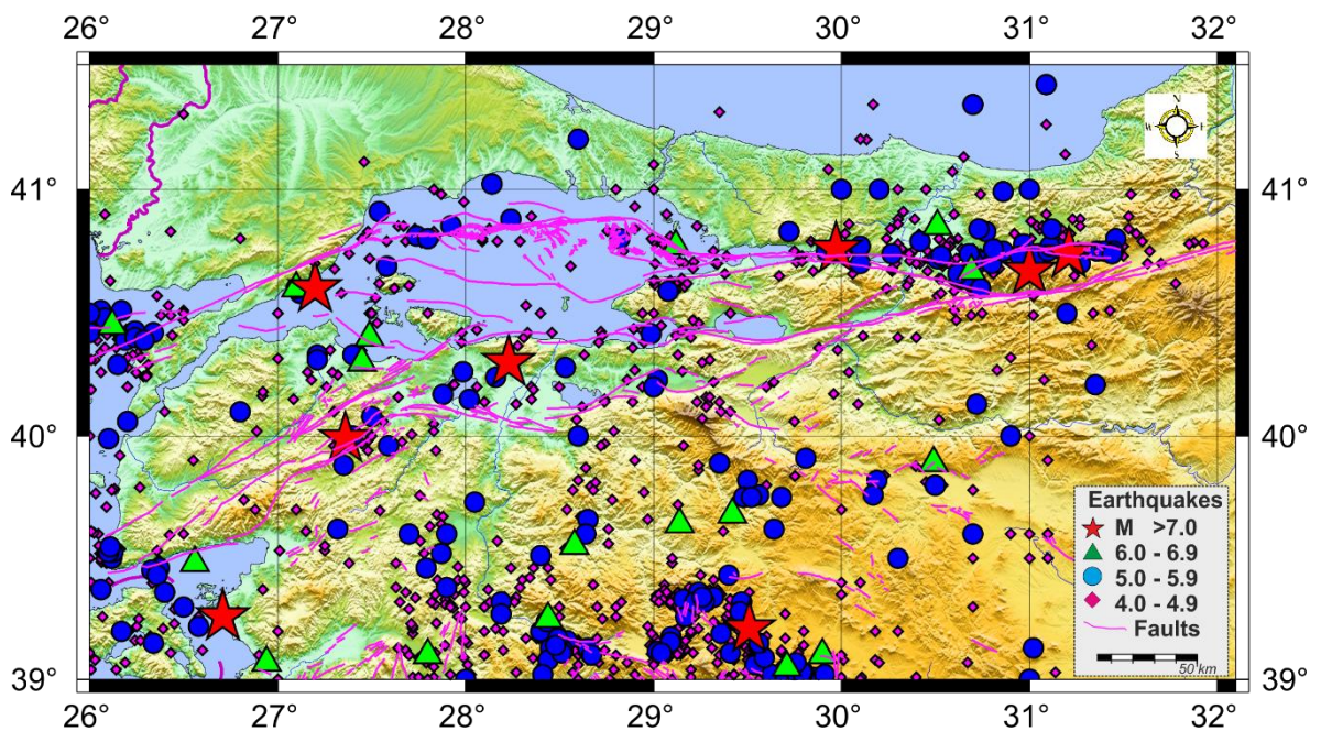
Figure 1.2. Recent seismicity and historical earthquakes and active fault map of the Marmara Region. Earthquake catalogs with magnitude M > 4.0 (1900-2016 taken from KOERI catalog. The pink lines present active faults in the Marmara Region (Şaroğlu et al., 1992; Barka, 1996; Ambraseys, 2002; Armijo et al., 2005).
