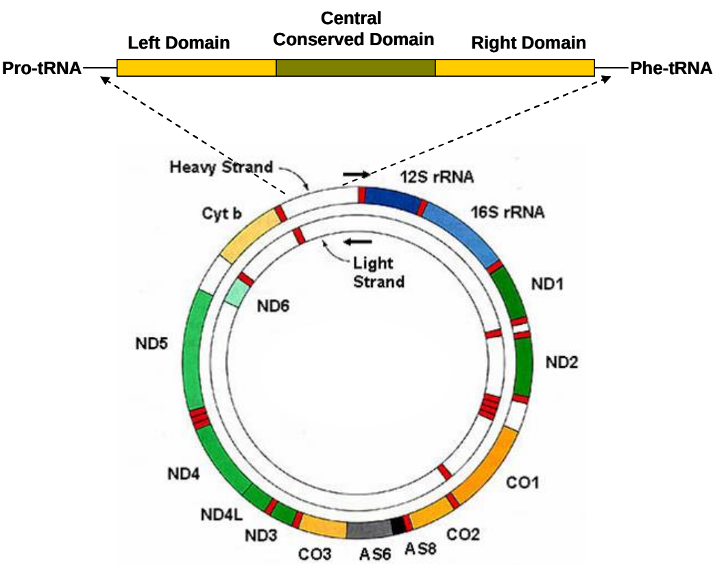
Figure 1.3. Vertebrate mitochondrial genome with amplified control region.
