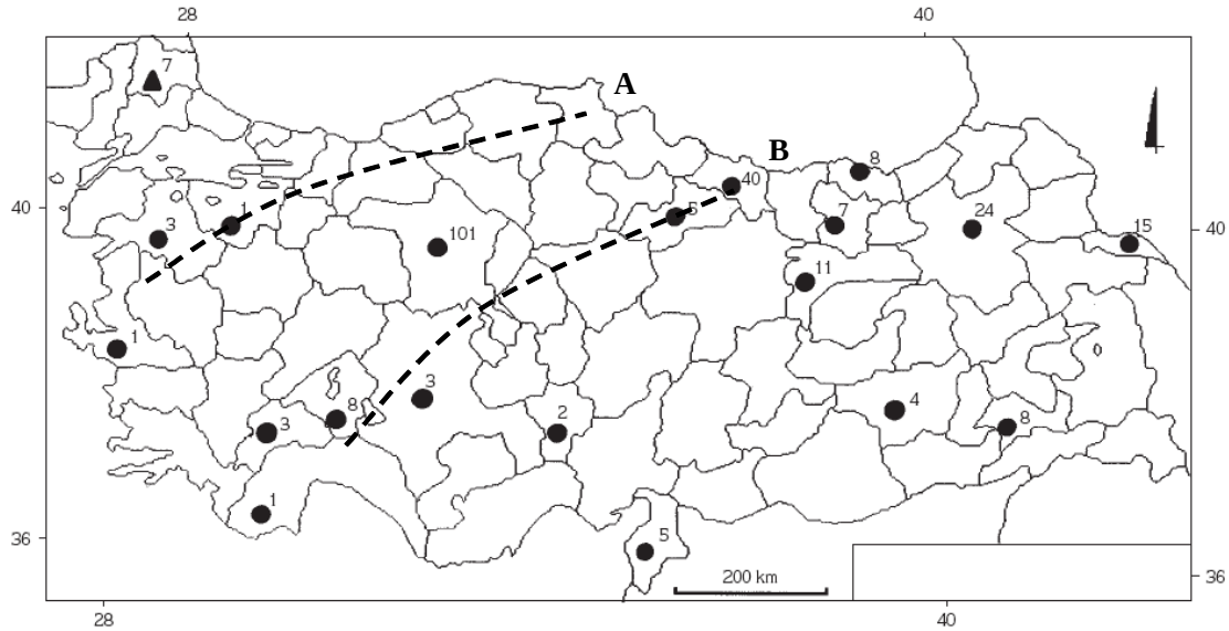
Figure 1.2. Distribution of M. s. pallidus and M. s. schreibersii in Turkey. According to Albayrak and Coşkun (2000): the presence of M. s. pallidus is marked by circles and M. s. schreibersii by triangles. According to Karataş and Sözen (2004): M. s. pallidus is found below the line B and M. s. schreibersii above the line A. The area between A and B is a transition zone.
