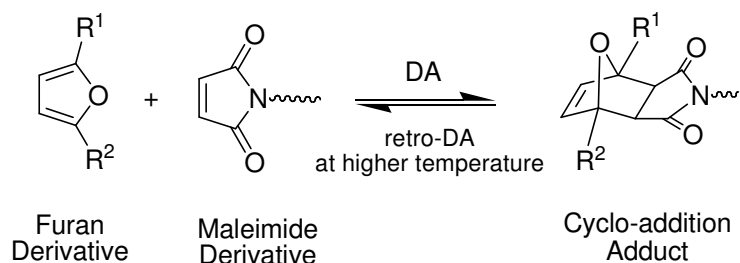
Figure 1.1. Representation of the DA and rDA reactions [2]
