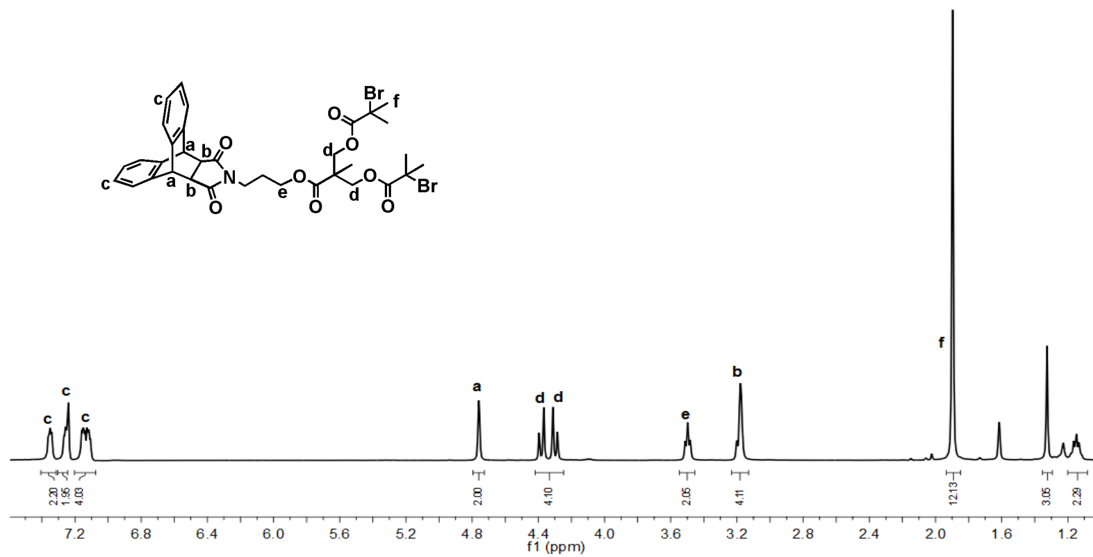
Figure A.19. ^1\text{H} NMR spectrum of 20
