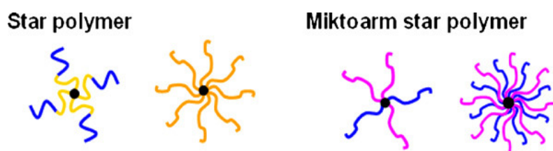
Figure 1.14. Categories of star polymers [32]
