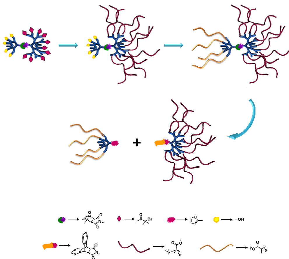
Figure 2.2. Synthetic approach for miktoarm polymer and thermal cleavage.
