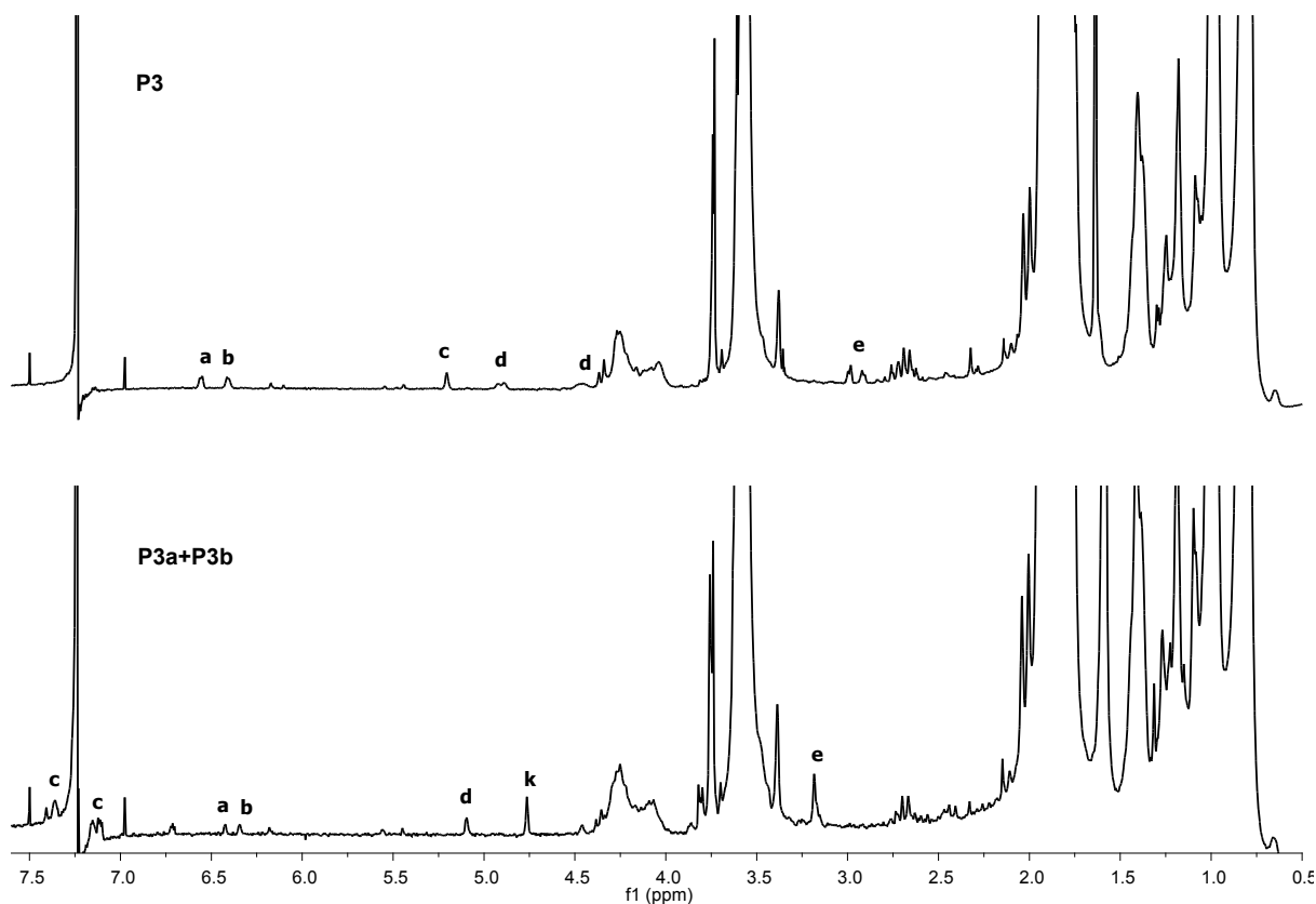
Figure 3.12. ^1\text{H} NMR spectrum of retro Diels-Alder products of 8-arm polymer, 3a and 3b
