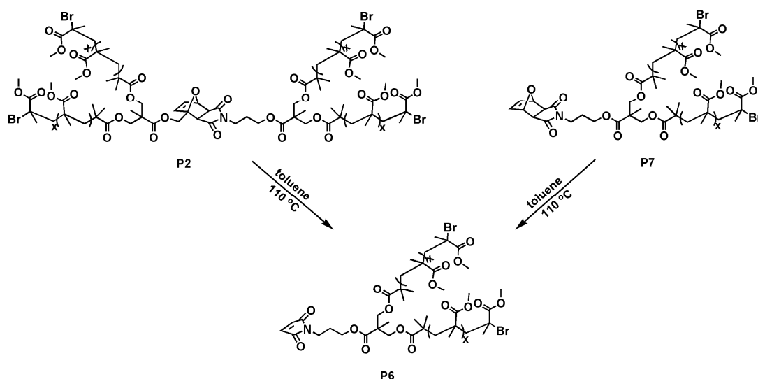
Figure 3.30. Synthesis of reactive polymer
