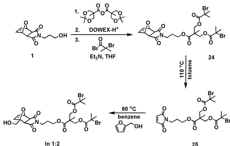
Figure 4.12. Synthesis of In1:2 ATRP and ROP initiator
