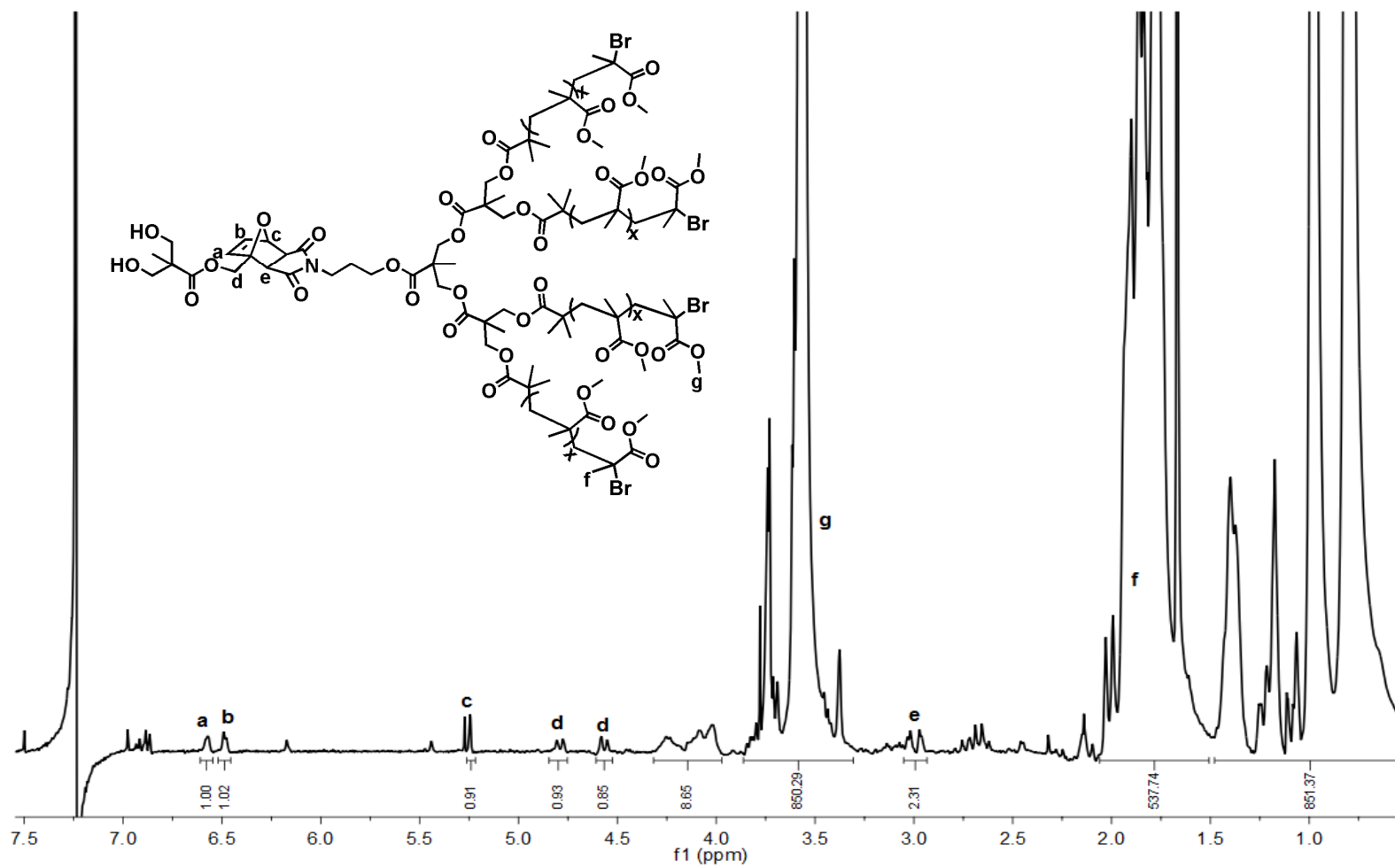
Figure A.39. ^1\text{H} NMR spectrum of 2OH:4PMMA
