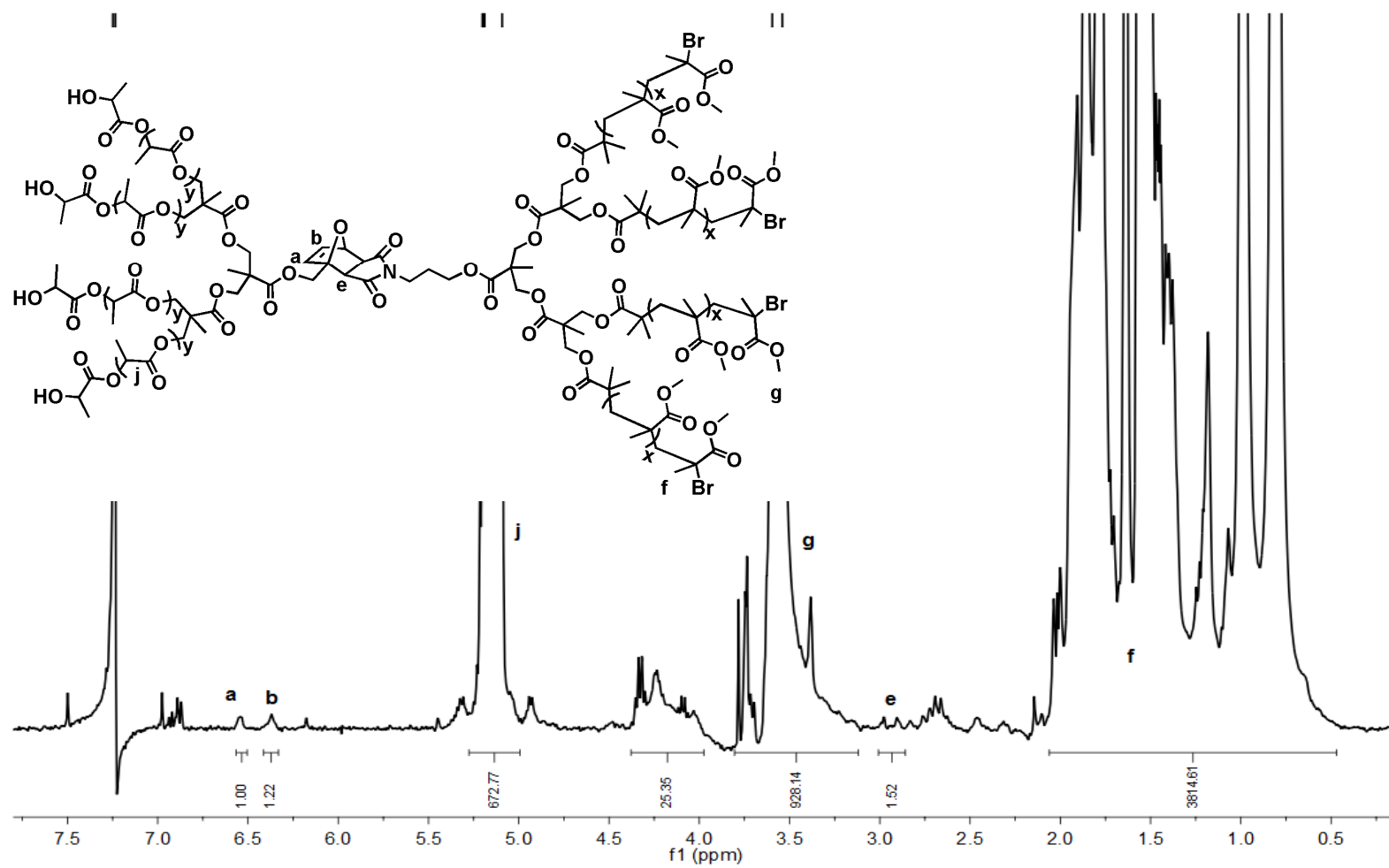
Figure A.43. ^1\text{H} NMR spectrum of 4PLA:4PMMA
