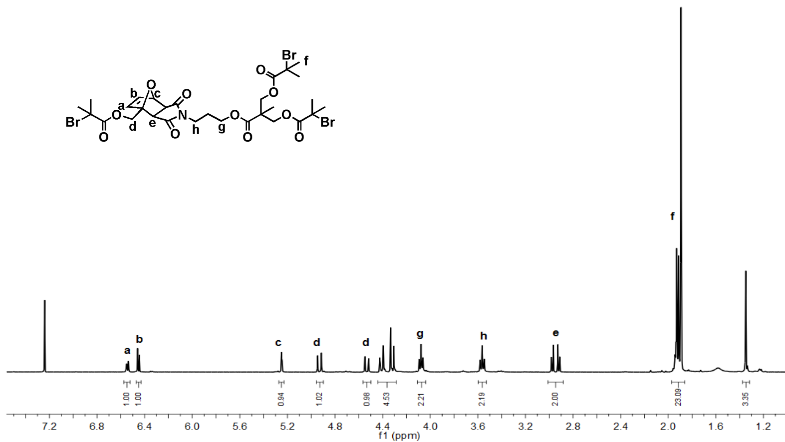
Figure A.2. ^1\text{H} NMR spectrum of 3arm initiator ( In1 )
