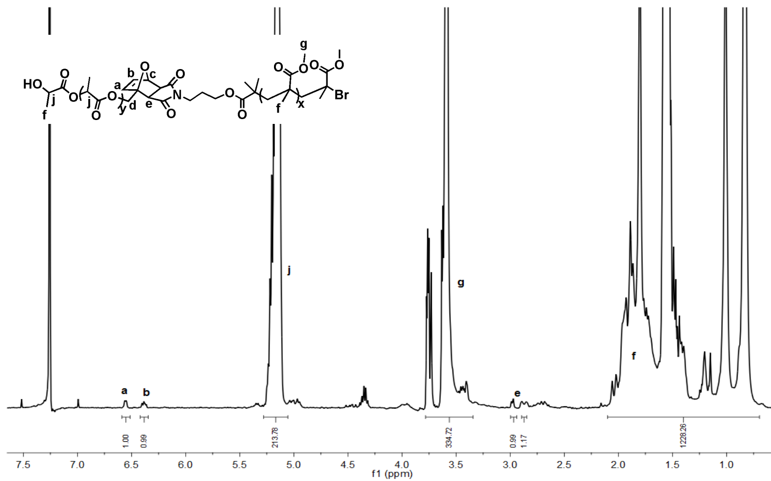
Figure A.28. ^1\text{H} NMR spectrum of 1PLA:1PMMA
