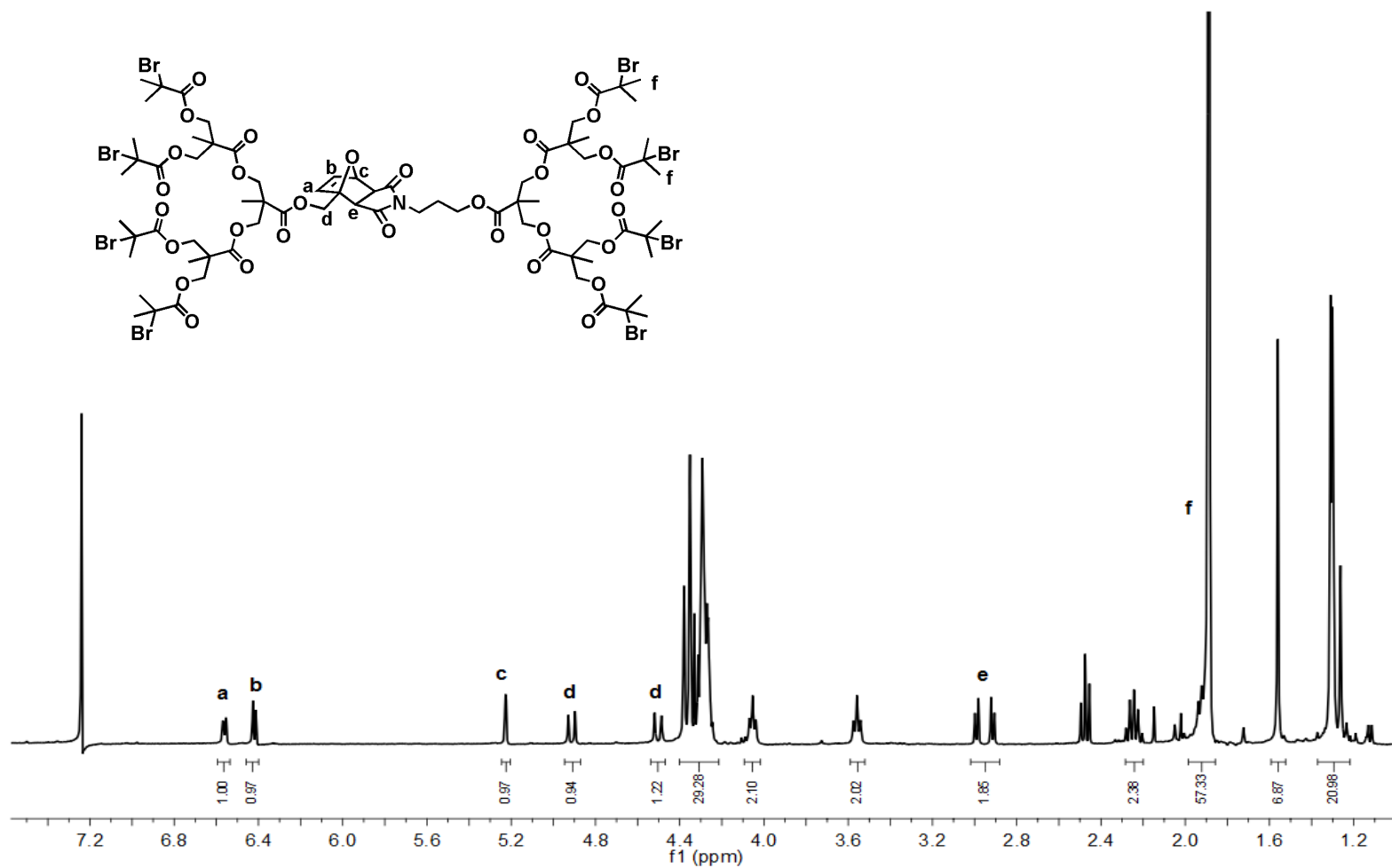
Figure A.4. ^1\text{H} NMR spectrum of 8arm initiator ( In3 )
