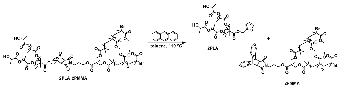
Figure 3.27. Thermal cleavage of 2PLA:2PMMA miktoarm polymer
