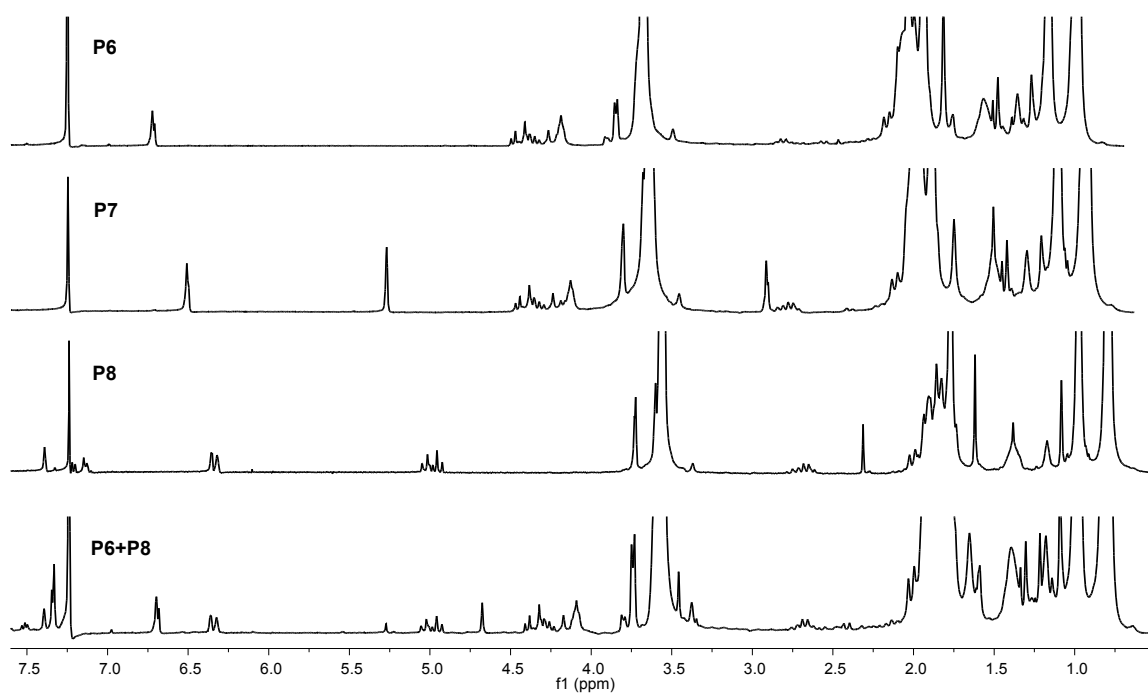
Figure 3.18. 1 H NMR spectra of P6 , P7 , P8 and mixture of P6 and P8
