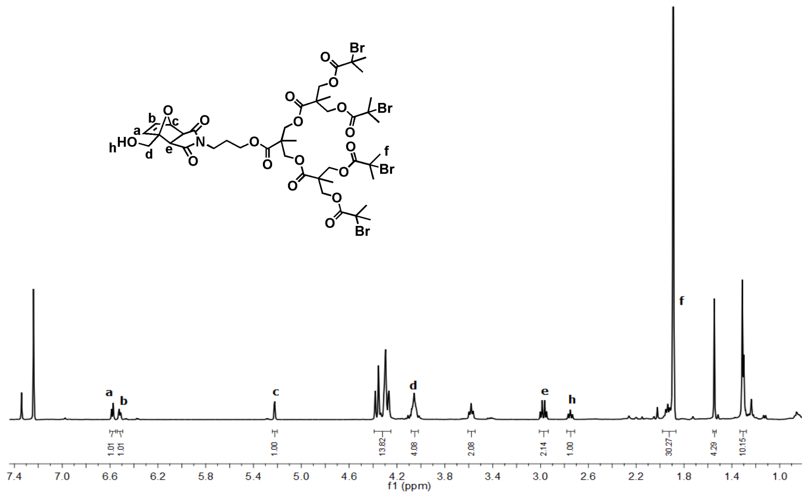
Figure A.24. ^1\text{H} NMR spectrum of In1:4
