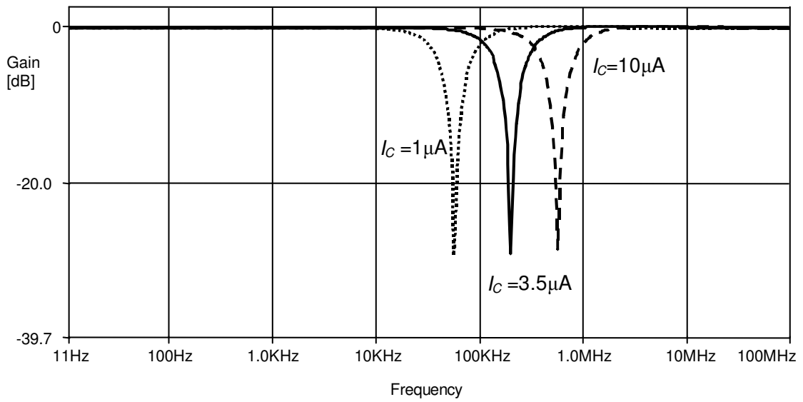
Figure 3.17. Illustrating electronic tunability of the proposed circuit (The center frequency of the filter is tuned between 57.5kHz and 575kHz through various control currents I_{C1}=I_{C2}=I_C )
