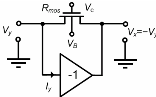
Figure 2.2. The MOS resistive cell (MRC) for canceling even order non-linearities of the MOS transistor
