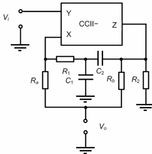
Figure 3.19. Notch/all-pass filter example in (Higashimura and Fukui, 1988)
