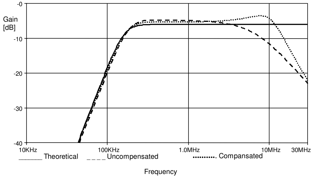
Figure 3.29. Theoretical and simulated frequency responses of the example ladder prototype with the compensated and uncompensated FDNR simulator
