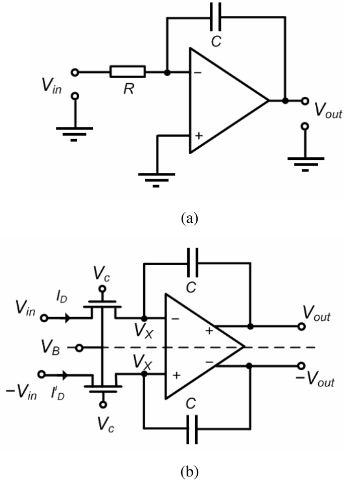
Figure 2.1. (a) An active-RC integrator (b) The MOSFET-C integrator
