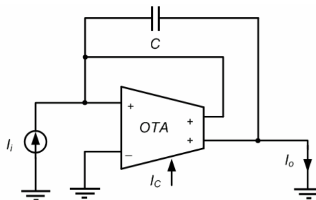
Figure 4.5. All-pass filter circuit in (Liu et al. , 1995)
