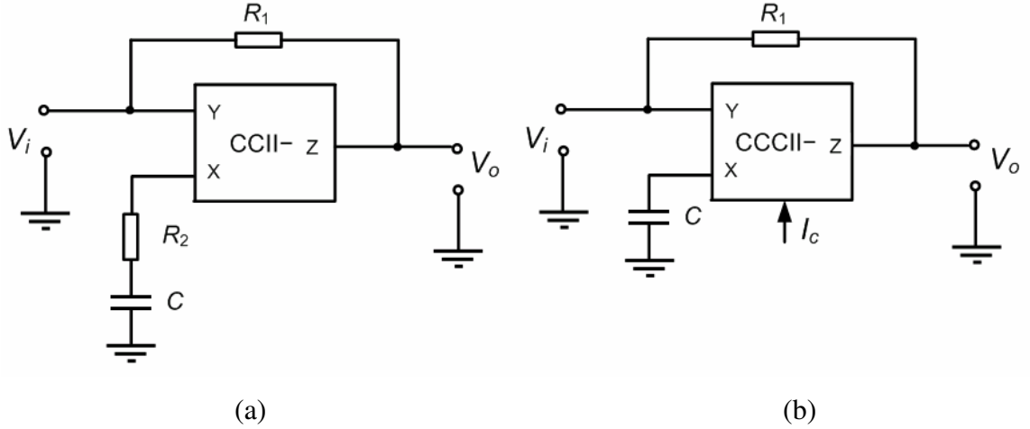
Figure 3.2. (a) All-pass filter with a single CCII– (b) All-pass filter with a single CCCII–
