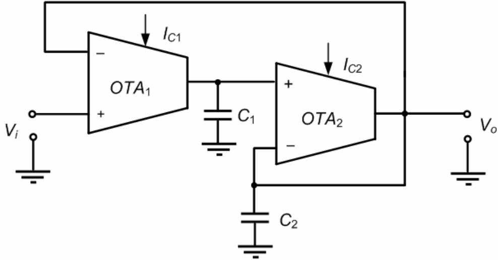
Figure 4.13. The OTA-C low-pass filter (Urbas and Osiowski, 1982)
