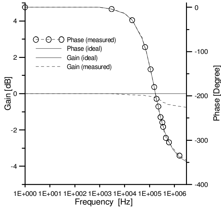
Figure 3.8. The theoretical and measured gain and phase response ( f_0 \approx 159.2\text{kHz} )
