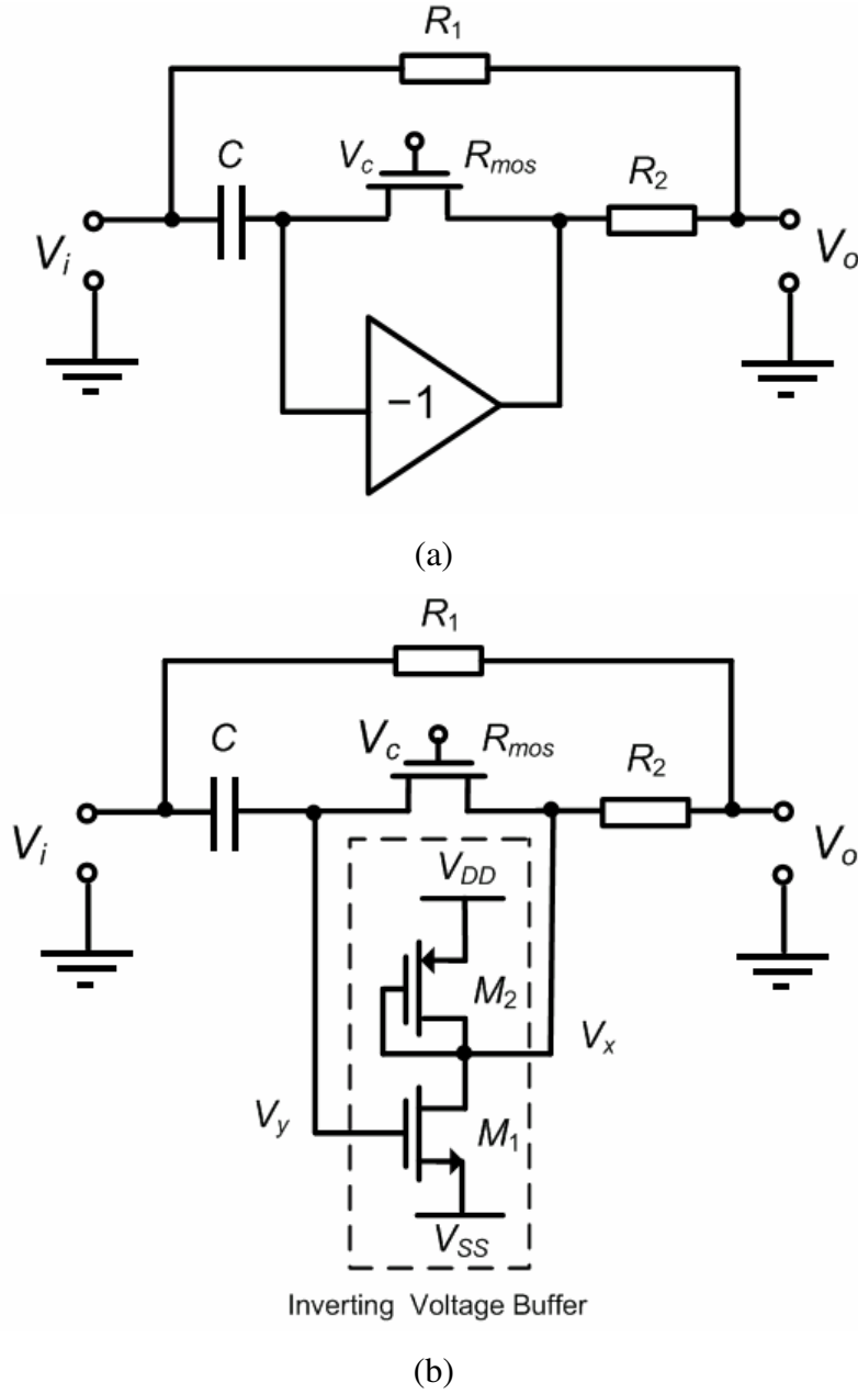
Figure 2.3. (a) The presented MOSFET-C all-pass filter (b) A possible CMOS implementation
