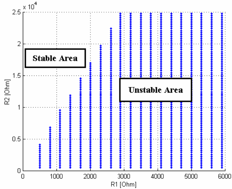
Figure 5.18. Tunability restricted by stability \omega_p s and L_X s are functions of the I_C for the CCCIIIs
