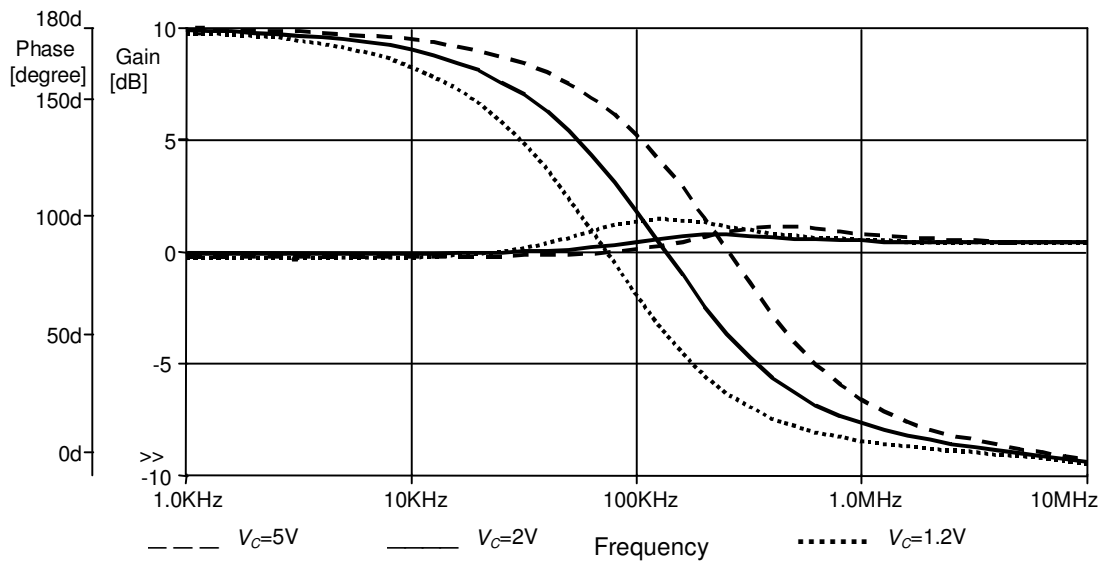
Figure 2.16. Simulated gain and phase responses of the proposed circuit (The pole frequency can be tuned between 68kHz and 235kHz)
