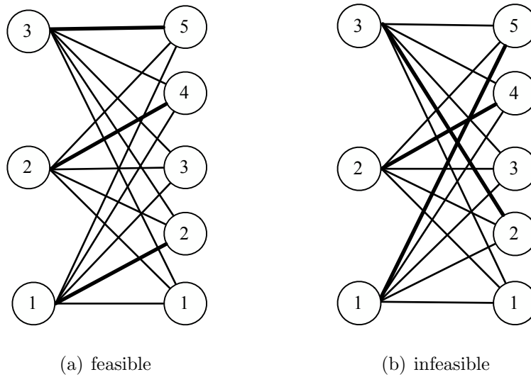
Figure 5.4. Matchings
