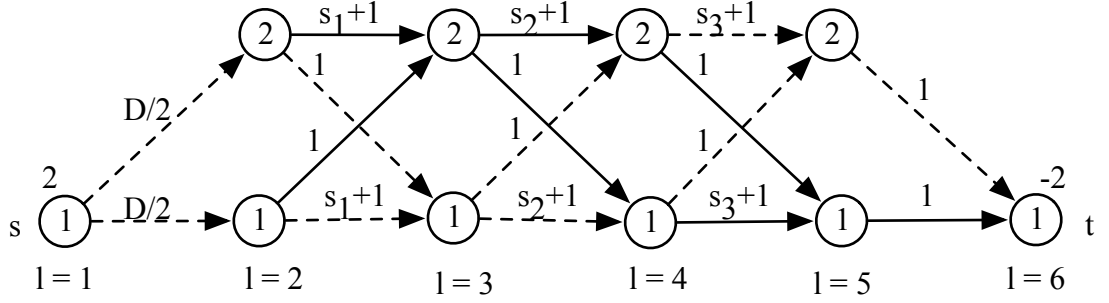
Figure 5.1. Noncrossing paths corresponding to an SPP instance
