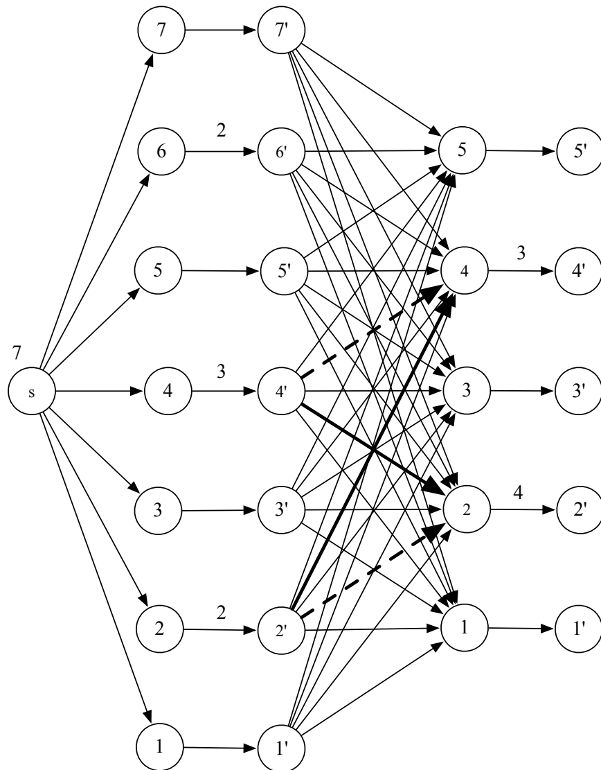
Figure 4.3. The layered network appropriate for a minimum cost network flow formulation of the example given in Figure 4.1 and Figure 4.2
