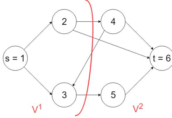
Figure 2.5. An s - t cut.
