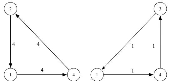
(c) Flow circuits of an equivalent path and circuit flow
