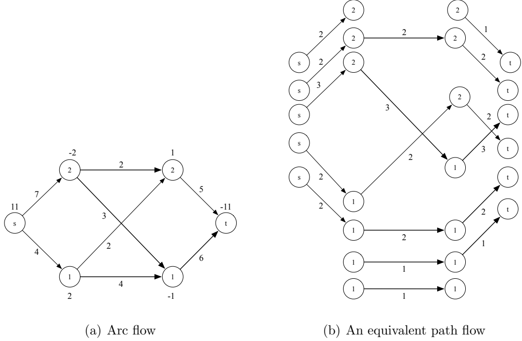
Figure 2.4. Two ways to express a flow in a layered network
