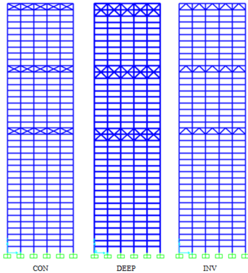
Figure 10.10. Different types of outrigger and belt truss systems on 40-story building.
