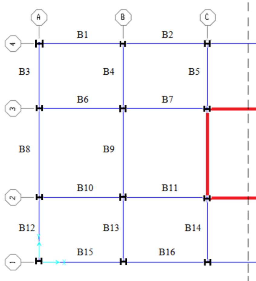
Figure 7.2. Given specific codes of beams.
