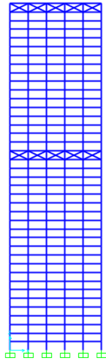
Figure 10.4. Optimum location of two outrigger systems on 40-story building.
