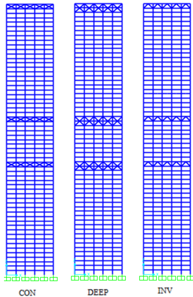
Figure 10.22. Different types of outrigger and belt truss systems on 60-story building.
