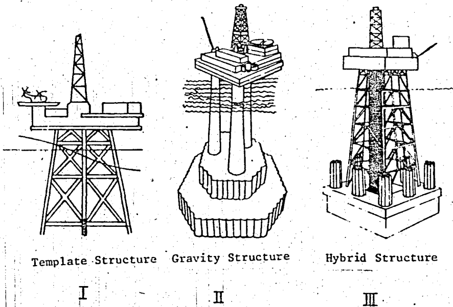
Fig. 1.3.- Offshore Platform Types (after Togrol, 1981)
