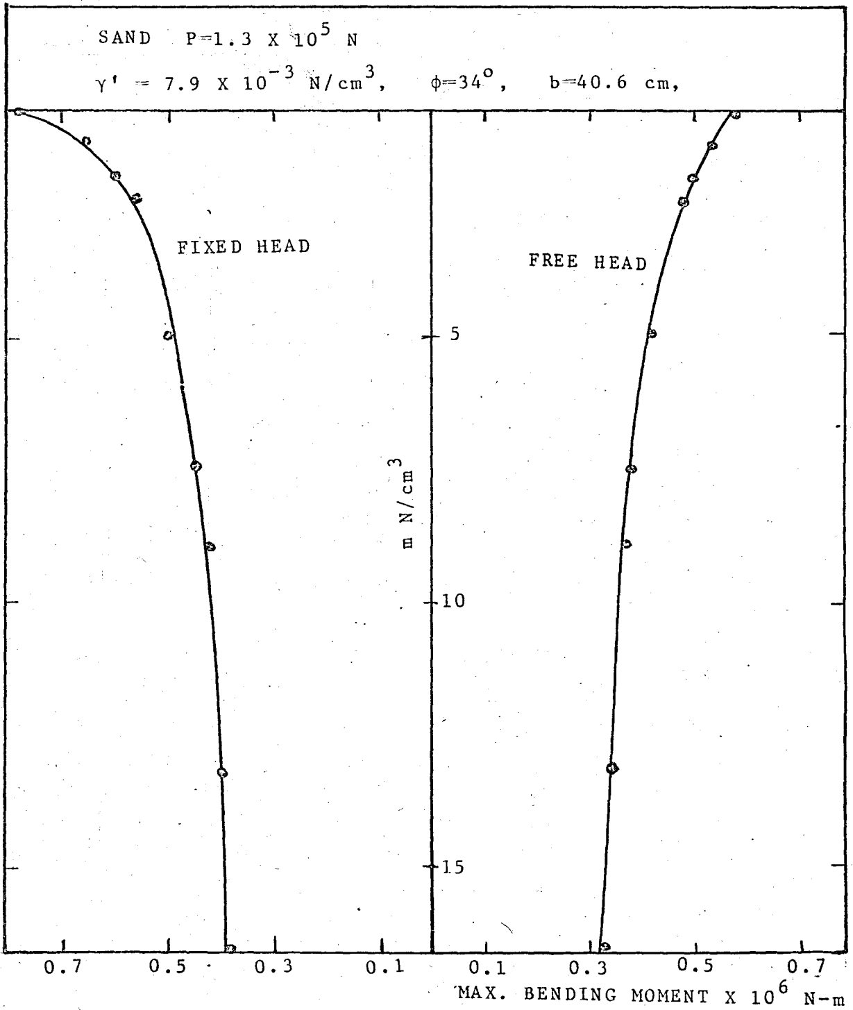
Fig. 6.11.- Maximum Bending Moments vs. Lateral Soil Reaction Coefficient in Dense Sand
