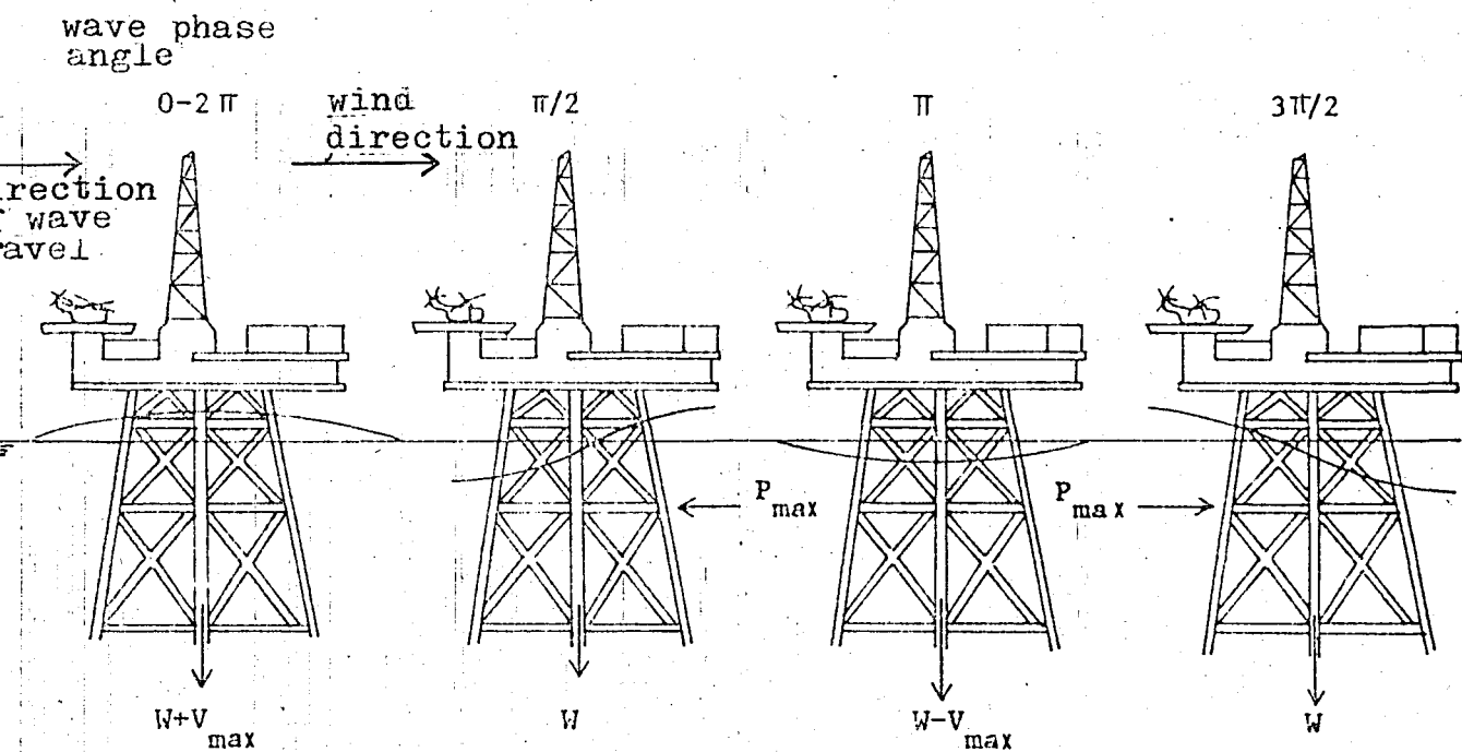
Fig. 2.3.- Principal Forces Acting on a Template Structure (after Saġlamer, 1977)
