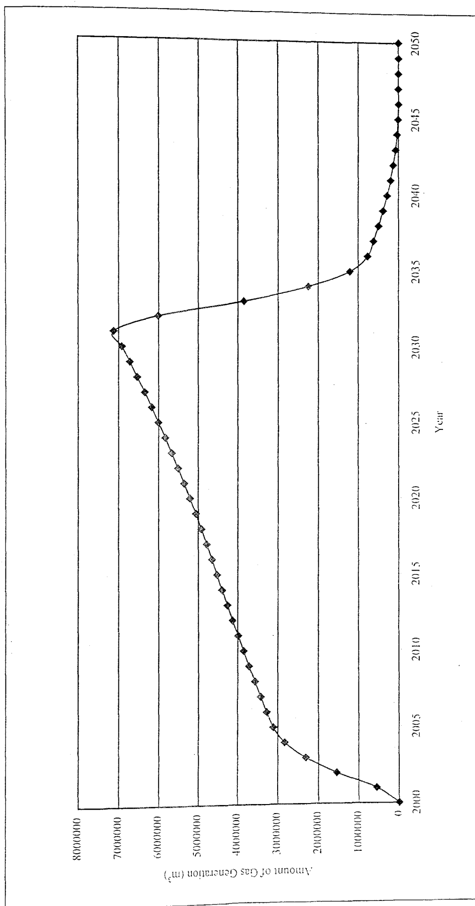
Figure 10.5. Method I - Annual gas generation (m³)
