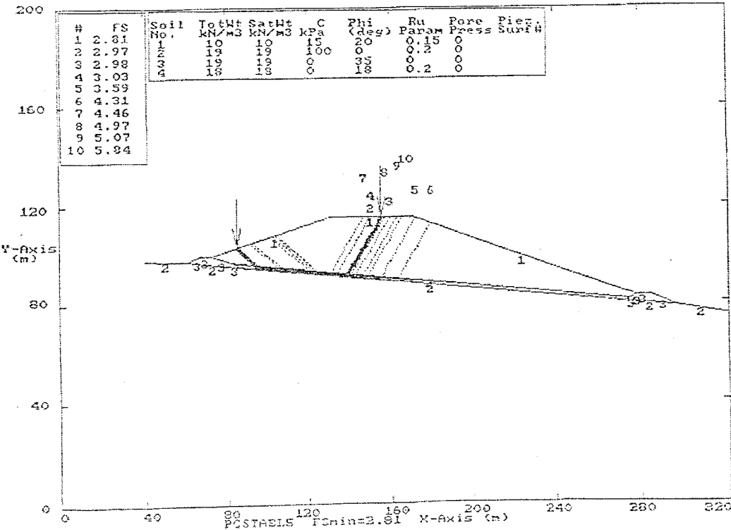
Figure 6.7d. 10 landslide surfaces giving minimum security coefficients in Lot-2 (left berm)
