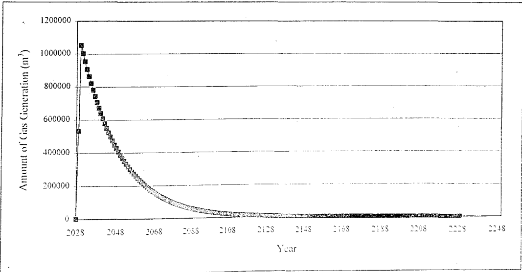
Figure 10.8. Gas generation in Lot-3 (LandGEM model - CAA defaults)
