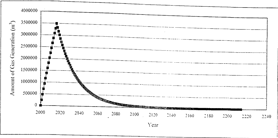
Figure 10.6. Gas generation in Lot-1 (LandGEM model - CAA defaults)
