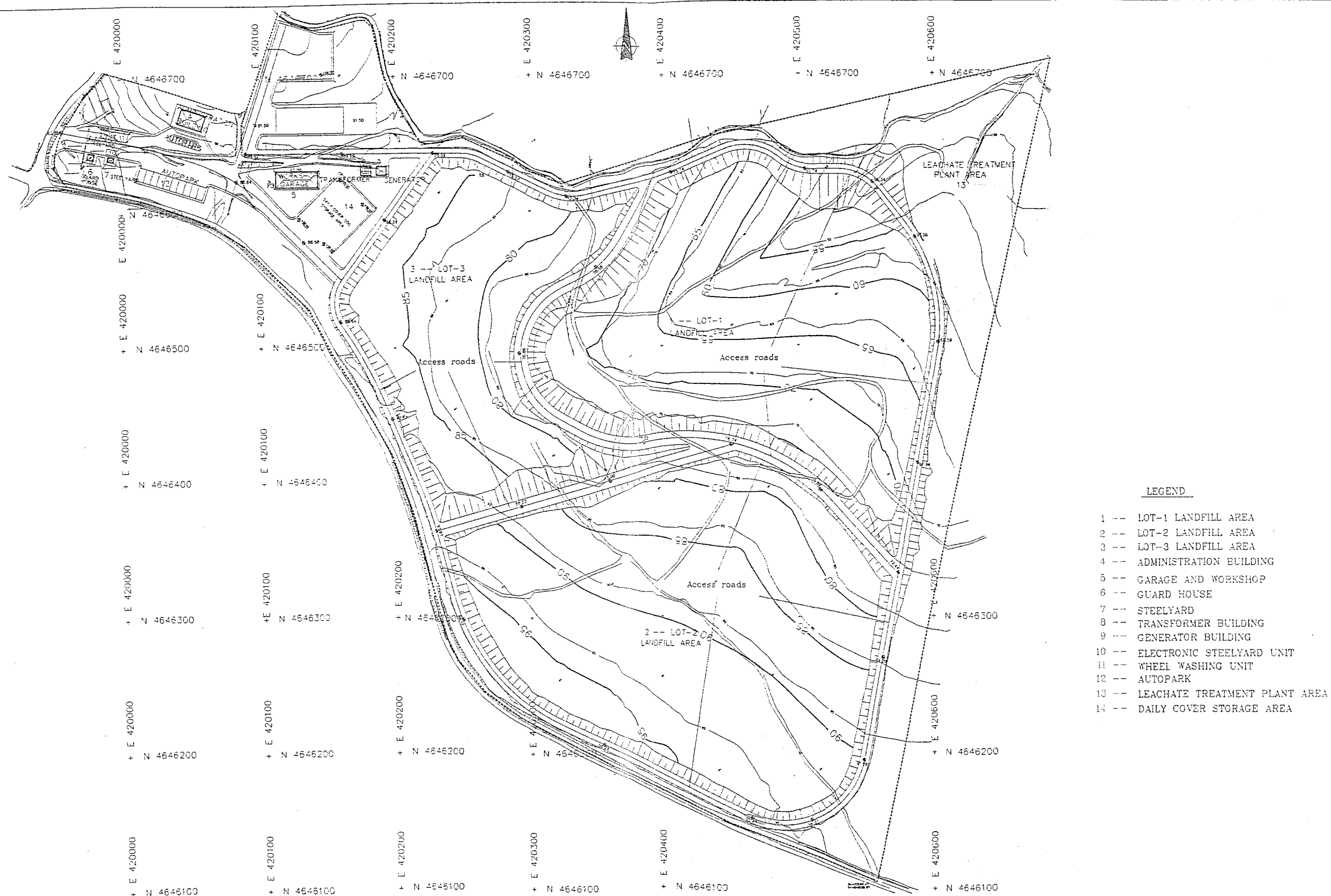
Figure 6.3. The general layout of the lots, access roads, units and leachate treatment plant area
