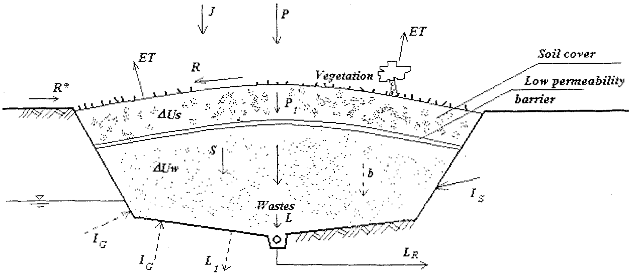
Figure 8.1. Schematic of the general hydrological balance in a completed sanitary landfill with leachate drainage system (Thornthwaite et al., 1955)
