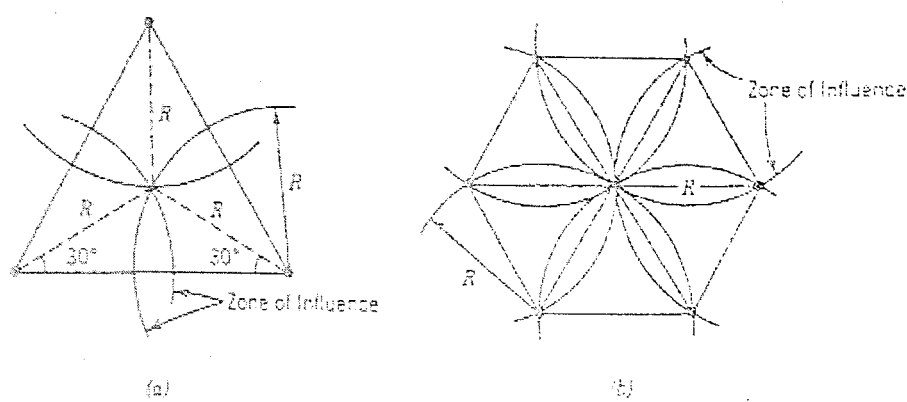
Figure 10.14. Positioning of gas extraction well for complete overlap: (a) triangular array: (b) hexagonal array (Bagchi, 1989)
