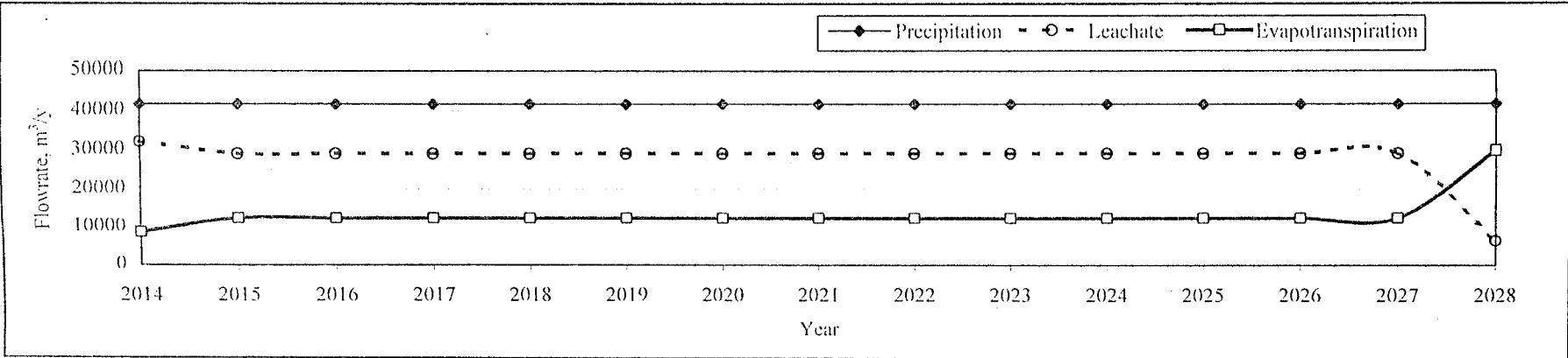
Figure 8.6a. Annual amount of precipitation, leachate and evapotranspiration in Lot-2 (HELP model)
