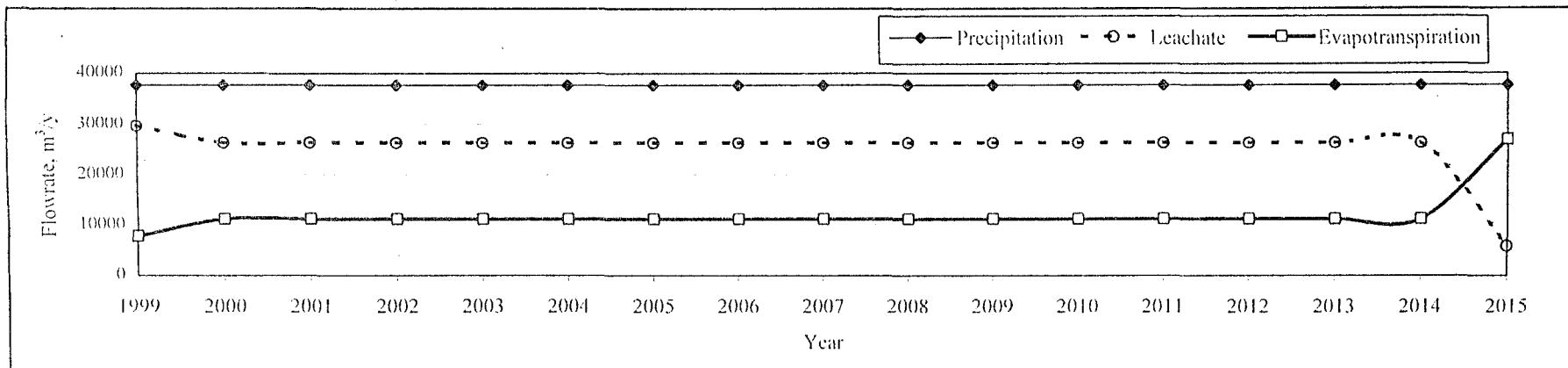
Figure 8.5a. Annual amount of precipitation, leachate and evapotranspiration in Lot-1 (HELP model)
