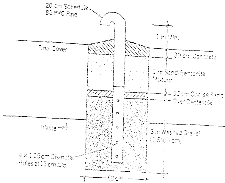
Figure 10.12. Typical detail of an isolated gas vent (Bagchi, 1989)
