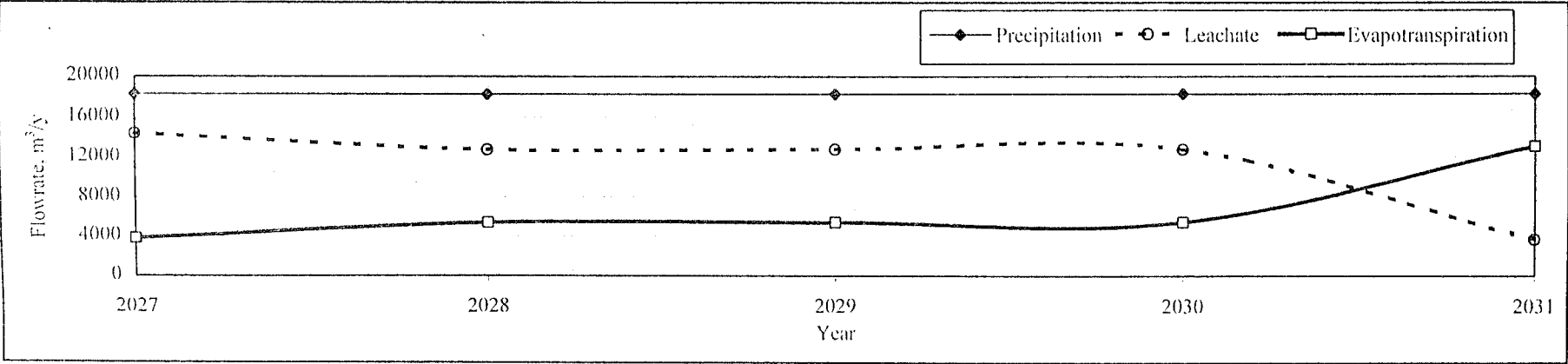
Figure 8.7a. Annual amount of precipitation, leachate and evapotranspiration in Lot-3 (HELP model)
