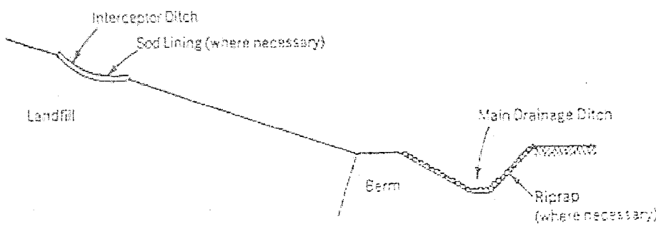
Figure 9.1. Typical arrangements in landfills for surface water routing (Bagchi, 1989)
