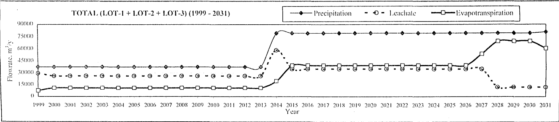
Figure 8.8a Annual total amount of precipitation, leachate and evapotranspiration in Lot-1, Lot-2 and Lot-3 (HELP model)
