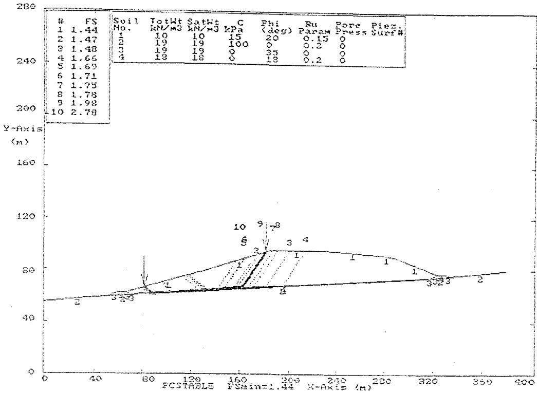
Figure 6.7a. 10 landslide surfaces giving minimum security coefficients in Lot-1 (right berm)
