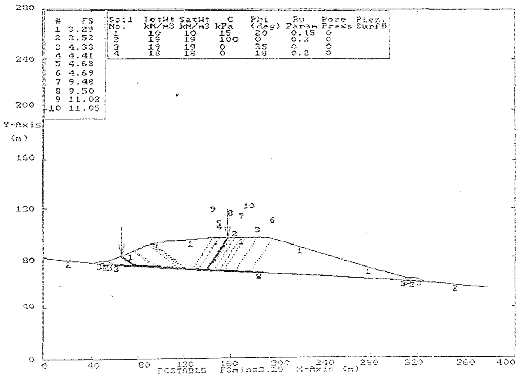
Figure 6.7b. 10 landslide surfaces giving minimum security coefficients in Lot-1 (left berm)
