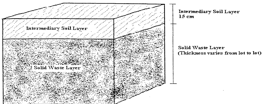
Figure 8.4. Representation of the final solid waste lift introduced into the HELP model system when the related lot is closed to solid waste disposal (Schroeder et al., 1997)
