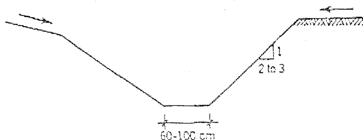
Figure 9.2. Typical cross section of drainage ditch (Bagchi, 1989)
