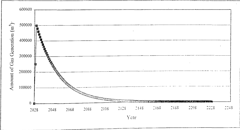
Figure 10.11. Gas generation in Lot-3 (LandGEM Model - AP42 defaults)
