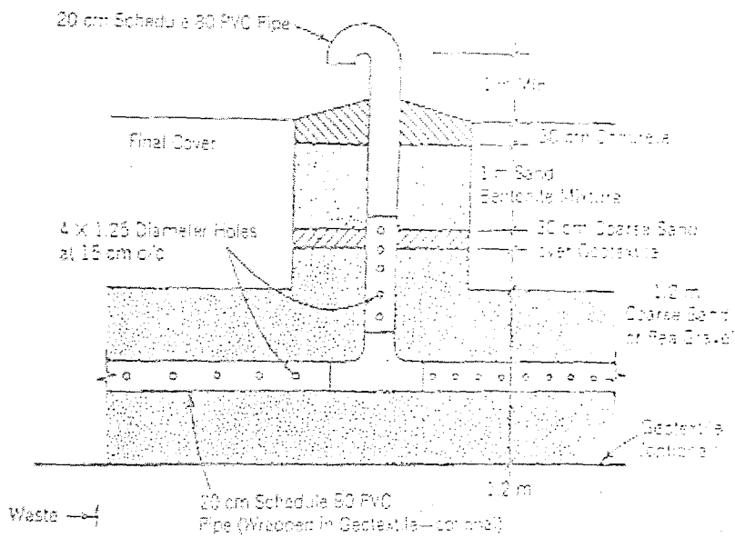
Figure 10.13. Typical detail of a passive gas venting system with a header pipe (Bagchi, 1989)
