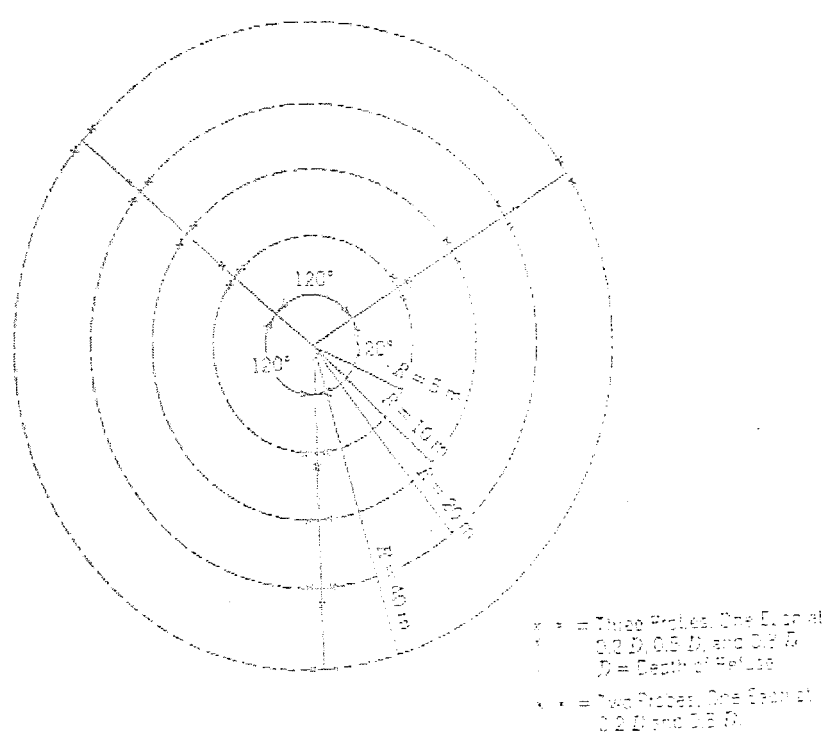
Figure 10.15. Gas extraction well and probe cluster configuration for zone of influence determination (Bagchi, 1989)
