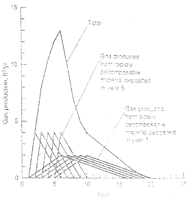
Figure 10.2. Graphical representation of gas production over a five-year period from the rapidly and slowly decomposable organic materials placed in a landfill (Tchobanoglous et al., 1993)
