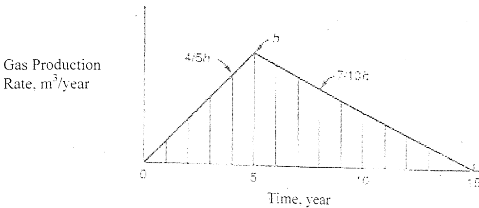
Figure 10.4. The gas production over the 15-year period (Tchobanoglous et al., 1993)
