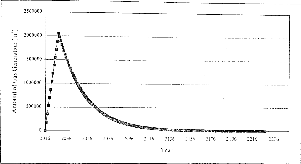
Figure 10.10. Gas generation in Lot-2 (LandGEM Model - AP42 defaults)
