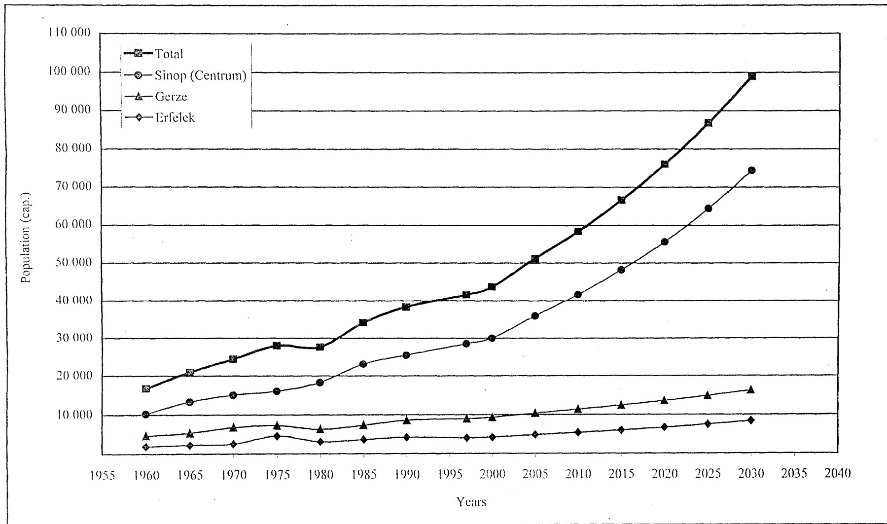
Figure 3.2. The future population projection according to geometric increase
