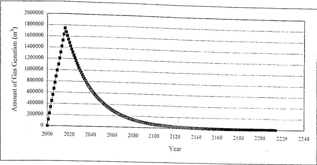
Figure 10.9. Gas generation in Lot-1 (LandGEM Model - AP42 defaults)
