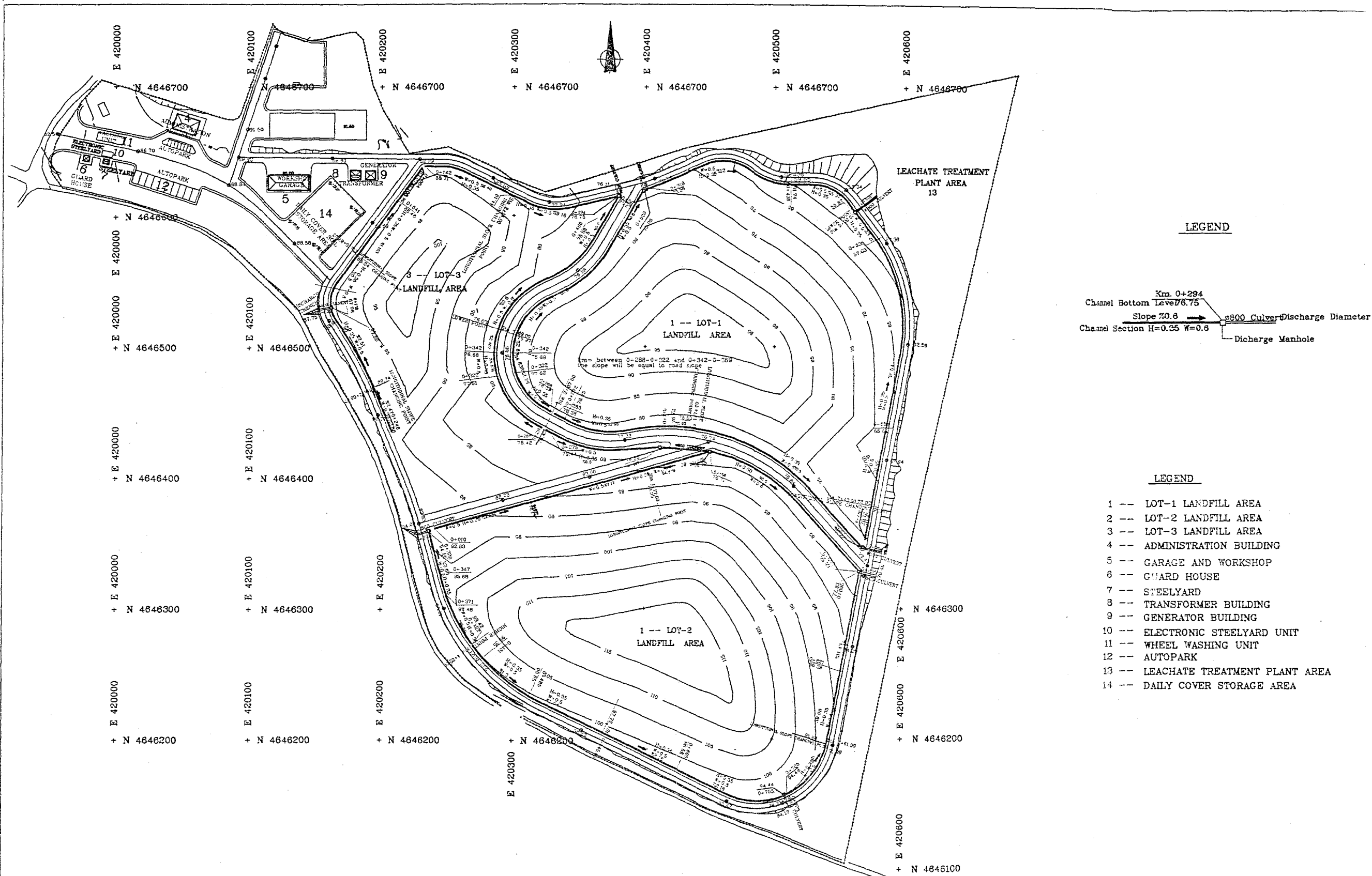
Figure 9.4. General view of surface water drainage system
